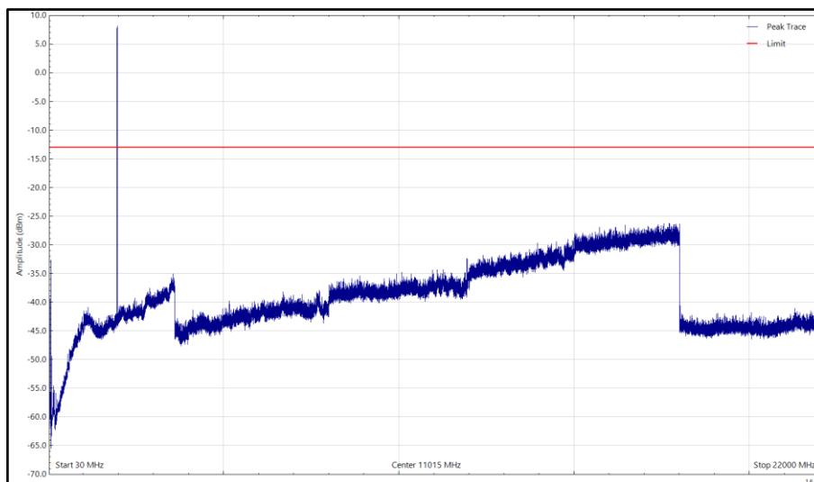
Mid - NR&NB-IoT - B2, 1960MHz, 30 MHz to 22 GHz, Vertical (Peak)
