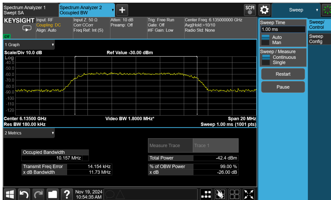
Plot 1: AWGN Signal BW Details
