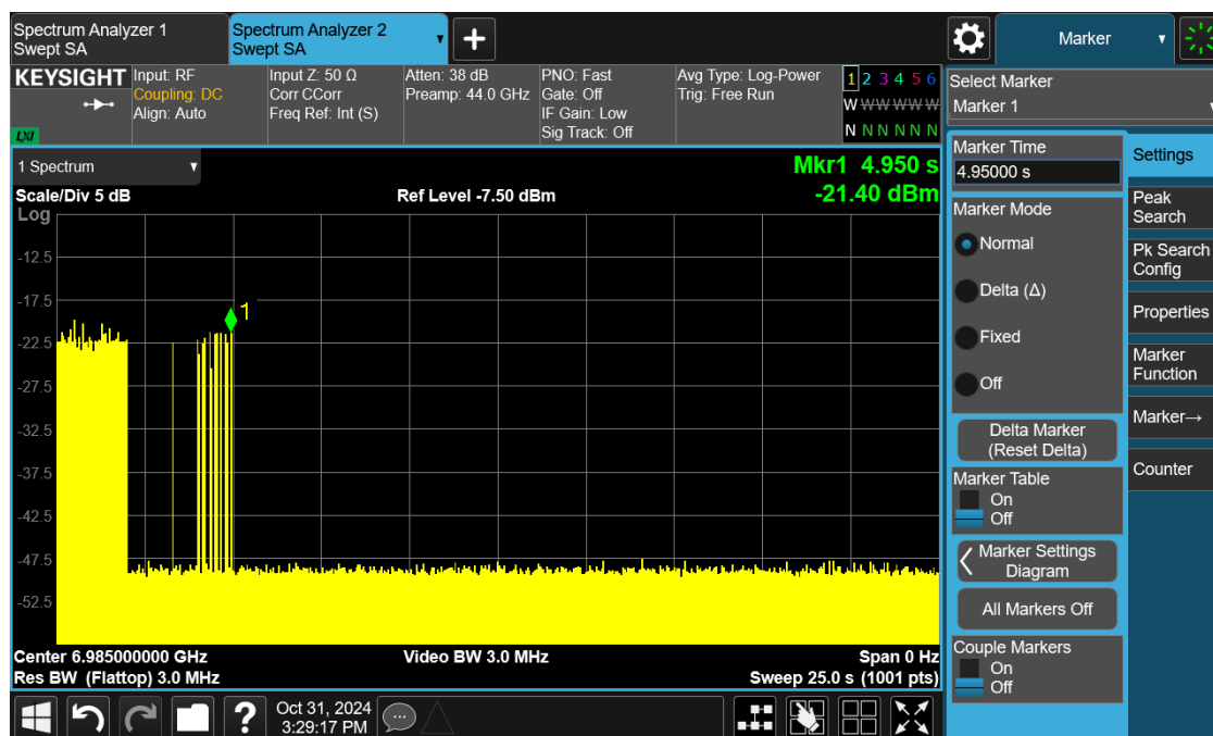
Plot 5: AWGN Signal Detection 160MHz
