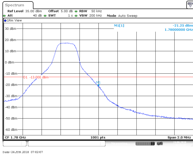
BAND 66_5MHz_16QAM_132647_25RB#0
