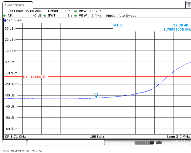
BAND 66_20MHz_16QAM_132572_1RB#0
