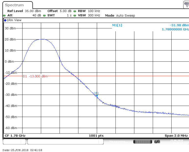
BAND 66_10MHz_64QAM_132622_50RB#0
