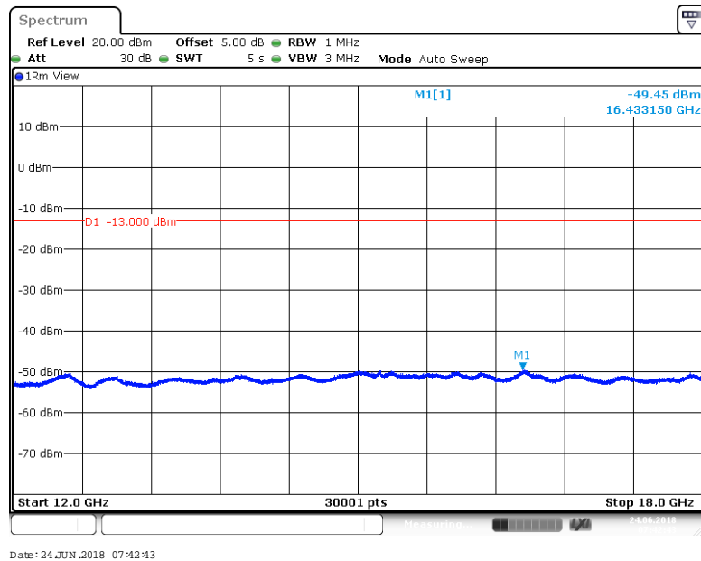
BAND 66_20MHz_64QAM_132072_1RB#0
