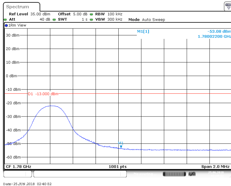
BAND 66_10MHz_64QAM_132622_1RB#49
