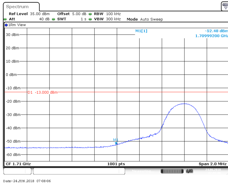
BAND 66_10MHz_16QAM_132022_50RB#0
