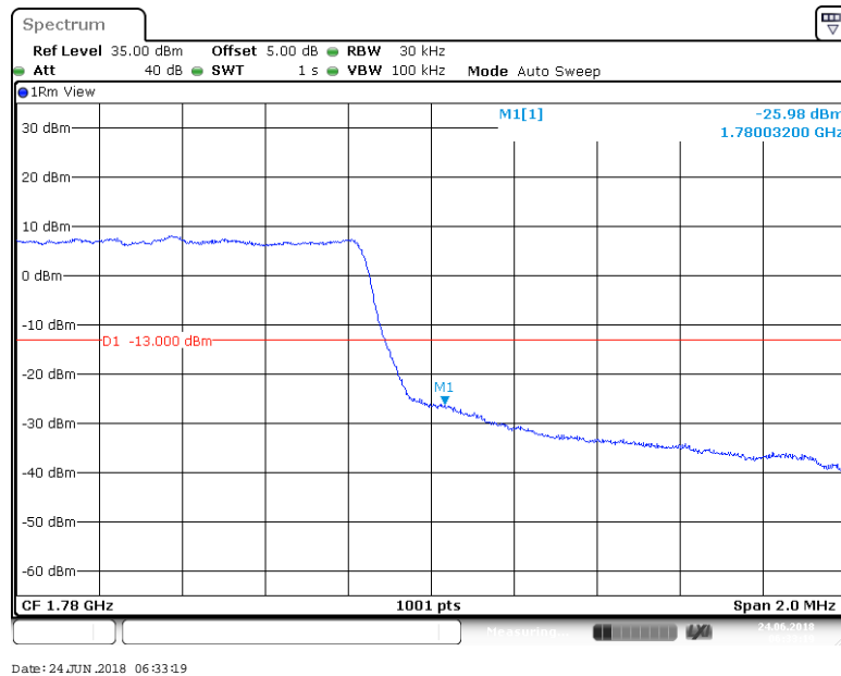
BAND 66_1.4MHz_64QAM_131979_1RB#0
