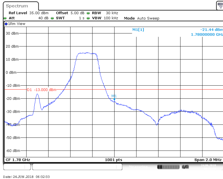
BAND 66_1.4MHz_16QAM_132665_6RB#0
