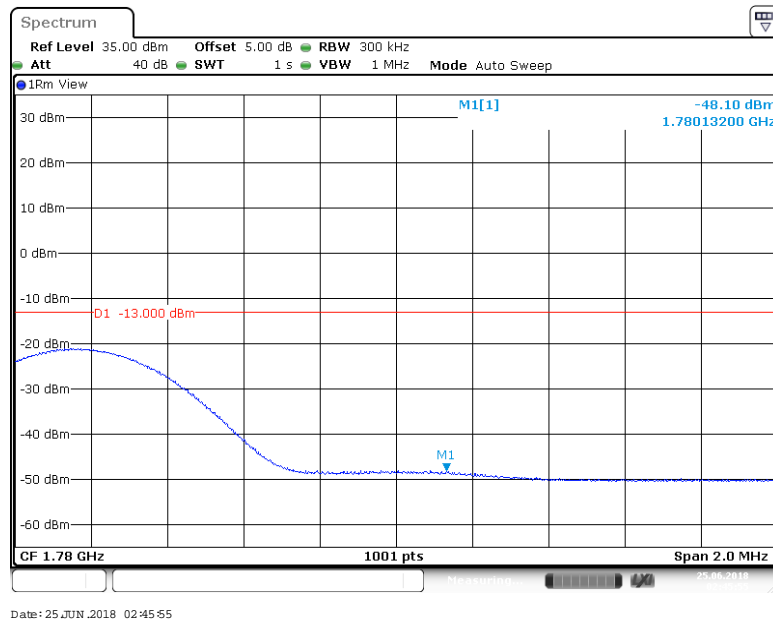
BAND 66_15MHz_64QAM_132597_1RB#74
