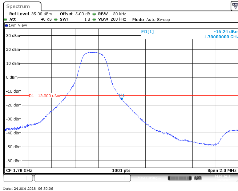
BAND 66_3MHz_QPSK_132657_15RB#0
