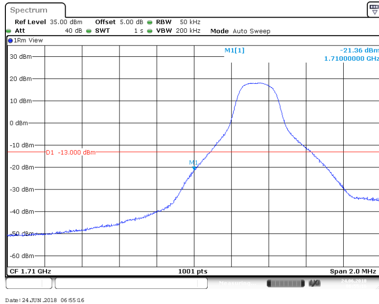
BAND 66_5MHz_QPSK_131997_1RB#24
