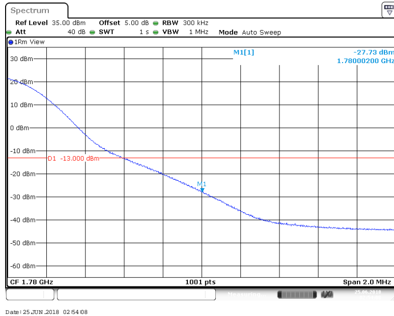
BAND 66_20MHz_64QAM_132572_100RB#0
