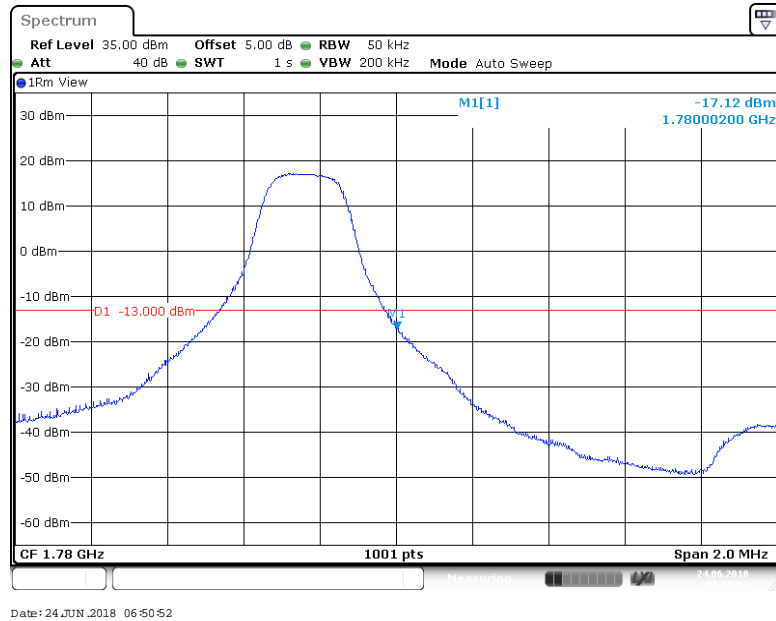
BAND 66_3MHz_16QAM_132657_15RB#0
