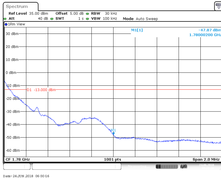
BAND 66_1.4MHz_QPSK_132665_1RB#5
