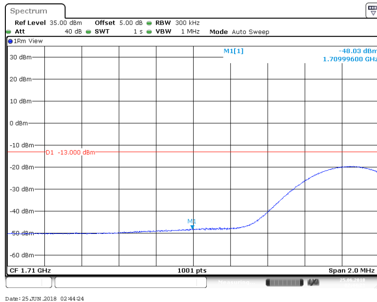
BAND 66_15MHz_64QAM_132047_75RB#0
