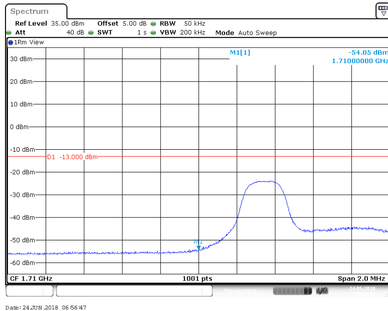
BAND 66_5MHz_QPSK_131997_25RB#0
