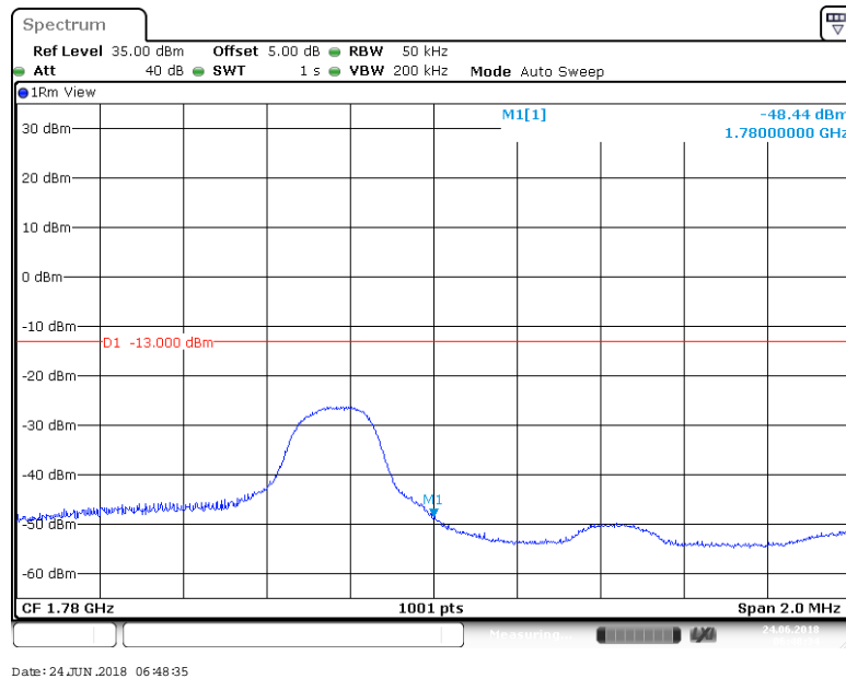
BAND 66_3MHz_QPSK_132657_1RB#14
