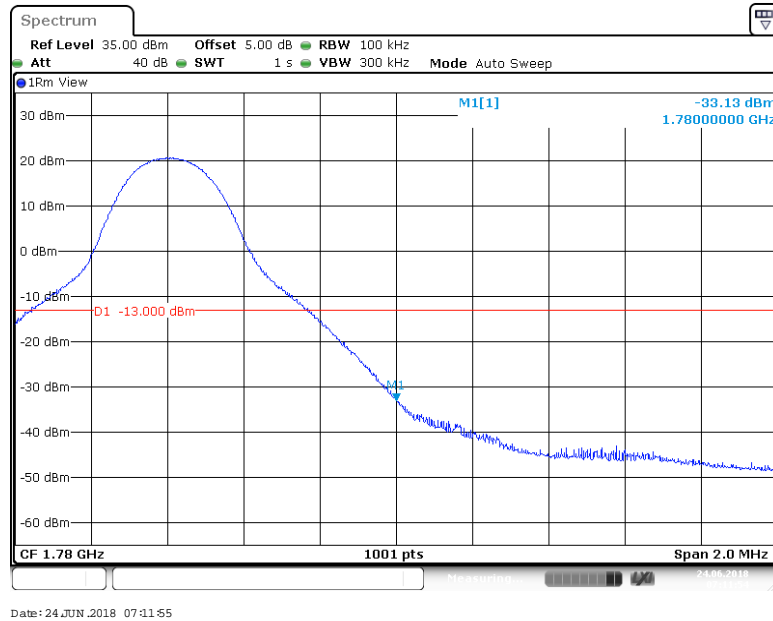
BAND 66_10MHz_QPSK_132622_50RB#0
