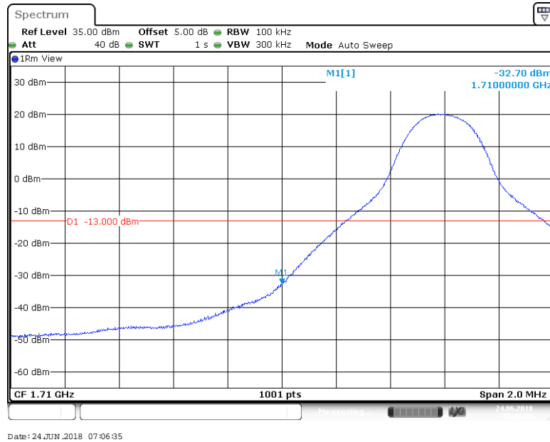
BAND 66_10MHz_16QAM_132022_1RB#49
