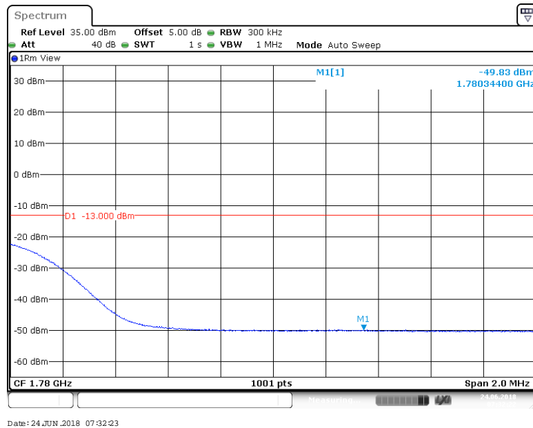
BAND 66_20MHz_16QAM_132572_1RB#99
