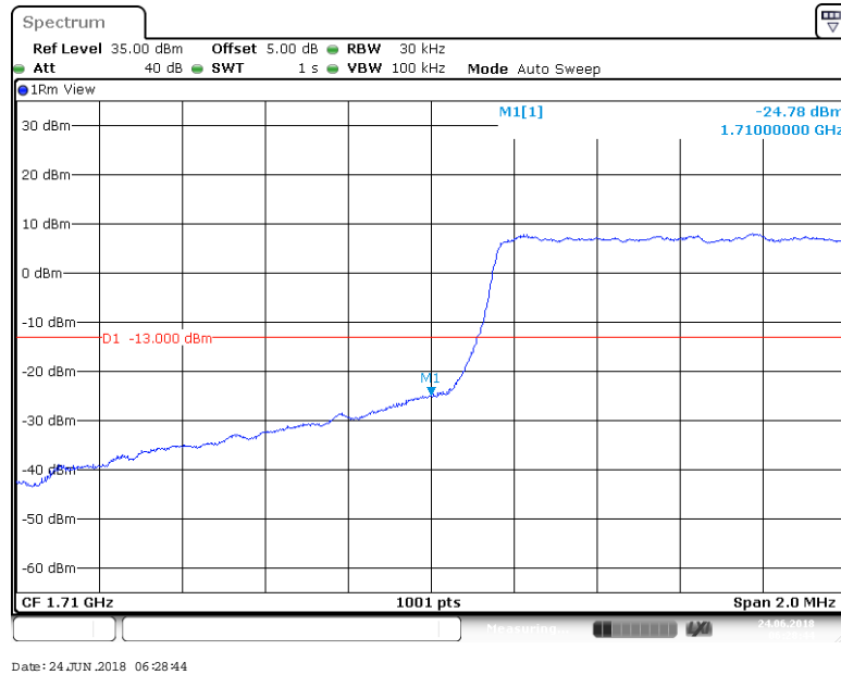
BAND 66_1.4MHz_QPSK_132665_1RB#0
