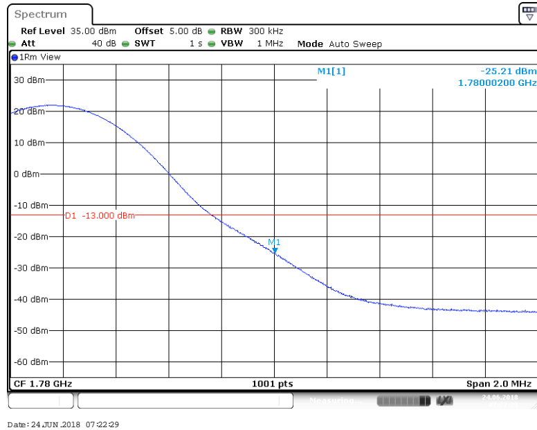
BAND 66_15MHz_QPSK_132597_75RB#0
