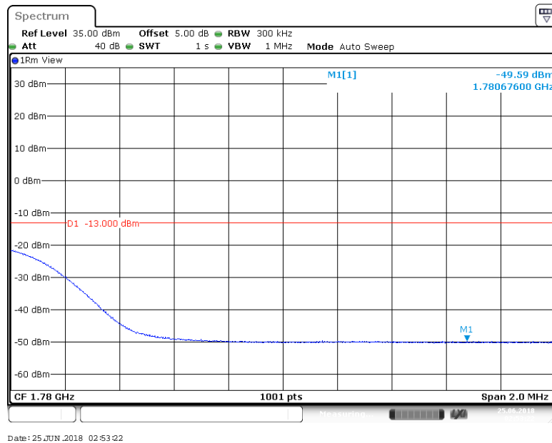
BAND 66_20MHz_64QAM_132572_1RB#99
