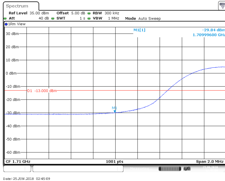
BAND 66_15MHz_64QAM_132597_1RB#0
