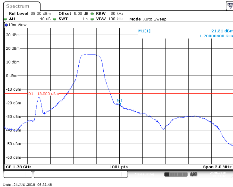
BAND 66_1.4MHz_QPSK_132665_6RB#0
