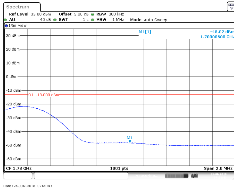
BAND 66_15MHz_16QAM_132597_1RB#74
