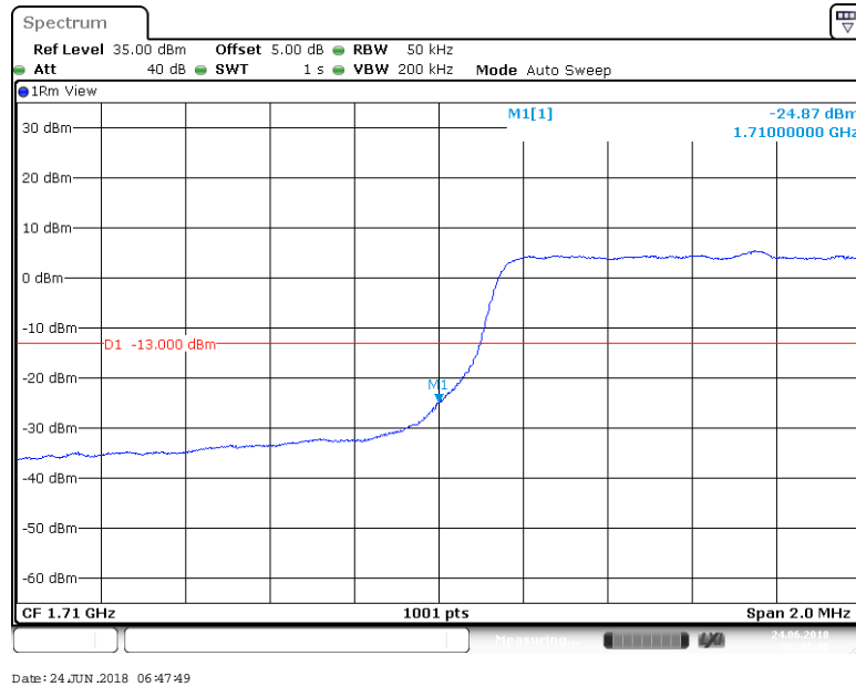
BAND 66_3MHz_16QAM_132657_1RB#0
