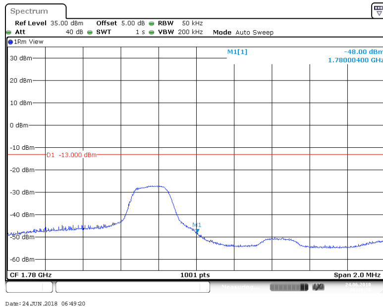
BAND 66_3MHz_16QAM_132657_1RB#14
