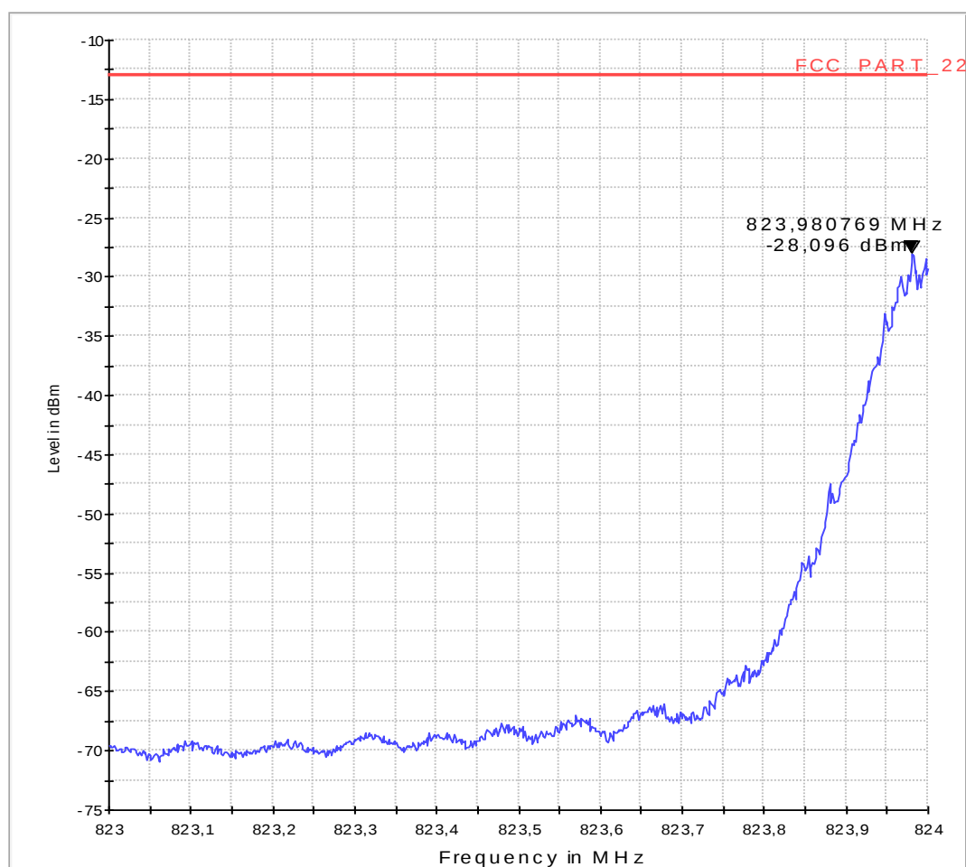
Sweep_3b_Band_Edge_Channel_128_AV
