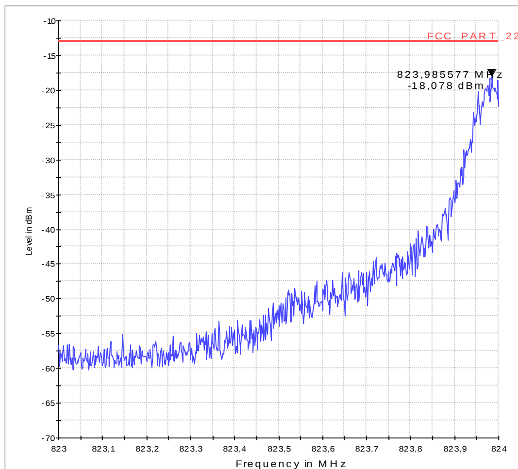
Sweep_3a_Band_Edge_Channel_128_PK
