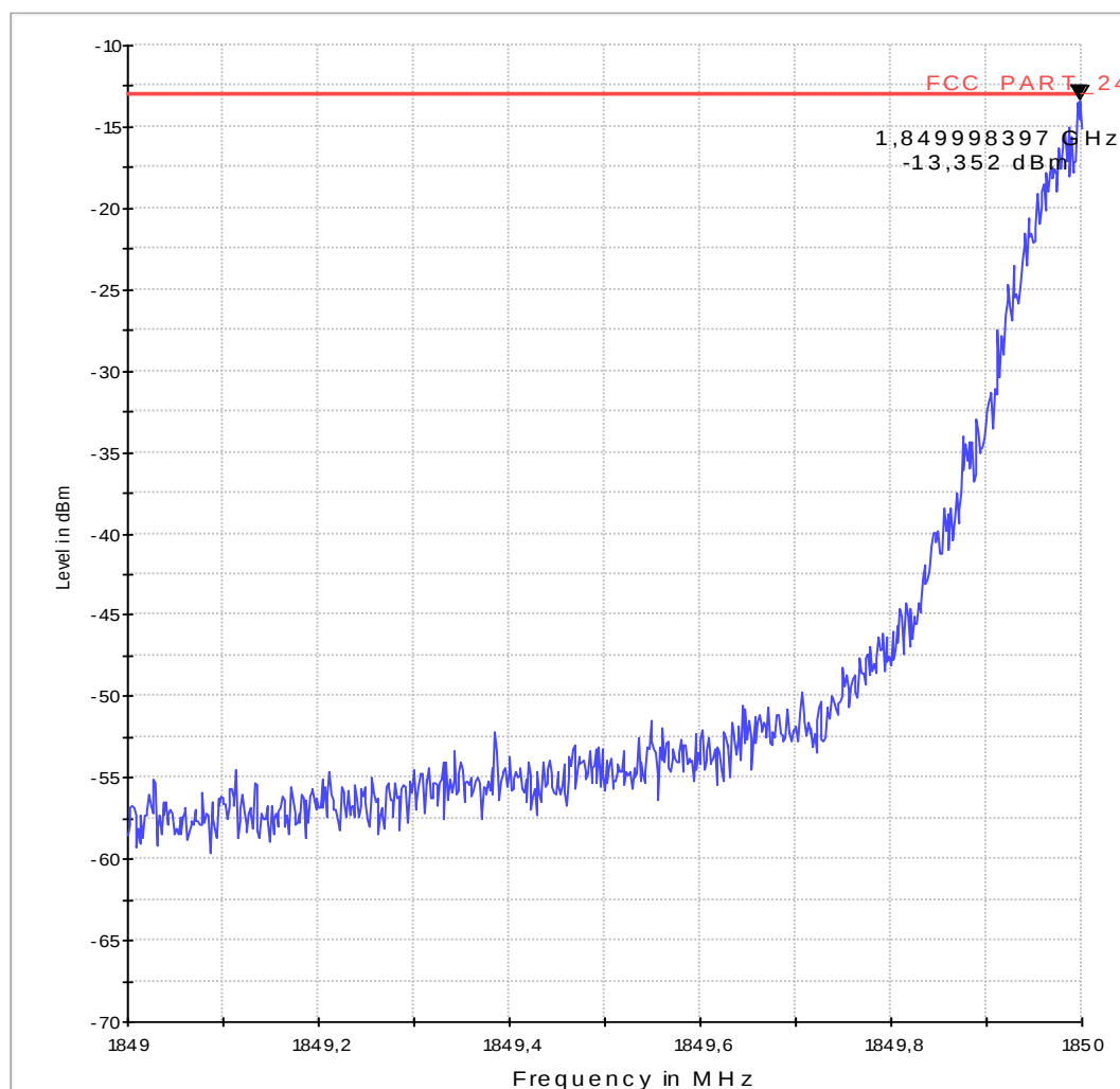
Sweep_3a_Band_Edge_Channel_512_PK
