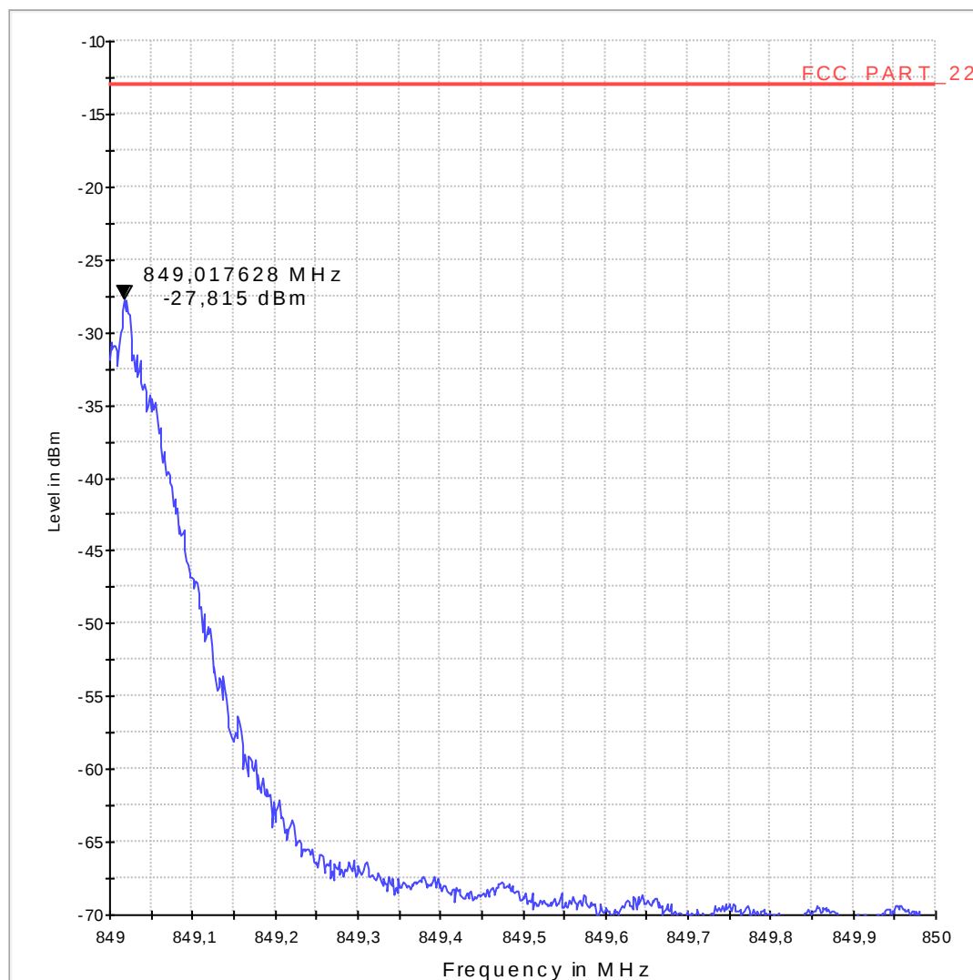
Sweep_4b_Band_Edge_Channel_251_AV
