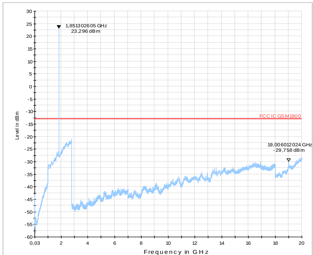
Diagram 8.08_RSE_EDGE
