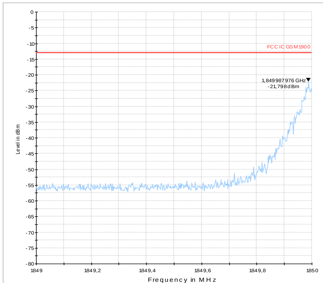
030405_FCC_Part24_GSM1900_TX_low_channel_band_edge
