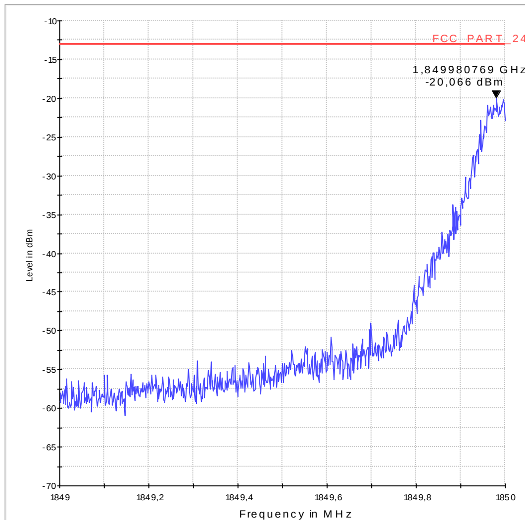
Sweep_3a_Band_Edge_Channel_512_PK
