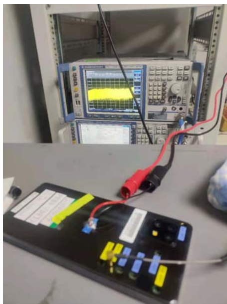
'RF Conducted Test setup (GSM/WCDMA/LTE)
