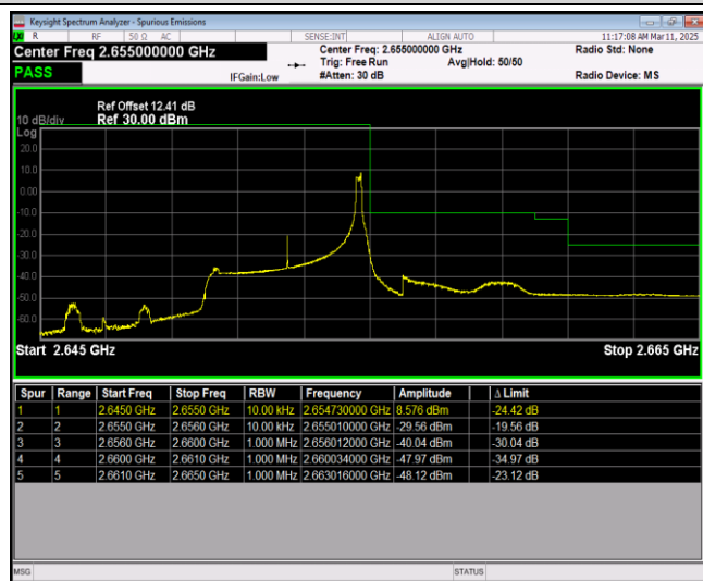
Band41-5MHz-16QAM-40065-1RB#0
