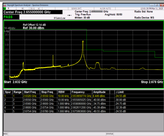
Band41-20MHz-64QAM-40140-1RB#0
