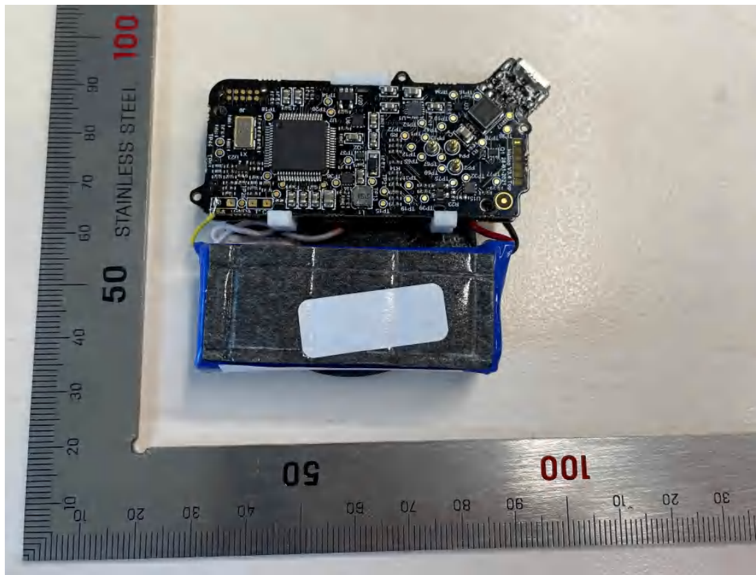
Figure 4 Internal electronics unit view with cover removed -2
