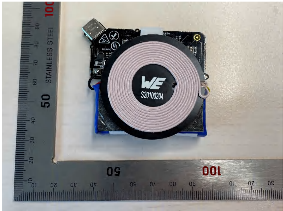
Figure 3 Internal electronics unit view with cover removed -1
