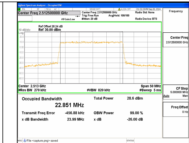
n7 25M DFT-s-OFDM 64QAM Outer_Full Low
