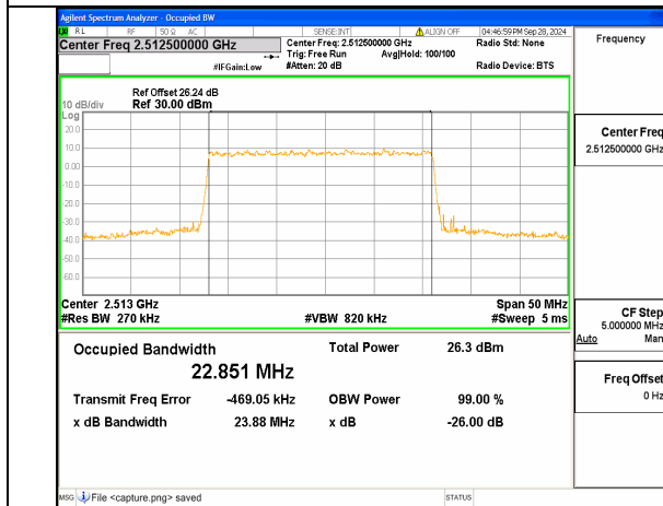
n7 25M DFT-s-OFDM 256QAM Outer_Full Low
