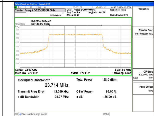
n7 25M CP-OFDM QPSK Outer_Full Low
