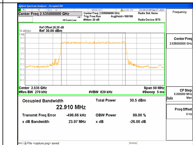
n7 25M DFT-s-OFDM QPSK Outer_Full Mid
