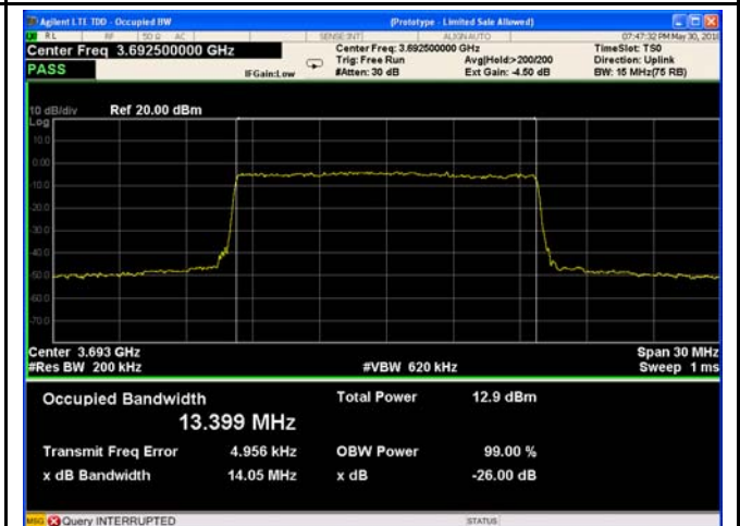
15MHz - High CH 16QAM
