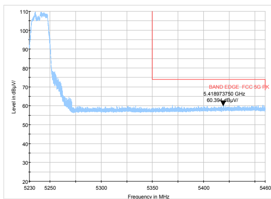
802.11a-Channel 48: Average
