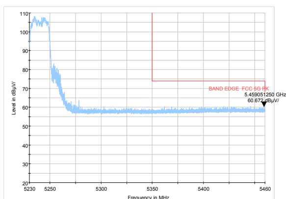
802.11n HT20-Channel 48: Peak
