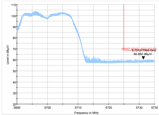
802.11a-Channel 140: Peak
