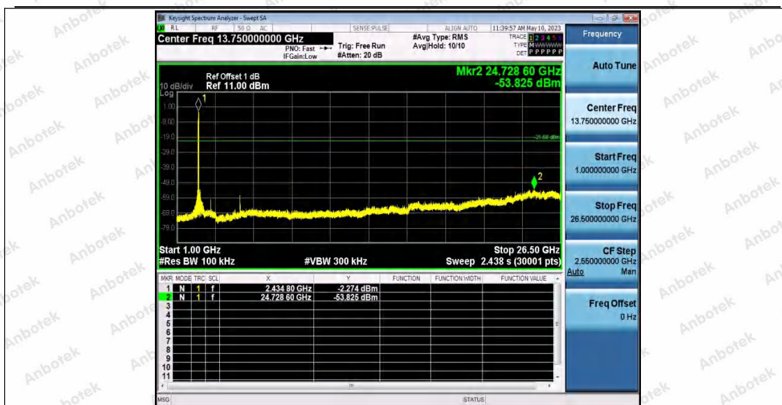
11N40SISO_Ant1_2452_0~Reference
