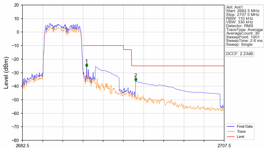
Band41_5MHz_16QAM_HCH_2687.5MHz_RB_25_0_NTNV
