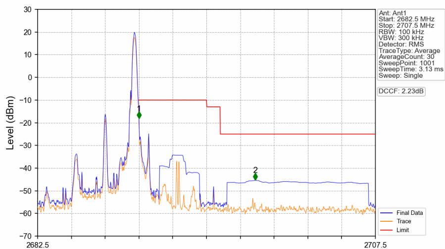
Band41_5MHz_16QAM_HCH_2687.5MHz_RB_1_24_NTNV
