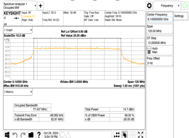
802.11ax_80MHz_ChainB_6145MHz
