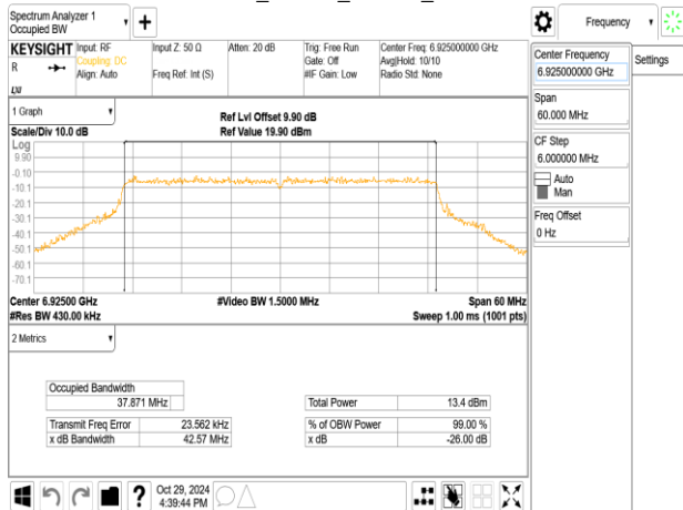
802.11ax_40MHz_ChainA_6925MHz_RU242_61
