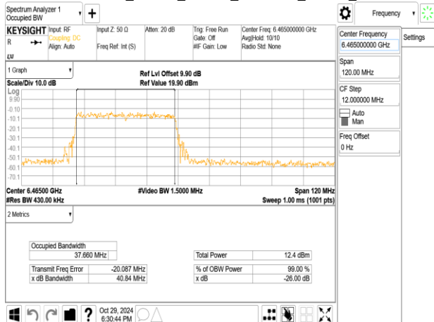
802.11ax_80MHz_ChainA_6465MHz_RU484_65
