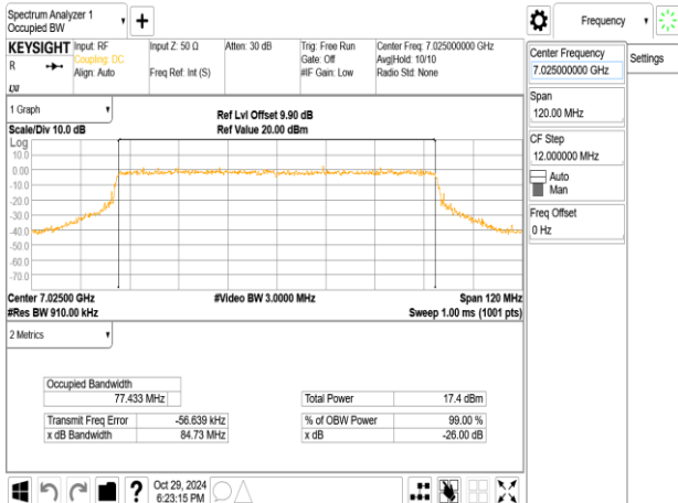
802.11ax_80MHz_ChainA_7025MHz_RU484_66
