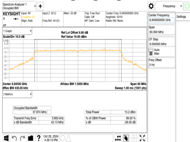
802.11ax_40MHz_ChainB_6845MHz_RU242_62
