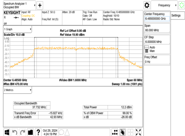
802.11ax_40MHz_ChainA_6485MHz_RU242_62
