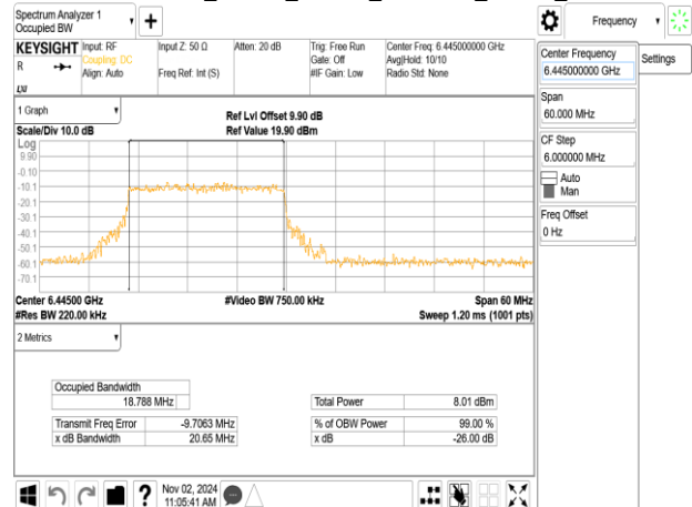
802.11ax_40MHz_ChainB_6445MHz_RU242_61
