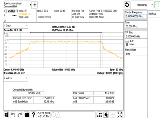
802.11ax_40MHz_ChainB_6445MHz_RU242_61
