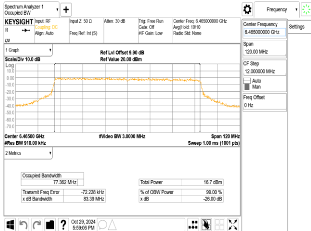
802.11ax_80MHz_ChainA_6465MHz_RU484_65
