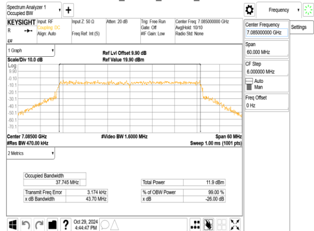
802.11ax_40MHz_ChainA_7085MHz_RU242_62
