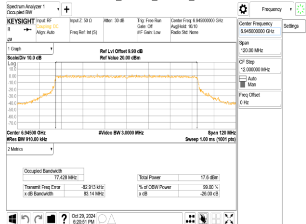
802.11ax_80MHz_ChainA_6945MHz
