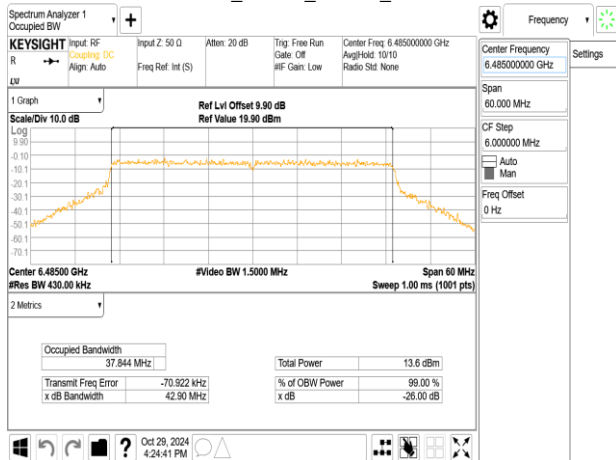
802.11ax_40MHz_ChainB_6485MHz_RU242_62
