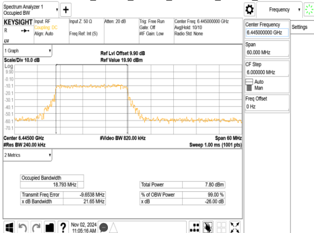
802.11ax_40MHz_ChainA_6445MHz_RU242_61
