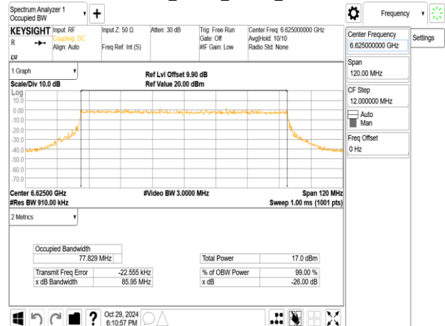
802.11ax_80MHz_ChainA_6625MHz
