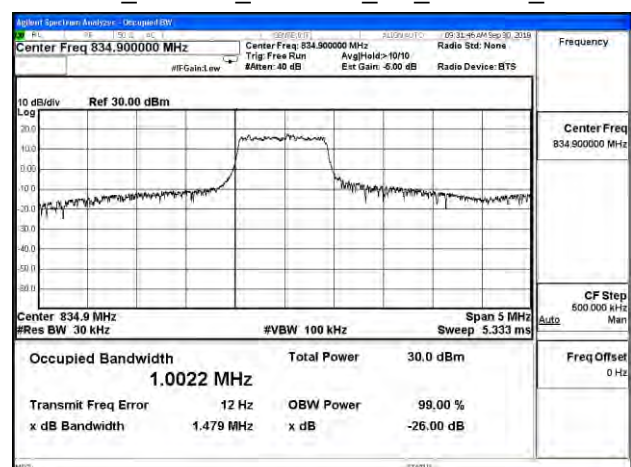
Cat M1_Band 26_CH26915_5M_16-QAM_5RB1
