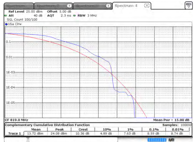
Cat M1_Band 26_CH26740_5M_QPSK_1RB0
