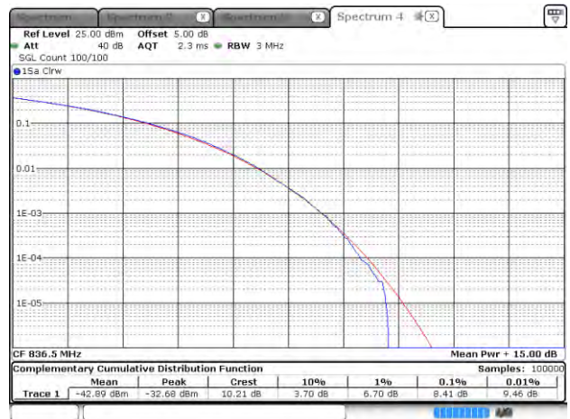
Cat M1_Band 5_CH20525_10M_QPSK_1RB0
