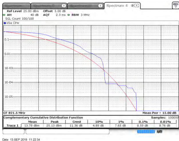
Cat M1_Band 26_CH26765_5M_QPSK_1RB0
