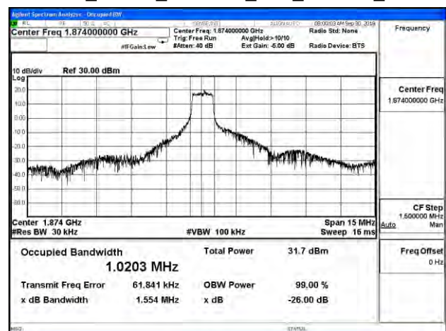
Cat M1_Band 2_CH18900_15M_16-QAM_5RB1
