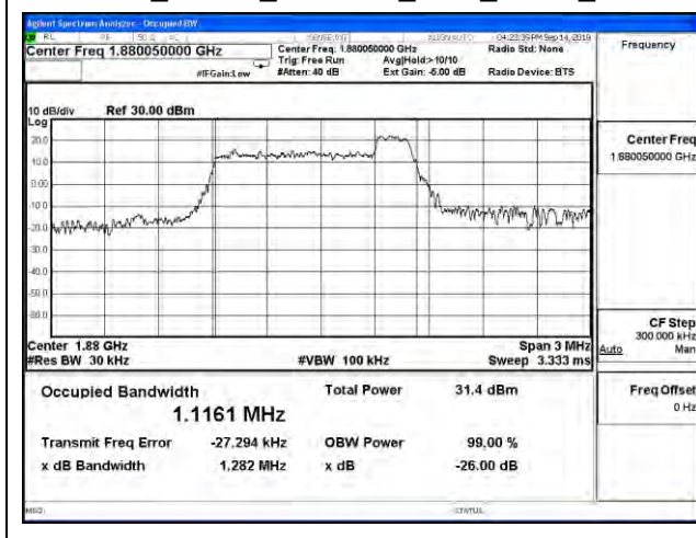
Cat M1_Band 2_CH18900_1.4M_QPSK_6RB0
