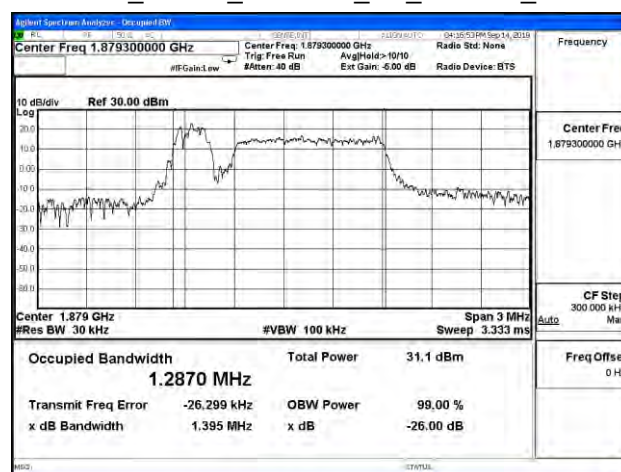
Cat M1_Band 2_CH18900_3M_16-QAM_5RB1
