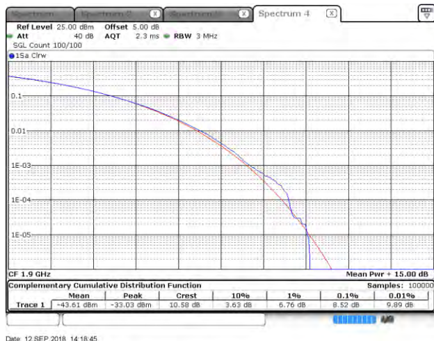
Cat M1_Band 2_CH19100_20M_QPSK_1RB0
