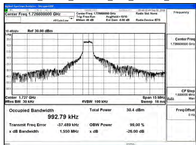
Cat M1_Band 4_CH20175_15M_16-QAM_5RB1
