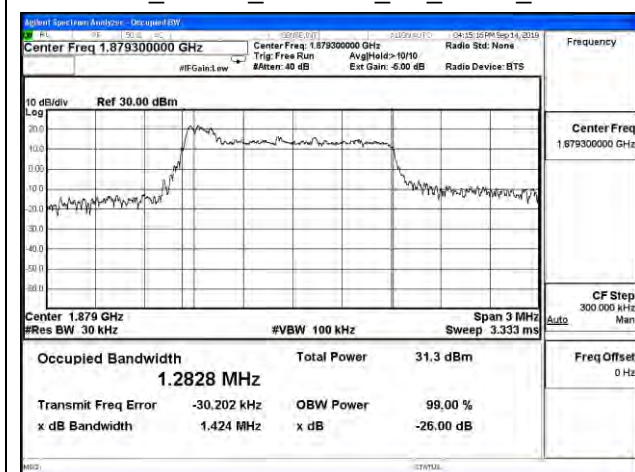
Cat M1_Band 2_CH18900_3M_QPSK_6RB0
