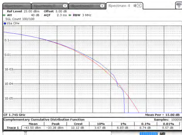
Cat M1_Band 4_CH20300_20M_QPSK_1RB0
