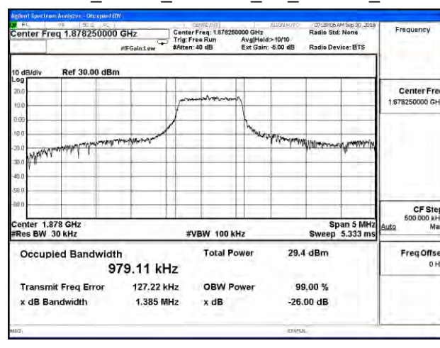
Cat M1_Band 2_CH18900_5M_16-QAM_5RB1
