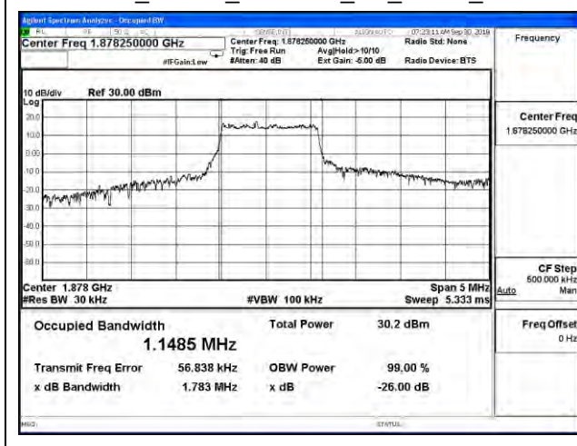
Cat M1_Band 2_CH18900_5M_QPSK_6RB0
