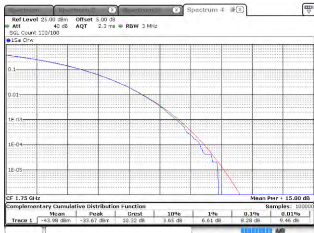
Cat M1_Band 4_CH20350_10M_QPSK_1RB0
