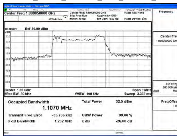
Cat M1_Band 2_CH18900_1.4M_16-QAM_5RB1
