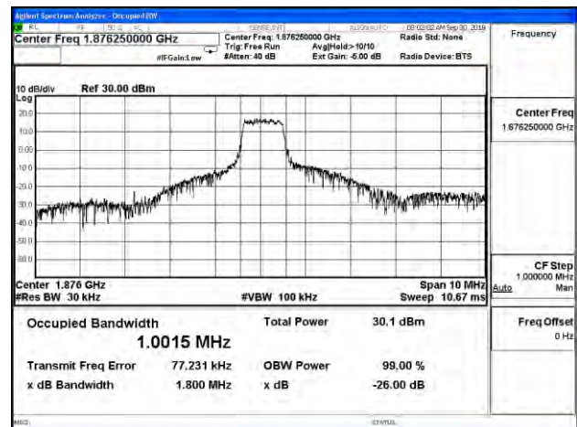
Cat M1_Band 2_CH18900_10M_16-QAM_5RB1
