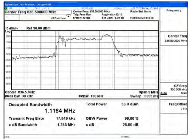
Cat M1_Band 26_CH26915_1.4M_16-QAM_5RB1
