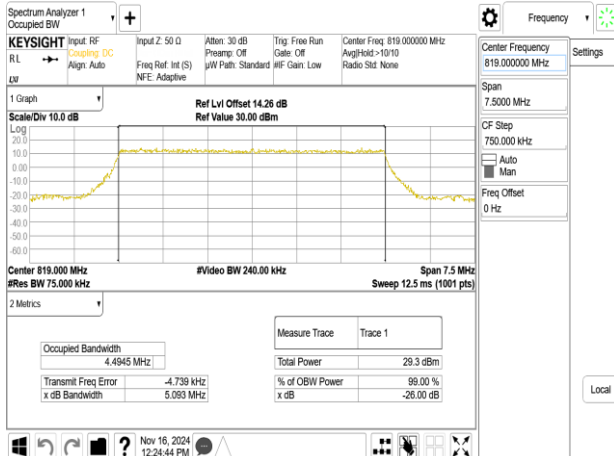
Band26-Part90s_5MHz_64QAM_RB25_0_CH26740
