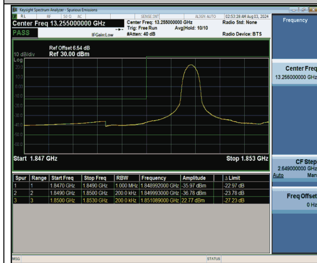
Band25_20MHz_QPSK_26140_1RB#0
