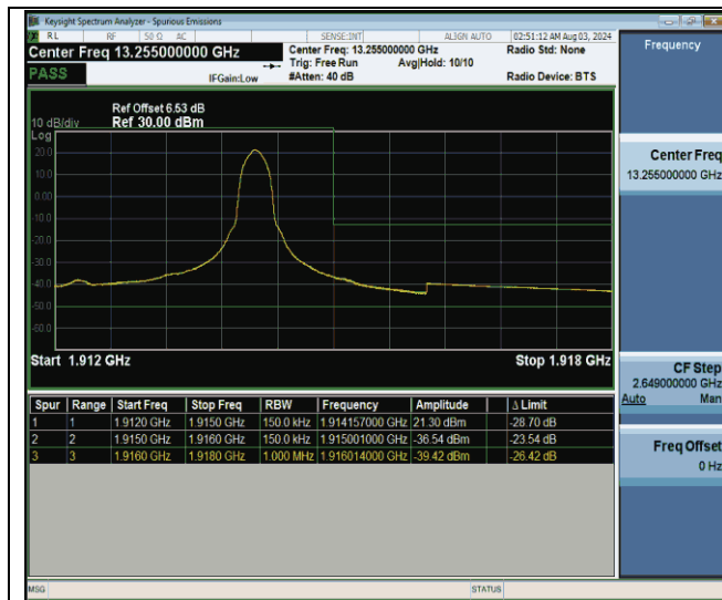
Band25_15MHz_QPSK_26615_1RB#74
