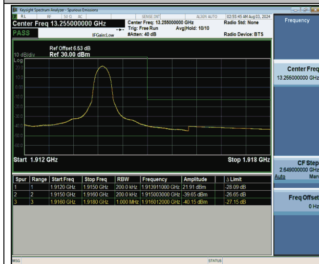
Band25_20MHz_QPSK_26590_1RB#99
