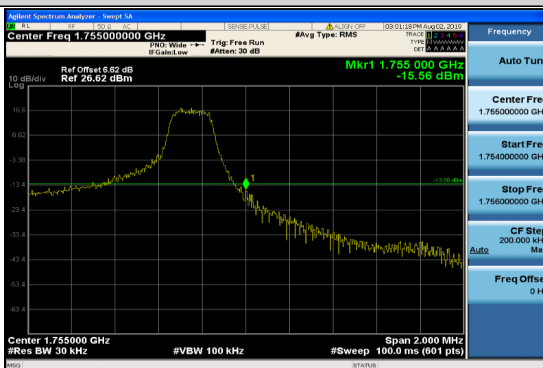
Band4-1.4MHz-QPSK-20393-1RB#5
