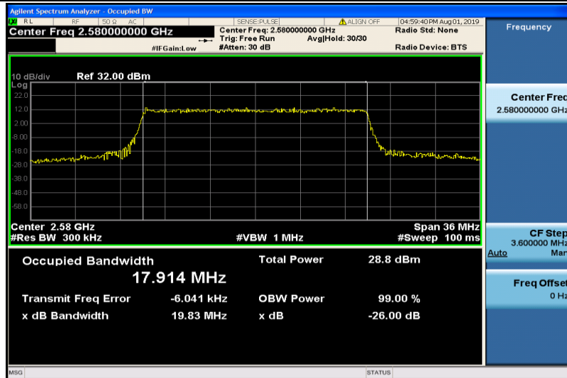
Band38-20MHz-16QAM-37850-100RB#0-17.914
