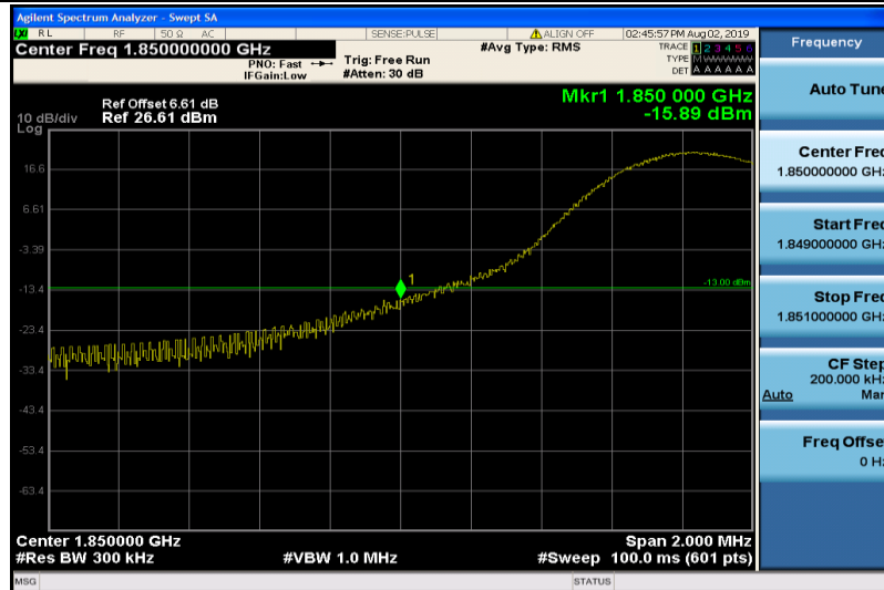
Band2-15MHz-16QAM-18675-1RB#0
