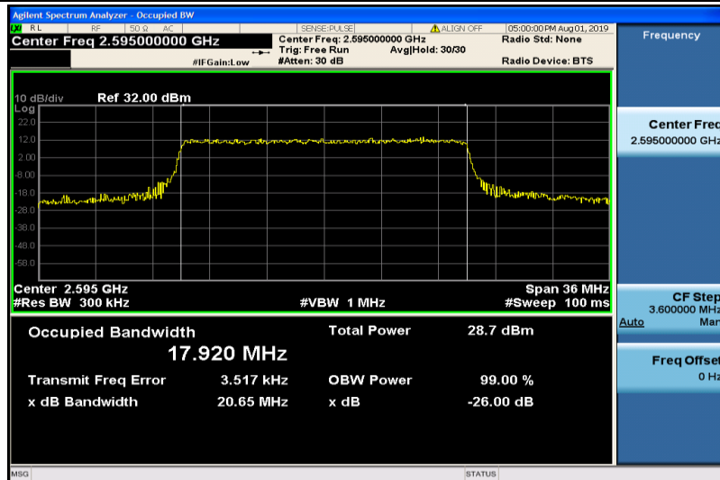
Band38-20MHz-16QAM-38000-100RB#0-17.920
