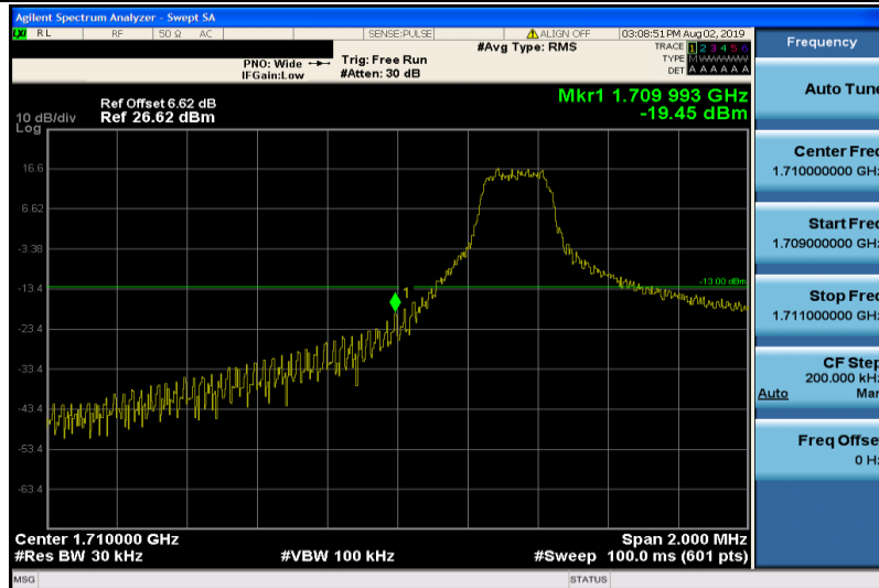
Band4-3MHz-16QAM-19965-1RB#0
