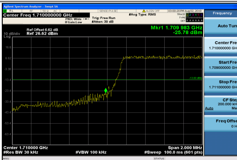
Band4-1.4MHz-QPSK-19957-6RB#0
