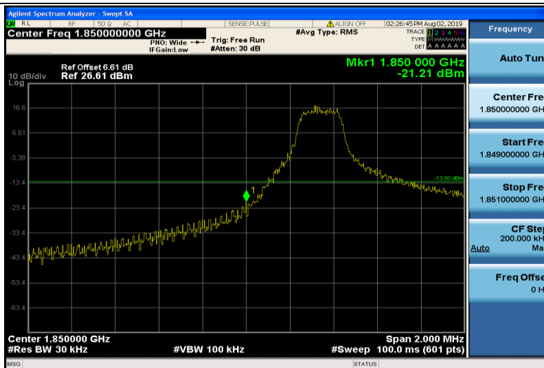
Band2-3MHz-16QAM-18615-1RB#0
