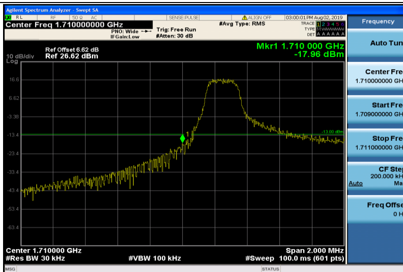
Band4-1.4MHz-QPSK-19957-1RB#0
