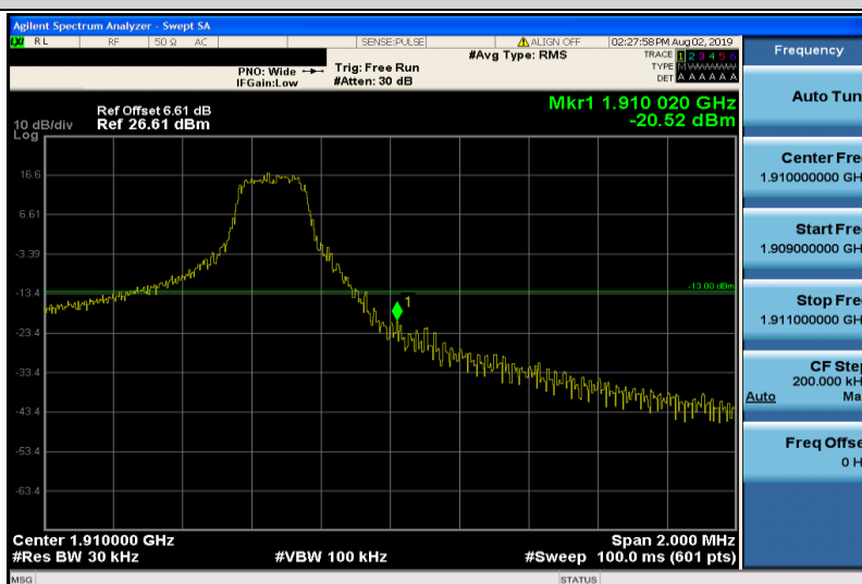
Band2-3MHz-16QAM-19185-1RB#14
