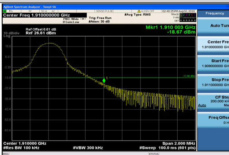
Band2-10MHz-QPSK-19150-1RB#49
