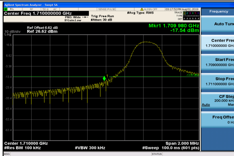
Band4-5MHz-QPSK-19975-1RB#0
