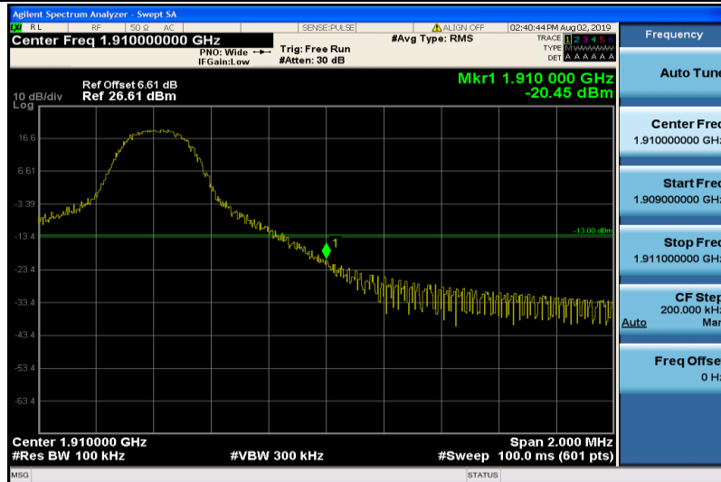
Band2-10MHz-16QAM-19150-1RB#49
