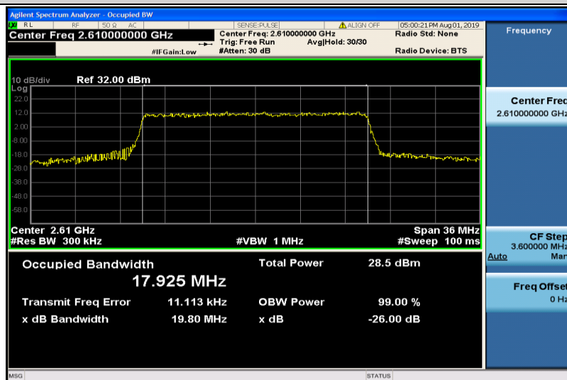
Band38-20MHz-16QAM-38150-100RB#0-17.925
