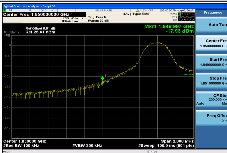
Band2-10MHz-16QAM-18650-1RB#0
