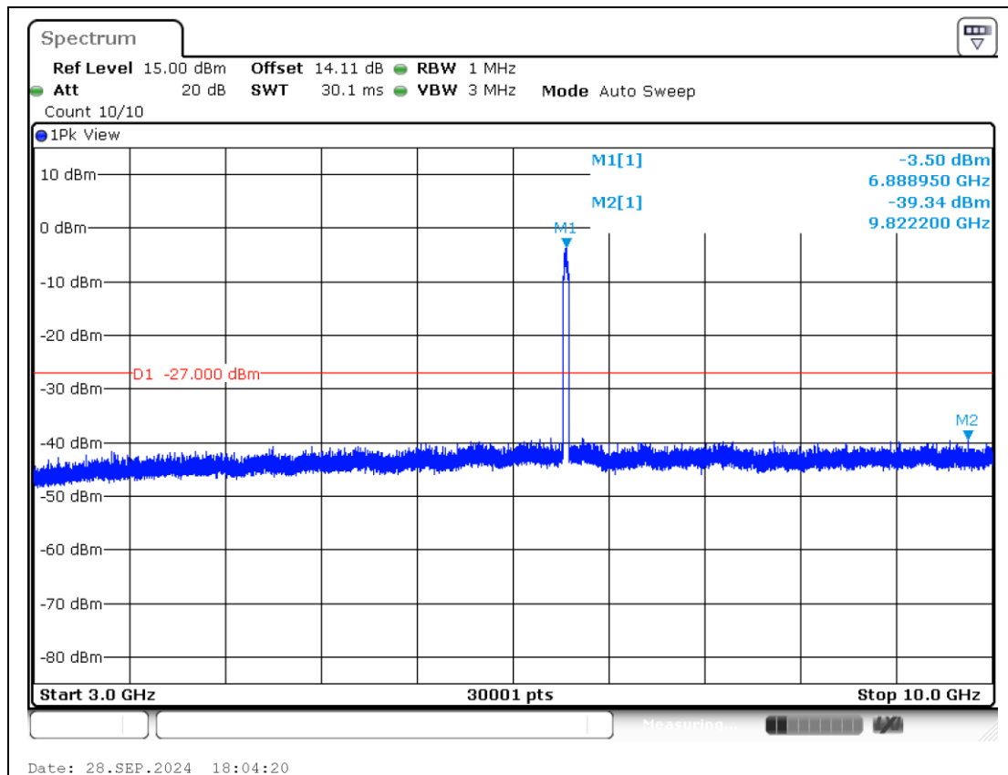
11AX40MIMO-Ant2-6885-3000~10000-PASS
