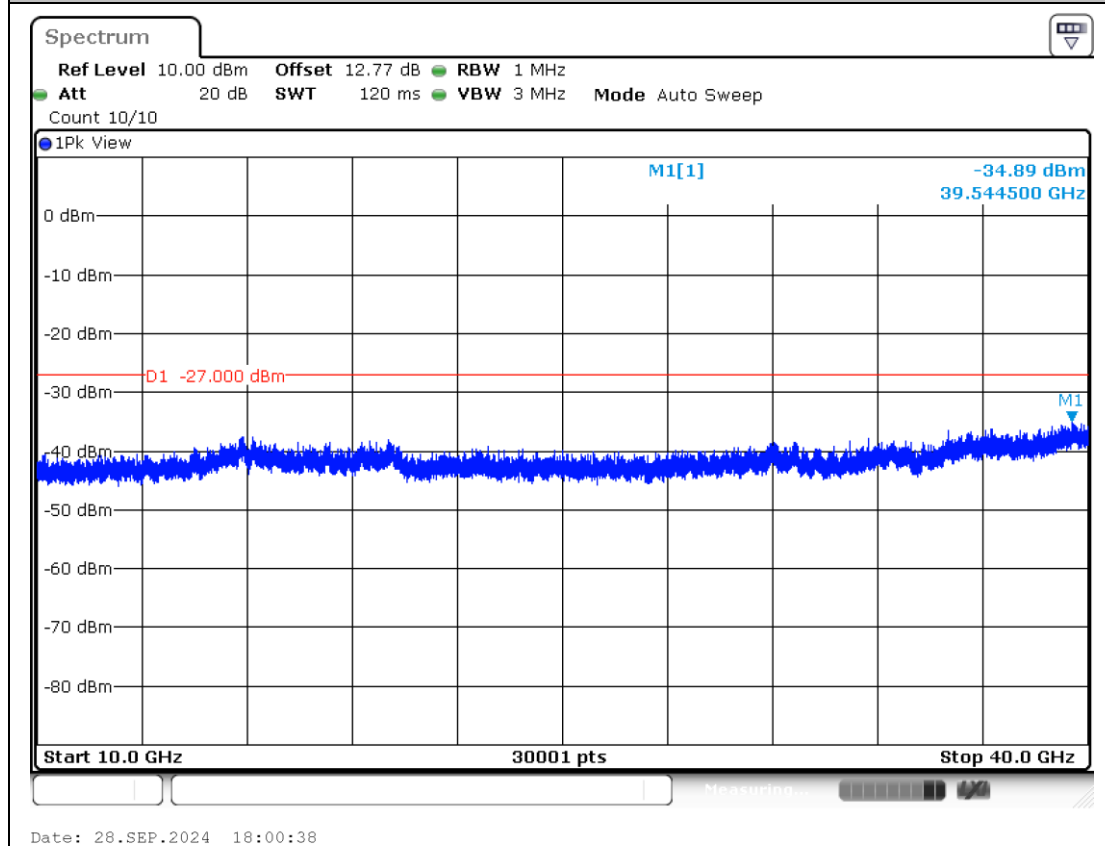
11AX40MIMO-Ant1-6845-10000~40000-PASS
