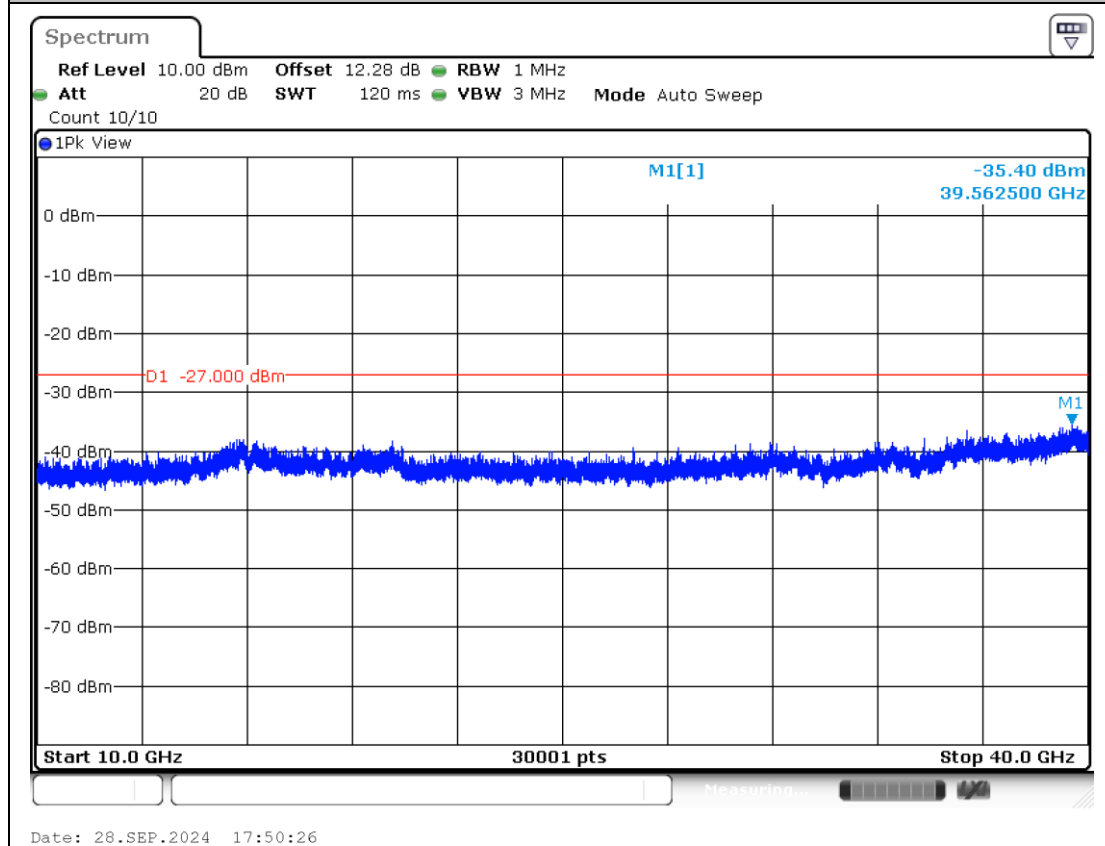
11AX40MIMO-Ant1-6525-10000~40000-PASS
