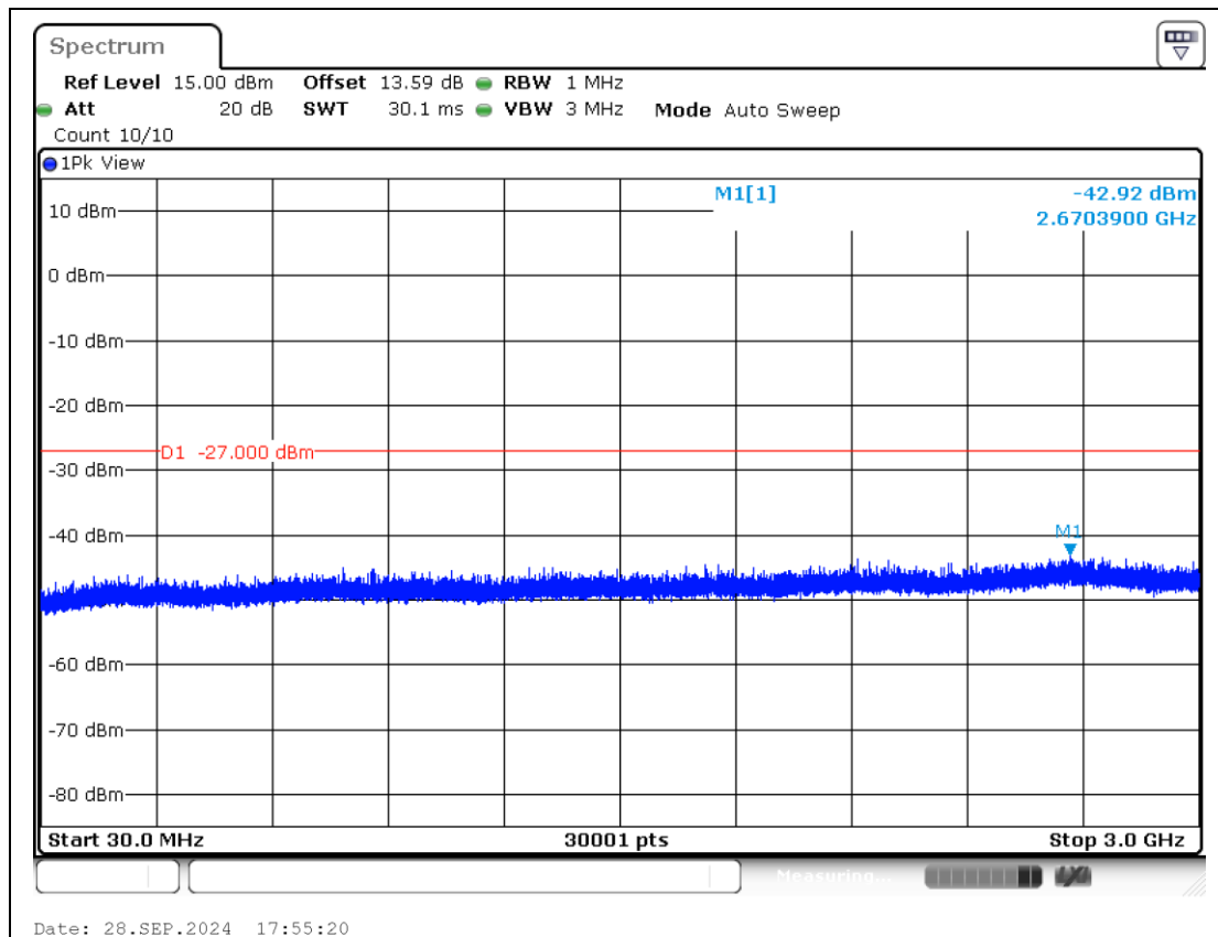
11AX40MIMO-Ant2-6565-30~3000-PASS
