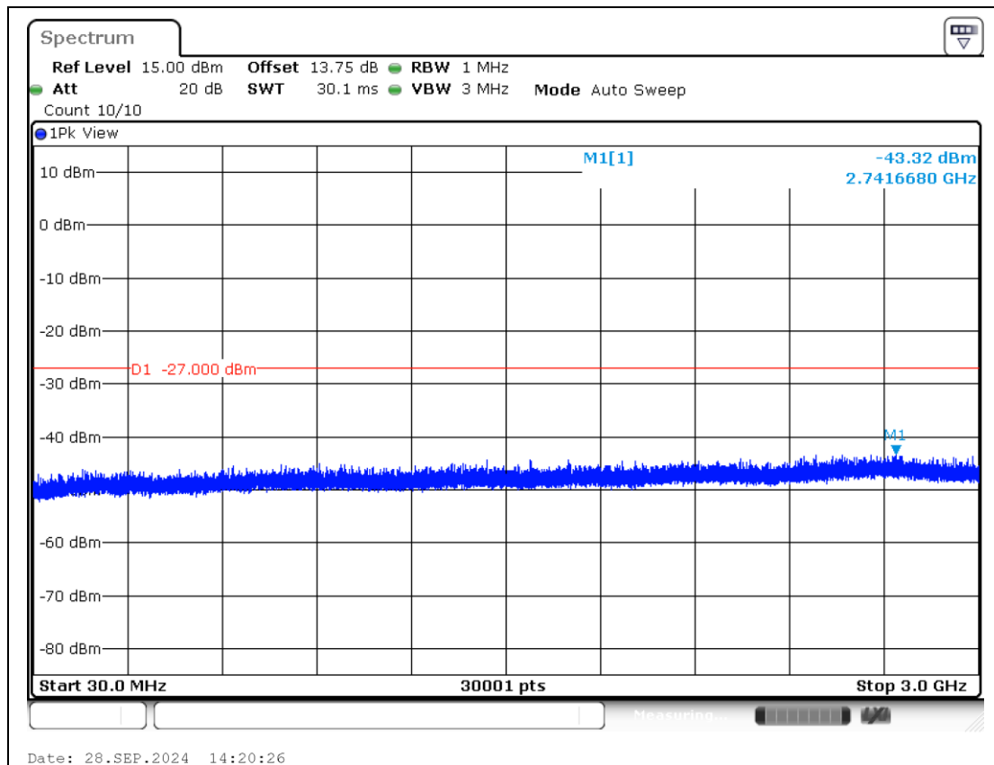
11AX40MIMO-Ant2-5965-30~3000-PASS
