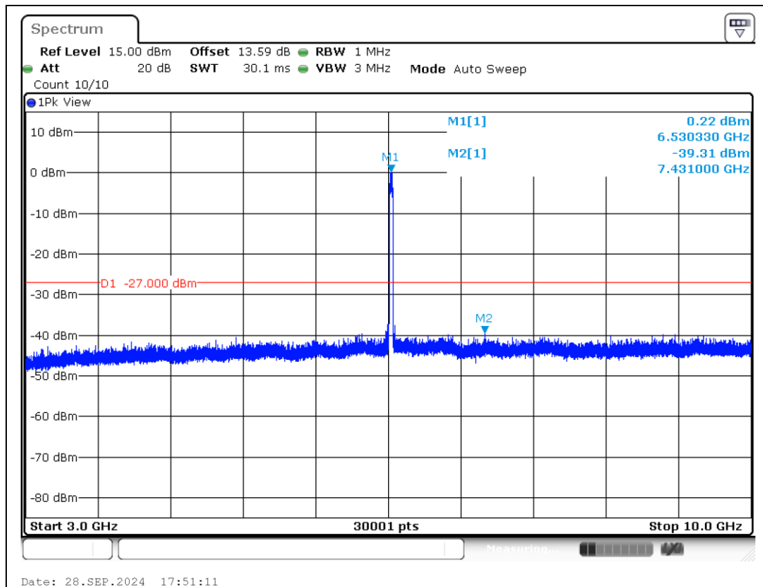
11AX40MIMO-Ant2-6525-3000~10000-PASS
