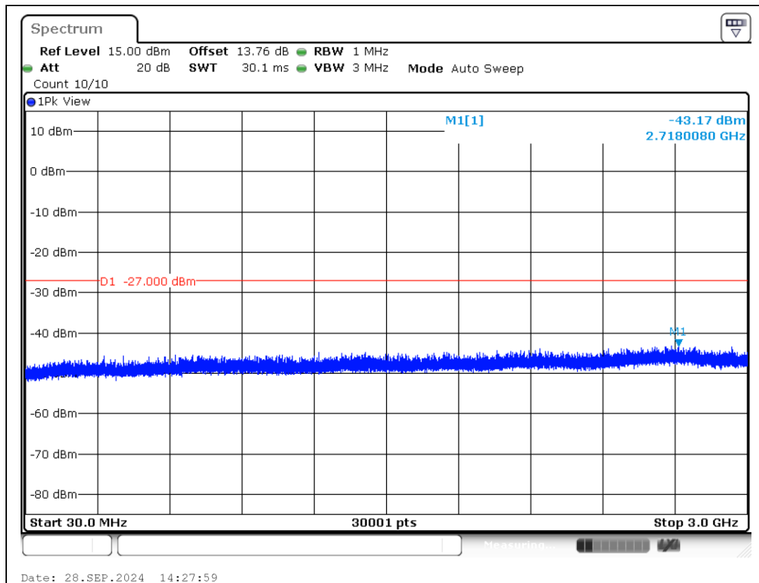
11AX40MIMO-Ant2-6405-30~3000-PASS
