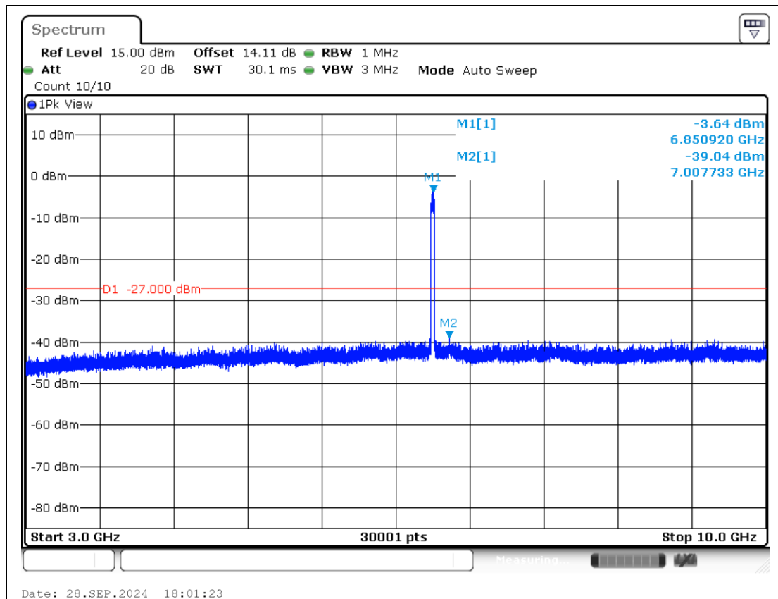
11AX40MIMO-Ant2-6845-3000~10000-PASS
