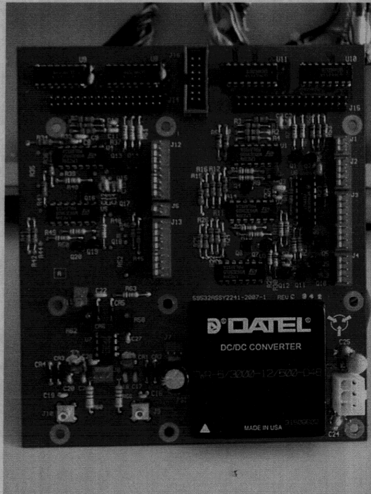
Figure 51. Front View of Relay Switch Board
