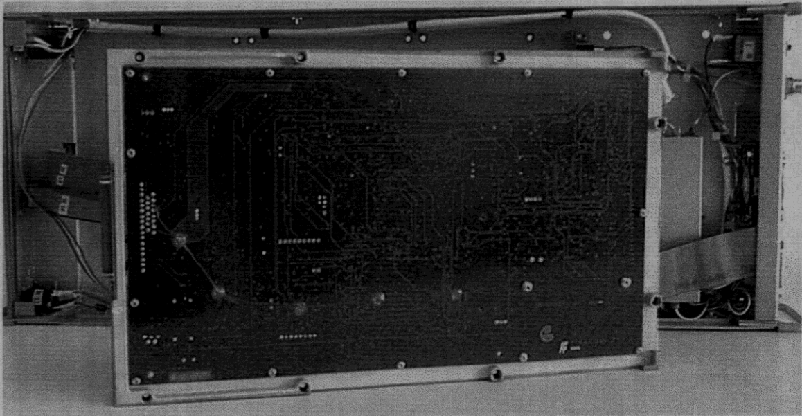
Figure 31. Bottom View of Digital Module
