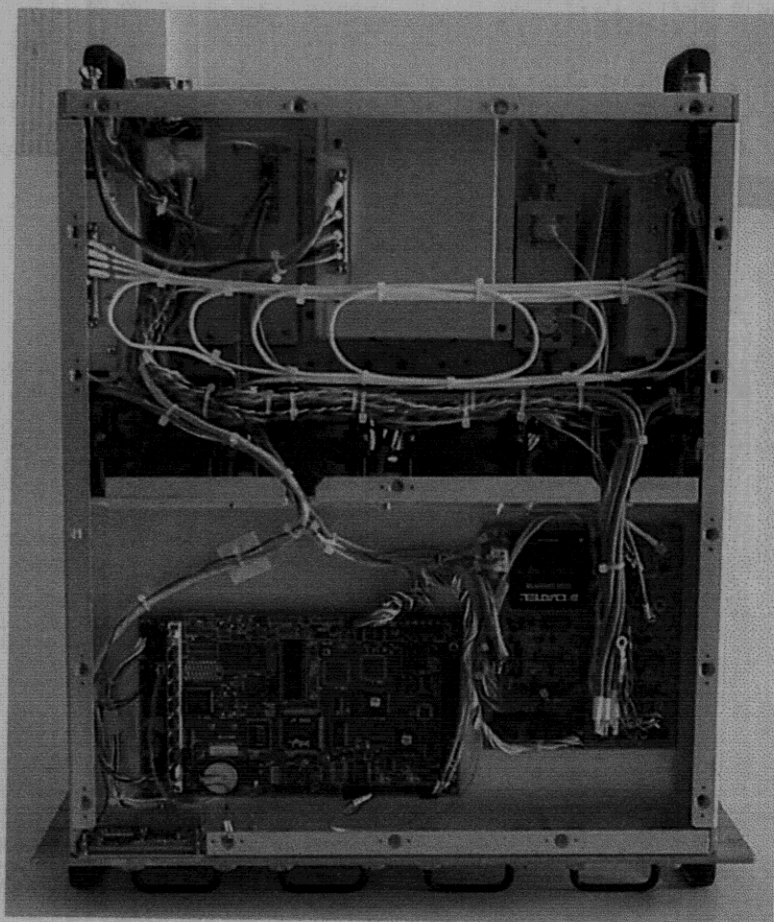
Figure 46. PA-5050A With Bottom Cover Removed
