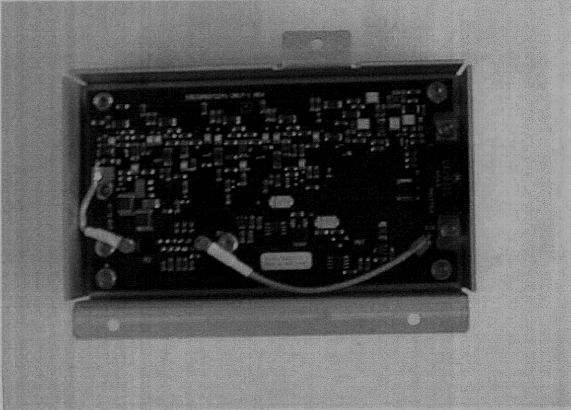
Figure 59. Bottom View of Pre-Driver Assembly (Removed)
