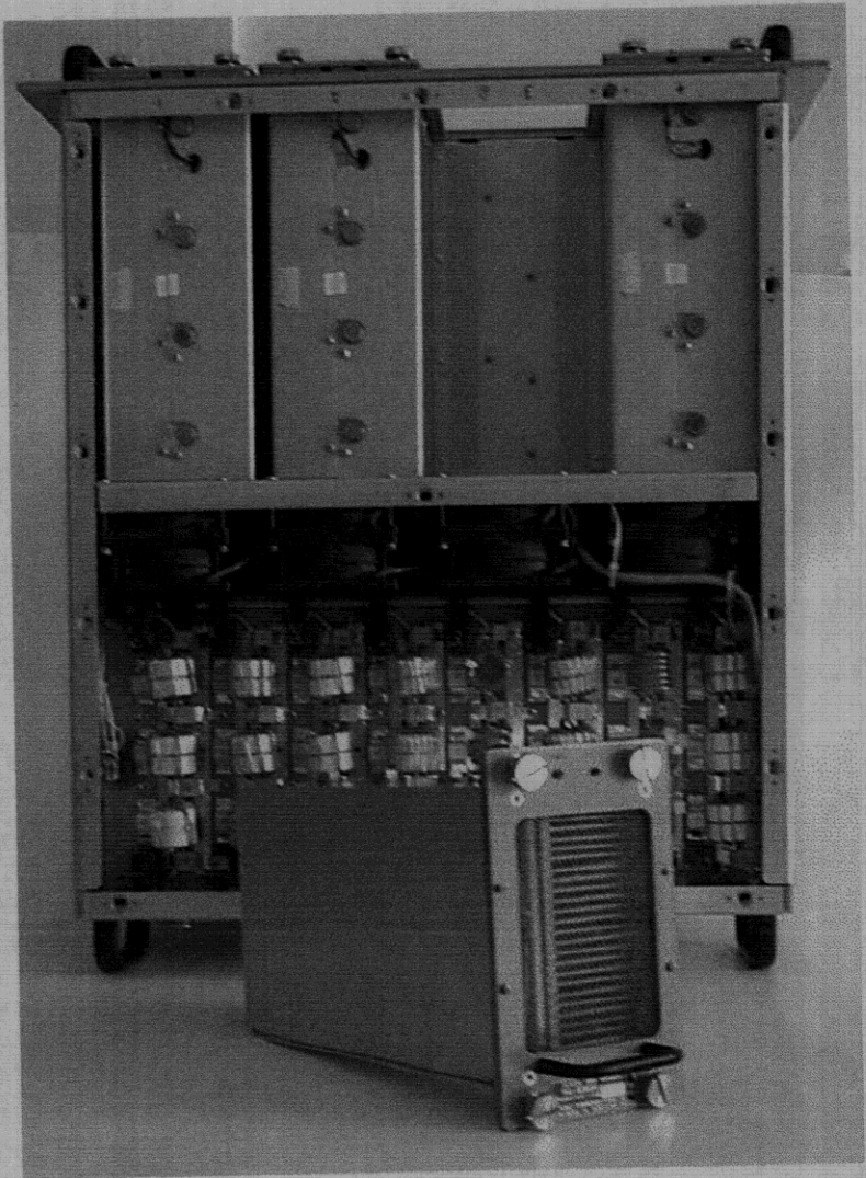
Figure 44. Front View of Power Amplifier Module (Removed)
