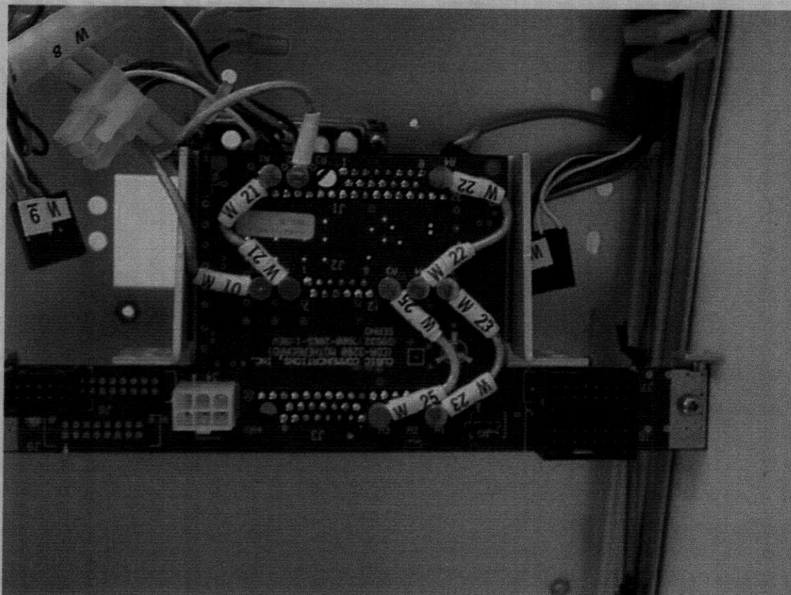
Figure 37. Top View of T-4180 Motherboard
