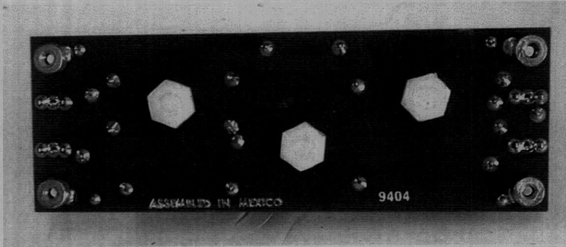
Figure 36. Bottom View of AC Line Filter (Removed)
