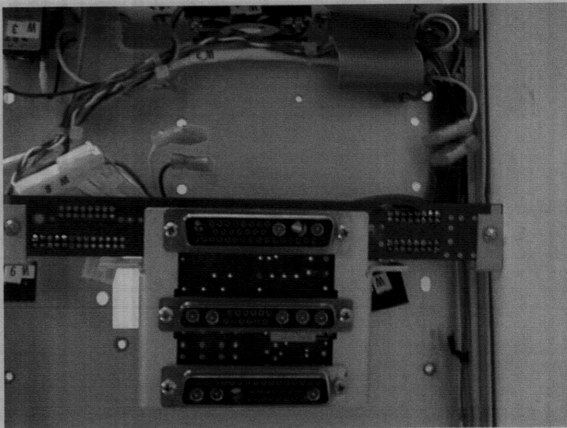
Figure 38. Bottom View of T-4180 Motherboard
