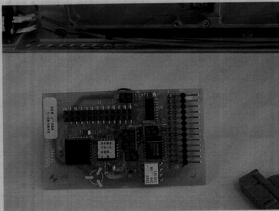
Figure 22. Front View of Remote Control Board (Removed)
