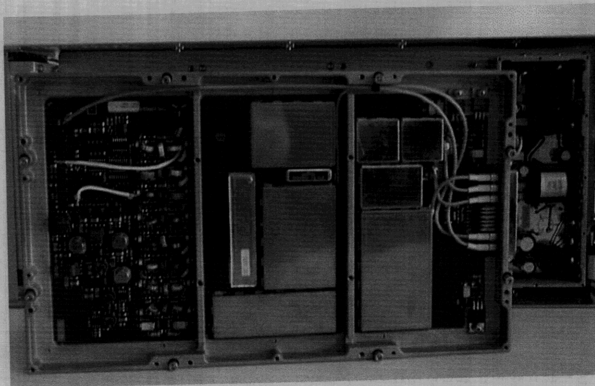
Figure 27. Top View of RF Analog Module (Removed)
