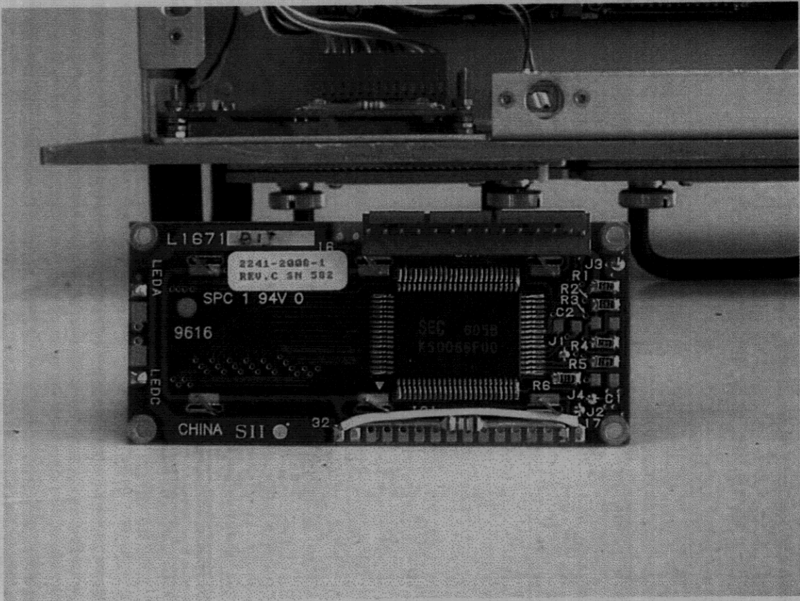
Figure 54. Rear View of Display Board
