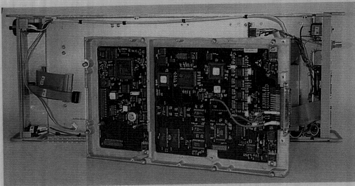
Figure 29. Digital Module (Removed)
