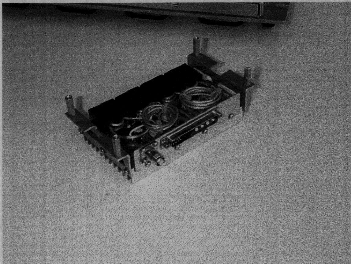
Figure 55. Combiner Assembly (Removed)
