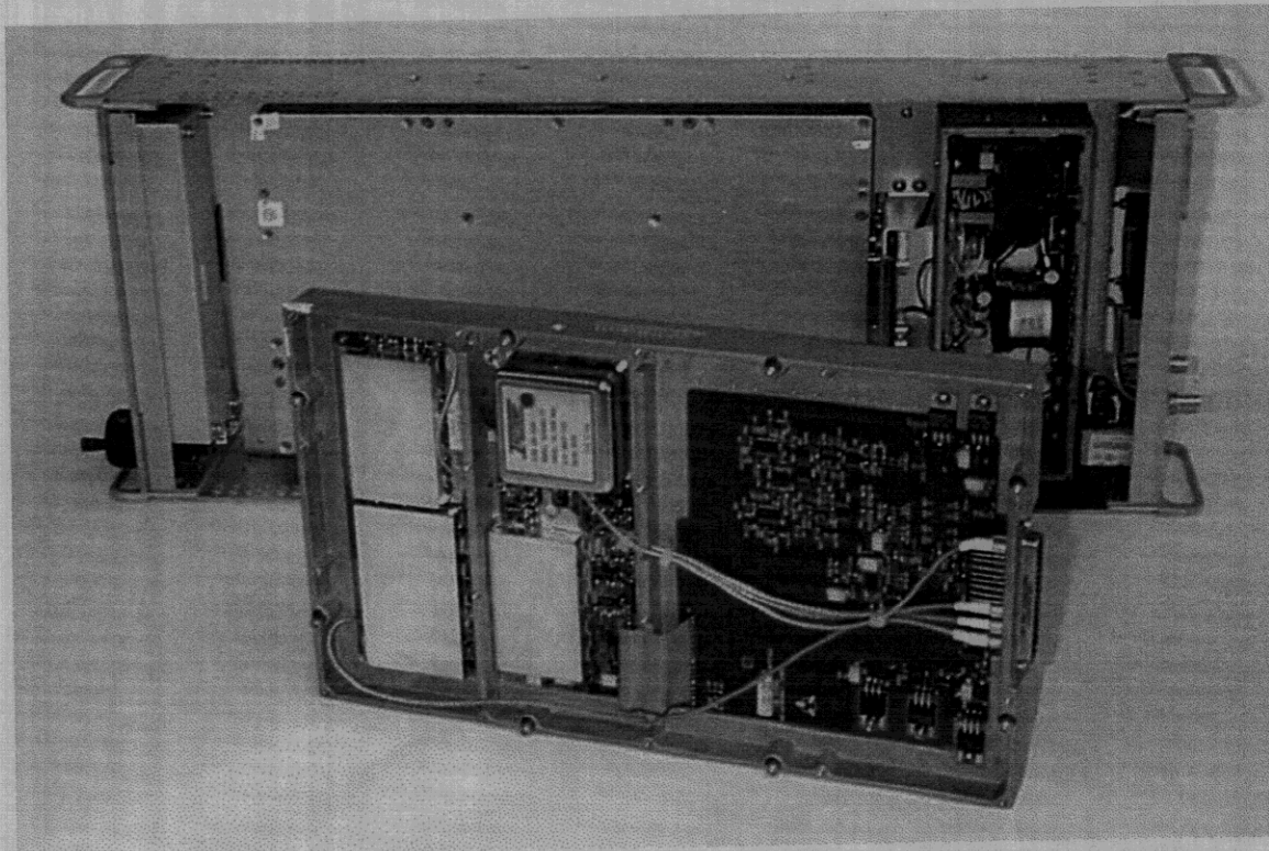
Figure 24. Front View of Synthesizer Module (Removed)
