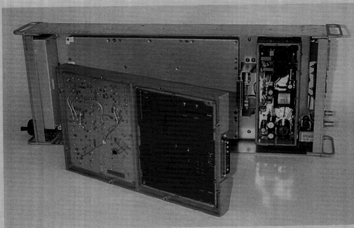
Figure 25. Rear View of Synthesizer Module (Removed)
