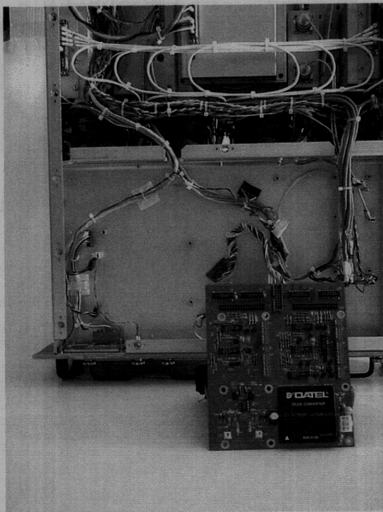
Figure 50. Relay Switch Board (Removed)
