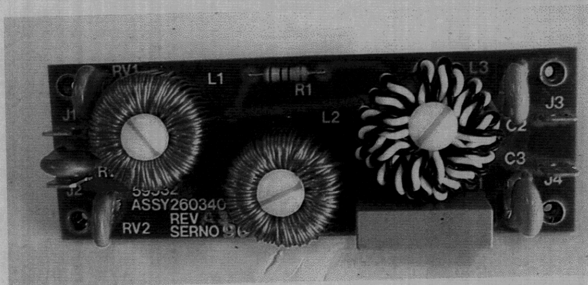
Figure 35. Top View of AC Line Filter (Removed)
