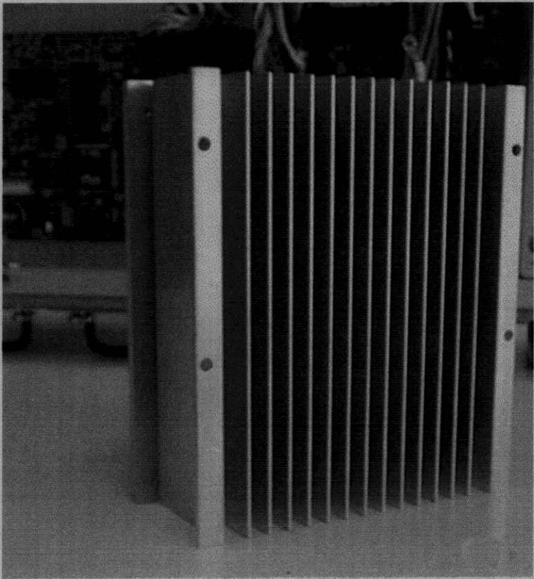
Figure 61. End View of PA Driver Assembly (Removed)
