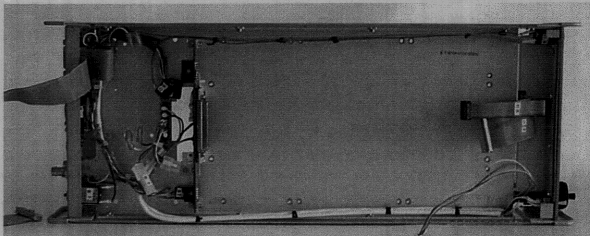
Figure 40. Bottom View of T-4180 Chassis
