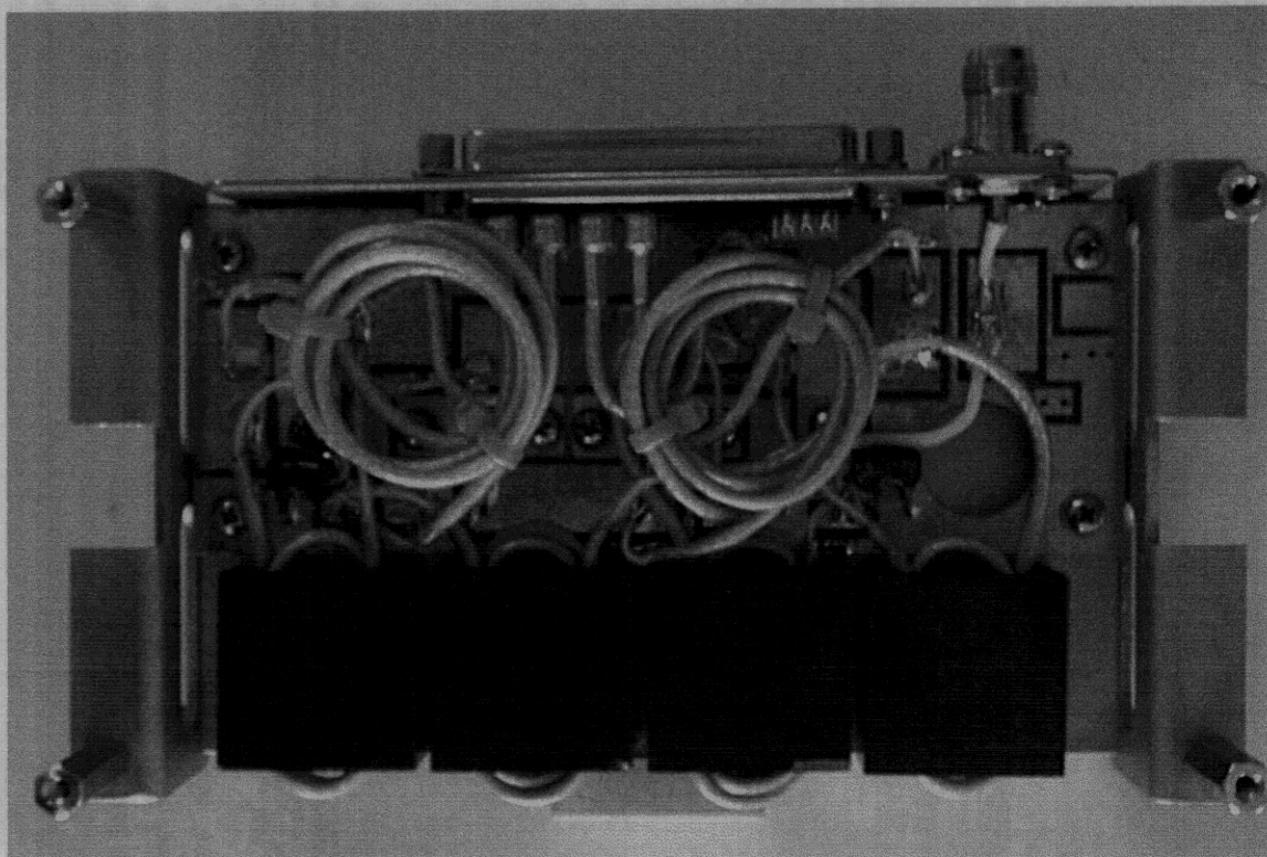
Figure 57. Top View of Combiner Assembly
