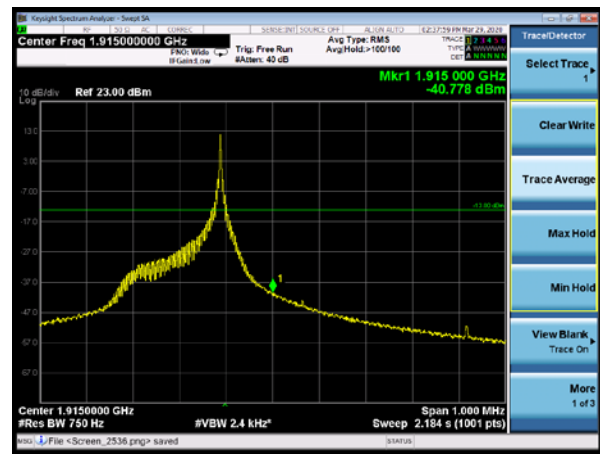
NB-IoT Band 25 QPSK 3.75kHz 1@47 CH-High
