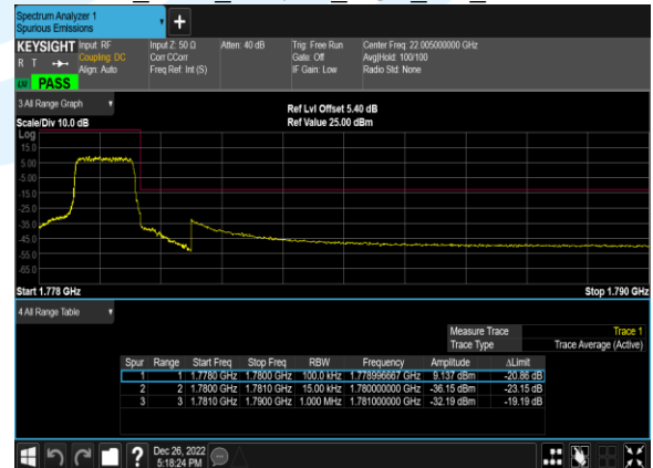
B66_1.4M_64QAM_6@0_CH_132665
