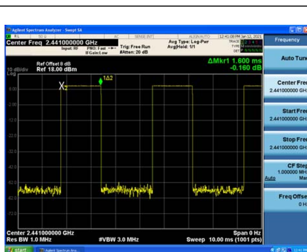
Modulation: GFSK DH3 2441
