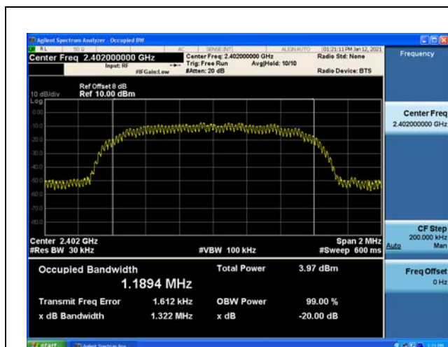
Modulation: \pi/4 DQPSK 2402MHz
