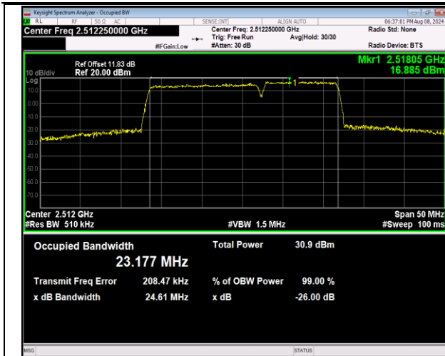
7-7-15MHz-10MHz-QPSK-QPSK-20825-20945-75RB#0-5 ORB#0-PASS
