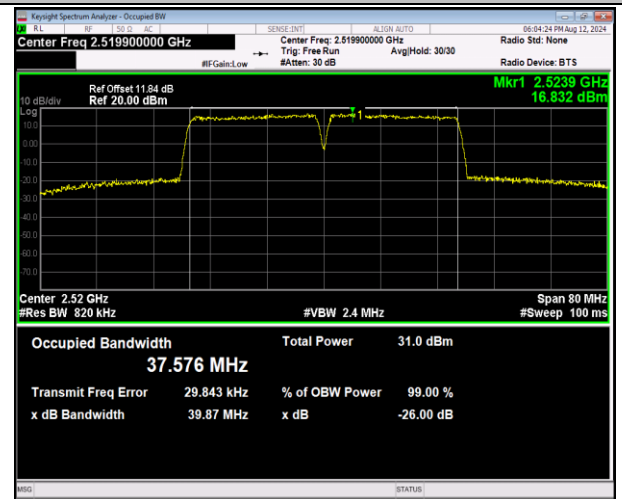
7-7-20MHz-20MHz-QPSK-QPSK-20850-21048-100RB#0-100RB#0-PASS
