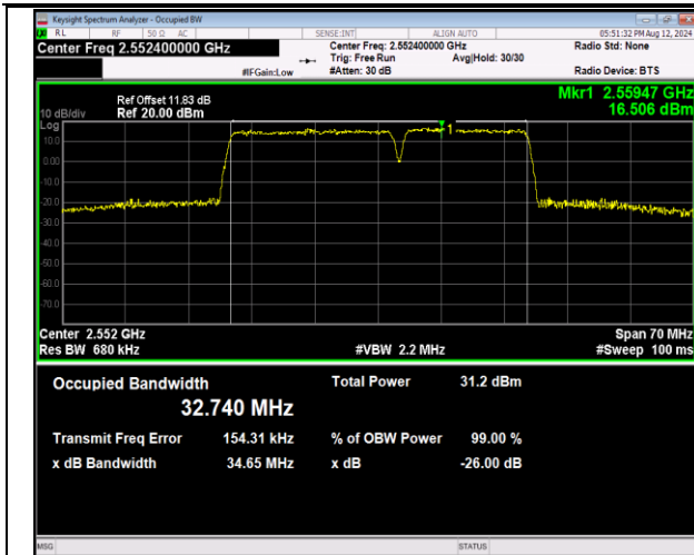
7-7-20MHz-15MHz-QPSK-QPSK-21201-21372-100RB#0-75RB#0-PASS
