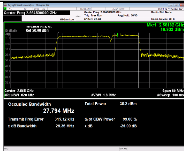
7-7-20MHz-10MHz-16QAM-16QAM-21251-21395-100RB#0-50RB#0-PASS
