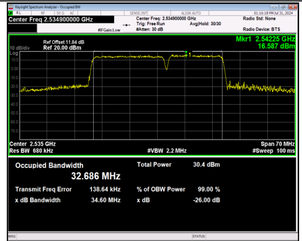
7-7-20MHz-15MHz-64QAM-64QAM-21026-21197-100RB#0-75RB#0-PASS
