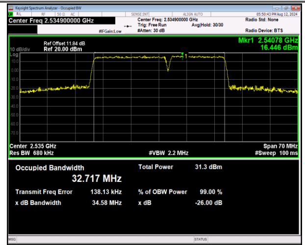
7-7-20MHz-15MHz-QPSK-QPSK-21026-21197-100RB#0-75RB#0-PASS
