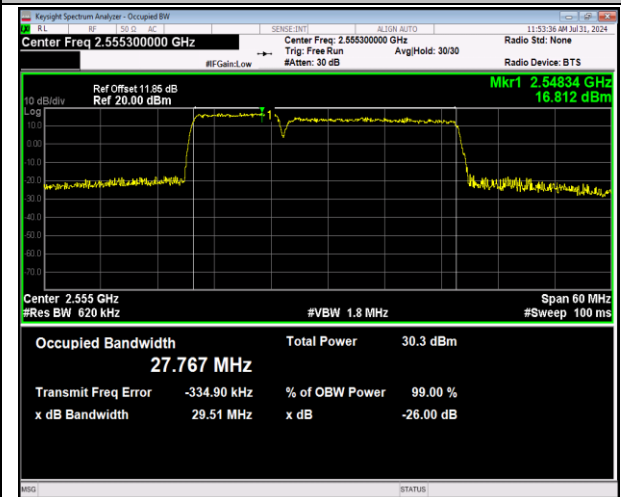
7-7-10MHz-20MHz-64QAM-64QAM-21206-21350-50RB#0-100RB#0-PASS
