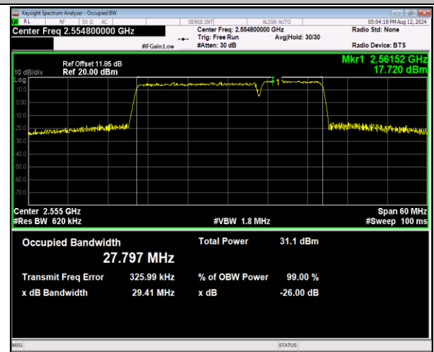
7-7-20MHz-10MHz-QPSK-QPSK-21251-21395-100RB#0-50RB#0-PASS
