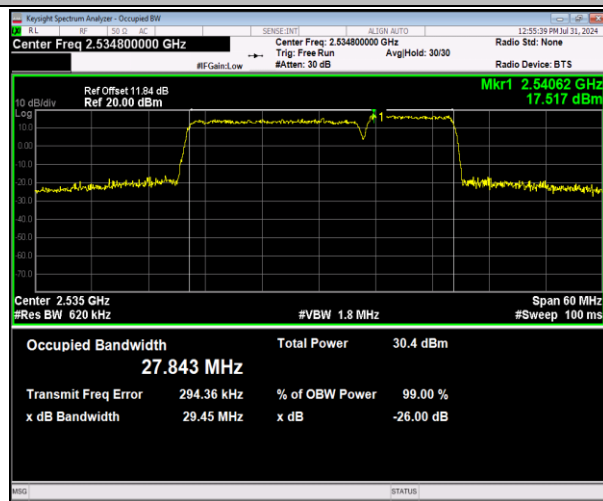
7-7-20MHz-10MHz-64QAM-64QAM-21051-21195-100RB#0-50RB#0-PASS
