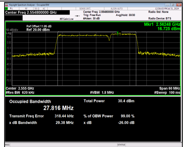
7-7-20MHz-10MHz-64QAM-64QAM-21251-21395-100RB#0-50RB#0-PASS
