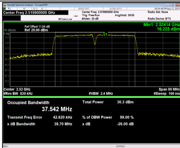
7-7-20MHz-20MHz-16QAM-16QAM-20850-21048-100RB#0-100RB#0-PASS
