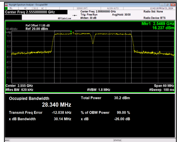
7-7-15MHz-15MHz-64QAM-64QAM-21225-21375-75RB #0-75RB#0-PASS
