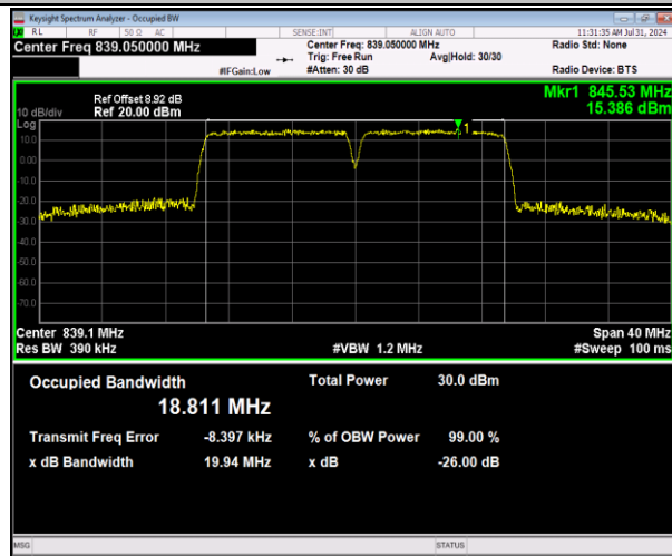
5-5-10MHz-10MHz-64QAM-64QAM-20501-20600-50RB# 0-50RB#0-PASS
