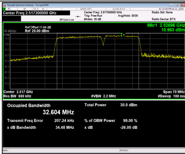
7-7-20MHz-15MHz-64QAM-64QAM-20850-21021-100RB#0-75RB#0-PASS
