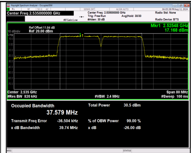
7-7-20MHz-20MHz-16QAM-16QAM-21001-21199-100RB#0-100RB#0-PASS
