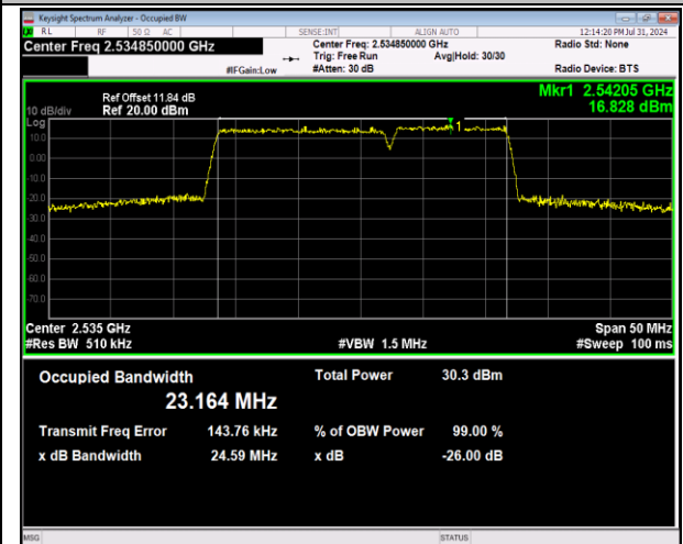
7-7-15MHz-10MHz-64QAM-64QAM-21051-21171-75RB #0-50RB#0-PASS
