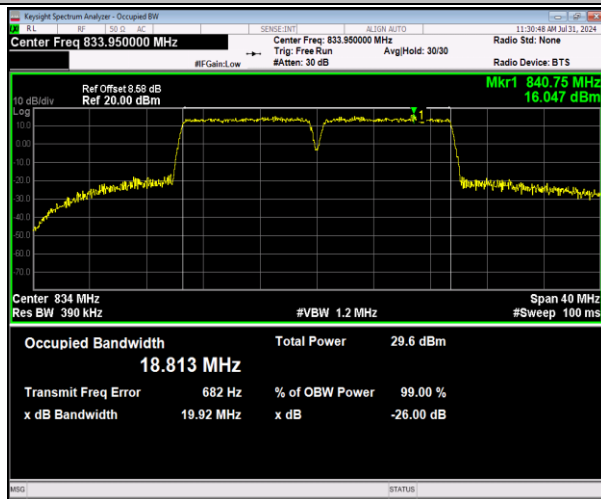
5-5-10MHz-10MHz-64QAM-64QAM-20450-20549-50RB#0-5 0-50RB#0-PASS
