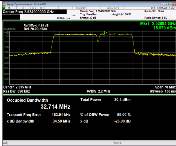
7-7-20MHz-15MHz-16QAM-16QAM-21026-21197-100RB#0-75RB#0-PASS
