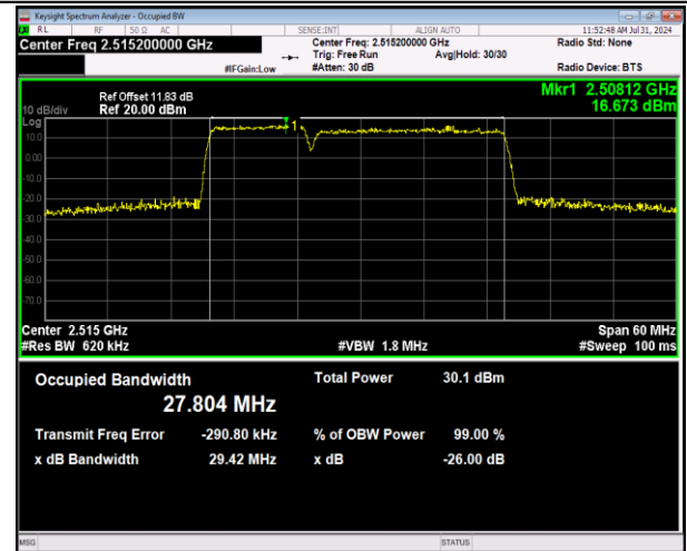
7-7-10MHz-20MHz-64QAM-64QAM-20805-20949-50RB #0-100RB#0-PASS
