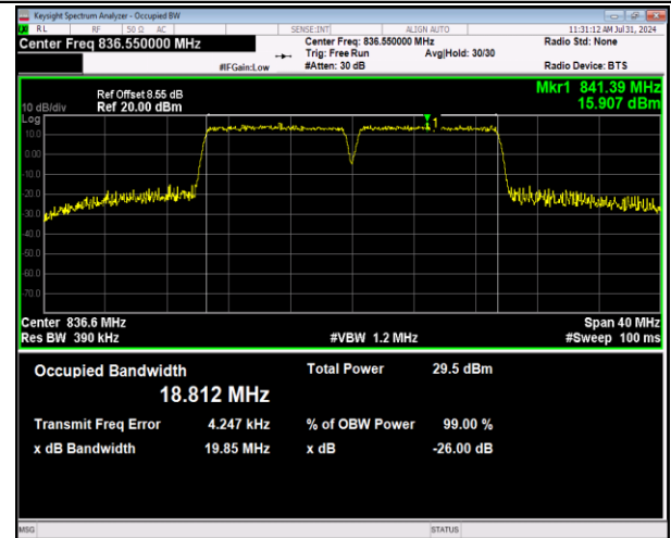
5-5-10MHz-10MHz-64QAM-64QAM-20476-20575-50RB#0-5 #0-50RB#0-PASS
