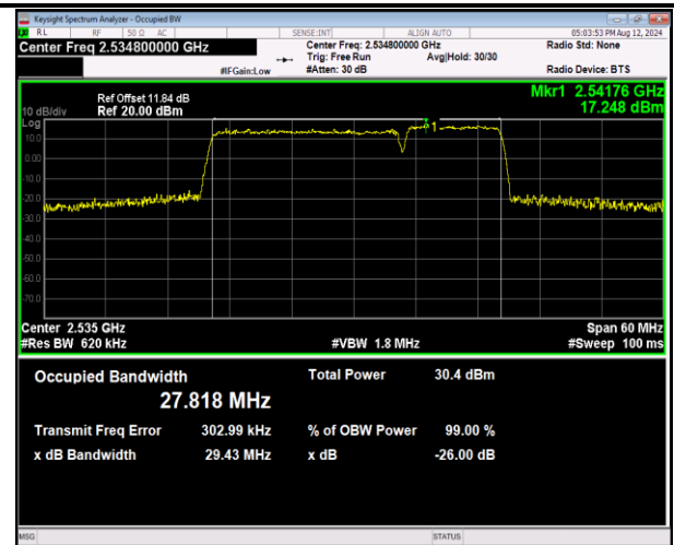
7-7-20MHz-10MHz-16QAM-16QAM-21051-21195-100RB#0-50RB#0-PASS
