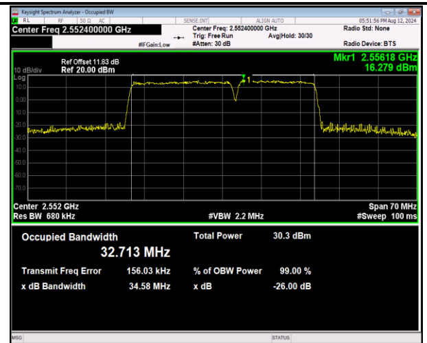
7-7-20MHz-15MHz-16QAM-16QAM-21201-21372-100RB#0-75RB#0-PASS
