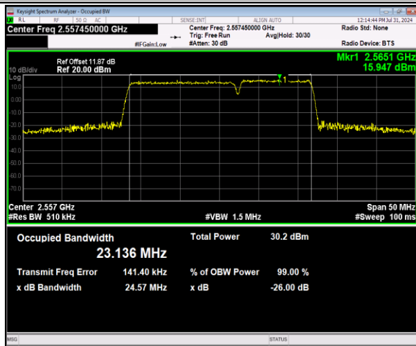
7-7-15MHz-10MHz-64QAM-64QAM-21277-21397-75RB#0-50RB#0-PASS
