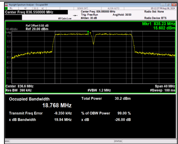
5-5-10MHz-10MHz-QPSK-QPSK-20476-20575-50RB#0-5 50RB#0-PASS
