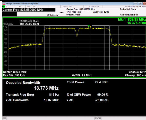
5-5-10MHz-10MHz-16QAM-16QAM-20476-20575-50RB#0-5 0-50RB#0-PASS
