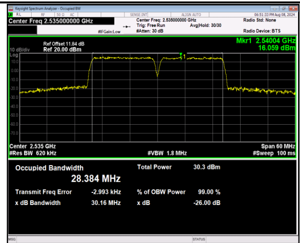
7-7-15MHz-15MHz-16QAM-16QAM-21025-21175-75RB #0-75RB#0-PASS
