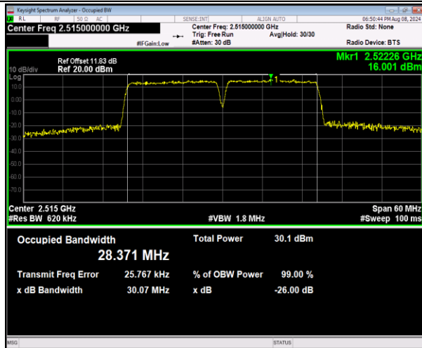
7-7-15MHz-15MHz-16QAM-16QAM-20825-20975-75RB#0-75RB#0-PASS
