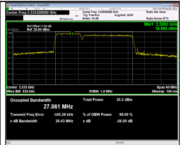
7-7-10MHz-20MHz-16QAM-16QAM-21006-21150-50RB#0-100RB#0-PASS
