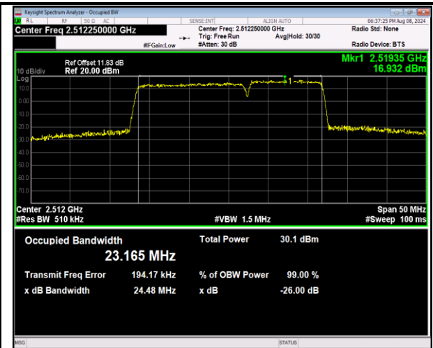
7-7-15MHz-10MHz-16QAM-16QAM-20825-20945-75RB #0-50RB#0-PASS
