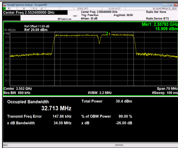
7-7-20MHz-15MHz-64QAM-64QAM-21201-21372-100RB#0-75RB#0-PASS
