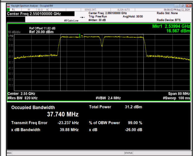
7-7-20MHz-20MHz-QPSK-QPSK-21152-21350-100RB#0-100RB#0-PASS
