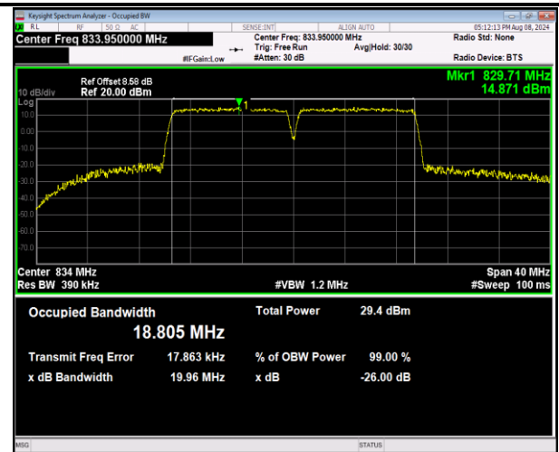
5-5-10MHz-10MHz-16QAM-16QAM-20450-20549-50RB#0-5 #0-50RB#0-PASS
