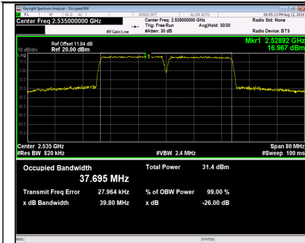
7-7-20MHz-20MHz-QPSK-QPSK-21001-21199-100RB#0-100RB#0-PASS
