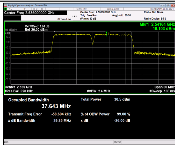
7-7-20MHz-20MHz-64QAM-64QAM-21001-21199-100RB#0-100RB#0-PASS
