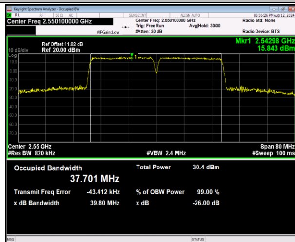
7-7-20MHz-20MHz-16QAM-16QAM-21152-21350-100RB#0-100RB#0-PASS
