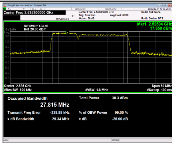
7-7-10MHz-20MHz-64QAM-64QAM-21006-21150-50RB#0-100RB#0-PASS
