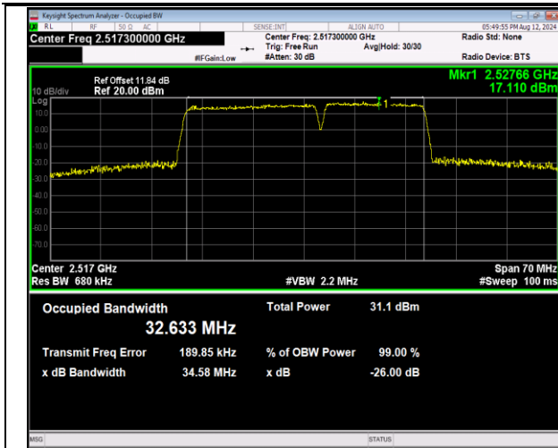
7-7-20MHz-15MHz-QPSK-QPSK-20850-21021-100RB#0-75RB#0-PASS
