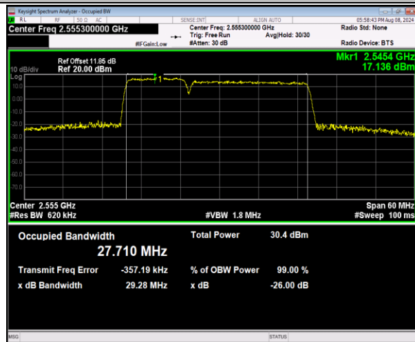
7-7-10MHz-20MHz-16QAM-16QAM-21206-21350-50RB#0-100RB#0-PASS
