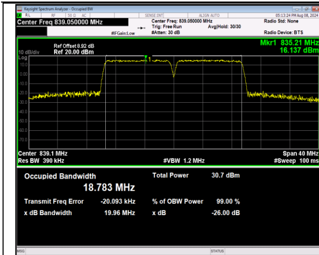
5-5-10MHz-10MHz-QPSK-QPSK-20501-20600-50RB#0-5 ORB#0-PASS
