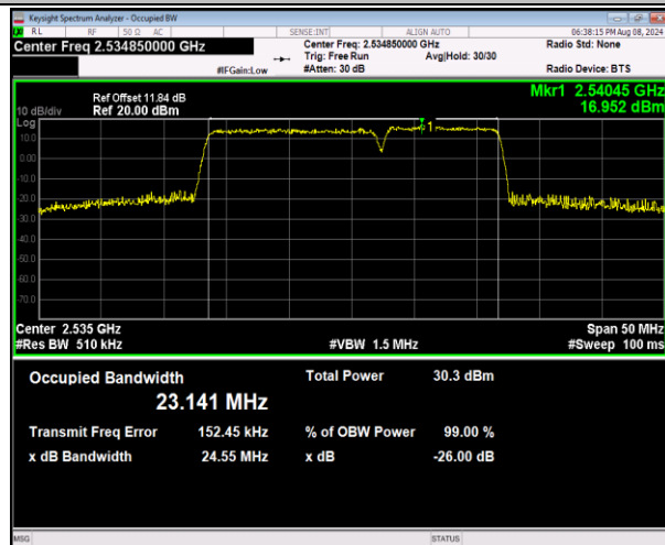
7-7-15MHz-10MHz-16QAM-16QAM-21051-21171-75RB# 0-50RB#0-PASS
