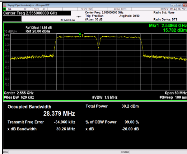
7-7-15MHz-15MHz-16QAM-16QAM-21225-21375-75RB# 0-75RB#0-PASS
