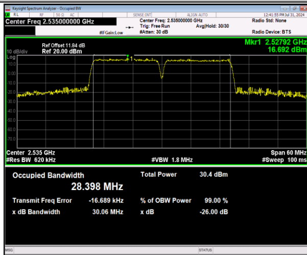
7-7-15MHz-15MHz-64QAM-64QAM-21025-21175-75RB# 0-75RB#0-PASS
