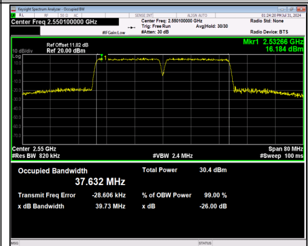
7-7-20MHz-20MHz-64QAM-64QAM-21152-21350-100RB#0-100RB#0-PASS
