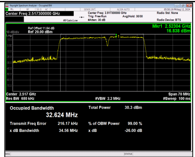
7-7-20MHz-15MHz-16QAM-16QAM-20850-21021-100RB#0-75RB#0-PASS
