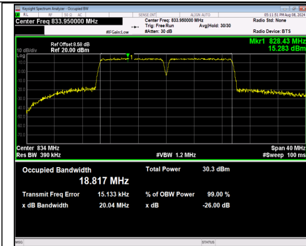
5-5-10MHz-10MHz-QPSK-QPSK-20450-20549-50RB#0-5 ORB#0-PASS
