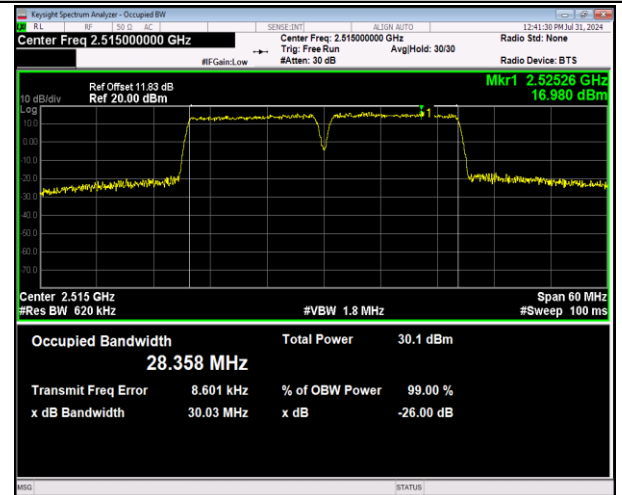
7-7-15MHz-15MHz-64QAM-64QAM-20825-20975-75RB#0-75RB#0-PASS
