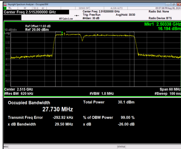
7-7-10MHz-20MHz-16QAM-16QAM-20805-20949-50RB# 0-100RB#0-PASS
