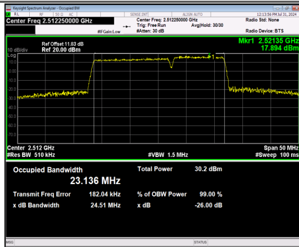
7-7-15MHz-10MHz-64QAM-64QAM-20825-20945-75RB# 0-50RB#0-PASS
