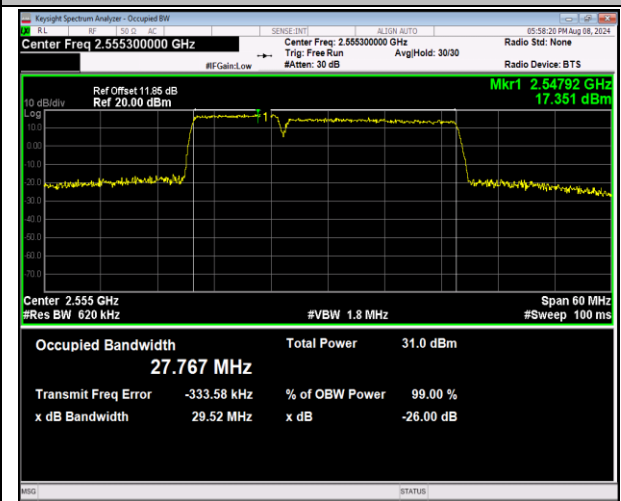
7-7-10MHz-20MHz-QPSK-QPSK-21206-21350-50RB#0-100RB#0-PASS
