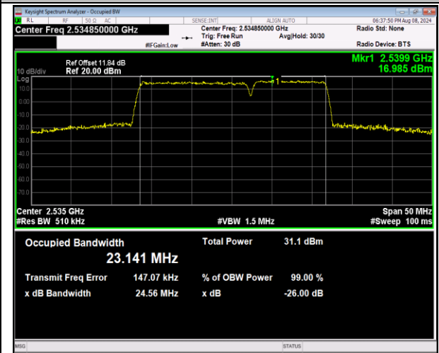
7-7-15MHz-10MHz-QPSK-QPSK-21051-21171-75RB#0- 50RB#0-PASS
