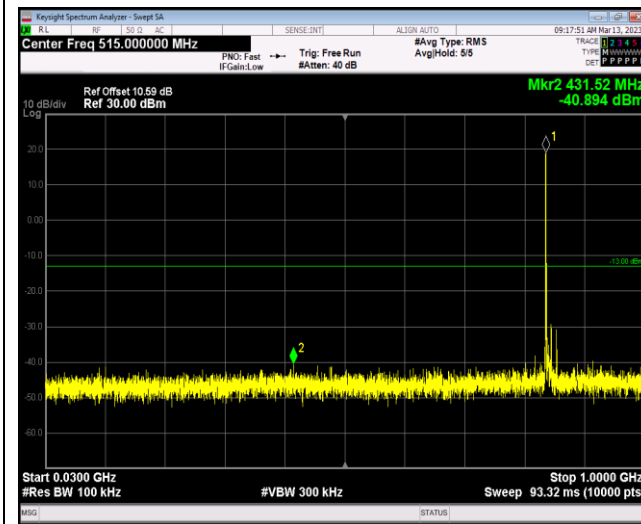
Band7-5MHz-QPSK-20775-1RB#0-Range1:30~1000MHz
