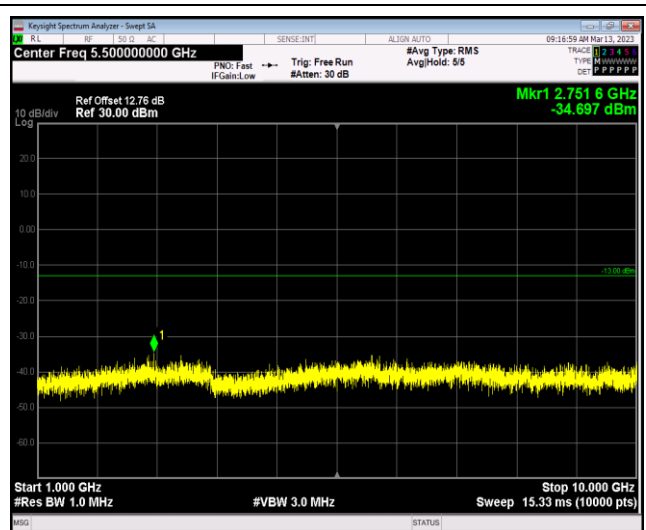
Band5-10MHz-64QAM-20600-1RB#0-Range2:1000~10000MHz
