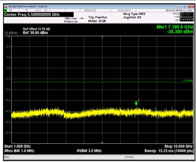
Band5-1.4MHz-64QAM-20643-1RB#0-Range2:1000~10000MHz
