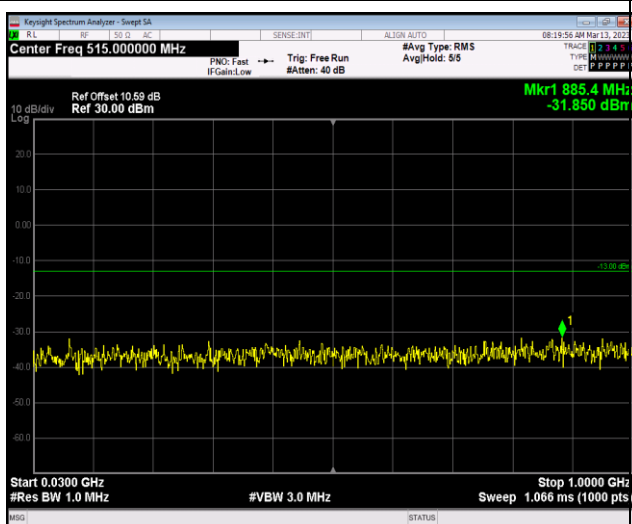
Band4-1.4MHz-16QAM-20175-1RB#0-Range1:30~ 1000MHz
