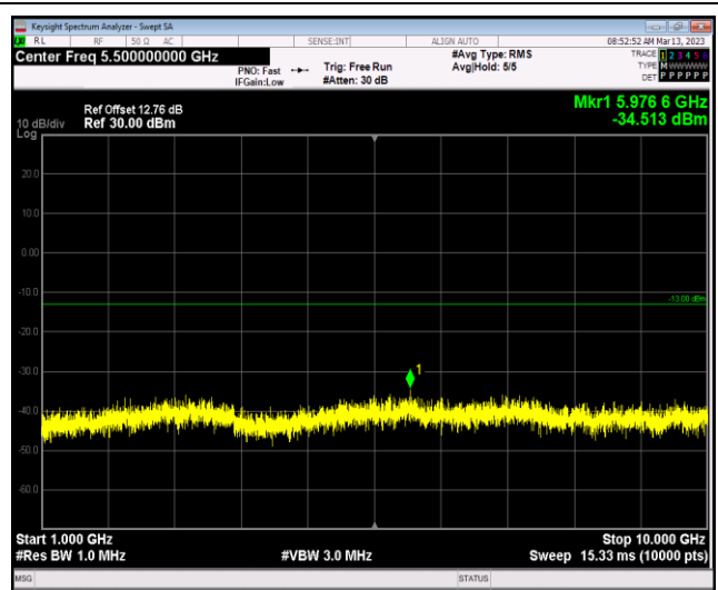
Band5-1.4MHz-64QAM-20525-1RB#0-Range2:1000~10000MHz
