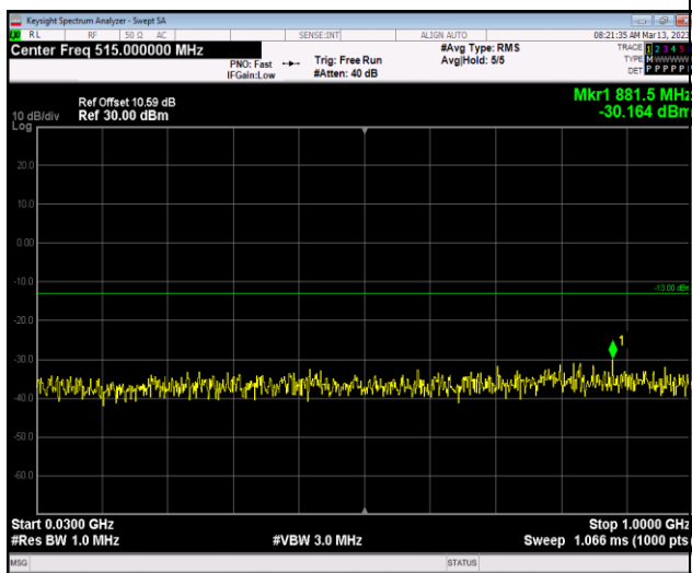
Band4-1.4MHz-16QAM-19957-1RB#0-Range1:30~ 1000MHz
