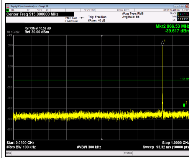
Band5-1.4MHz-64QAM-20643-1RB#0-Range1:30~1000MHz
