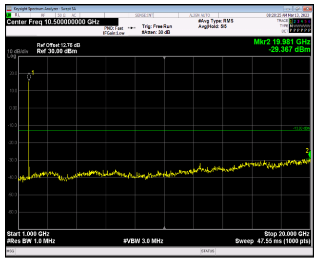
Band4-1.4MHz-64QAM-19957-1RB#0-Range2:1000~20000MHz
