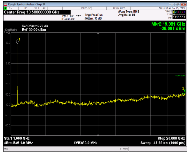
Band4-20MHz-64QAM-20175-1RB#0-Range2:1000~20000MHz
