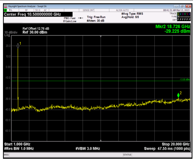
Band4-20MHz-64QAM-20175-1RB#0-Range2:1000~20000MHz
