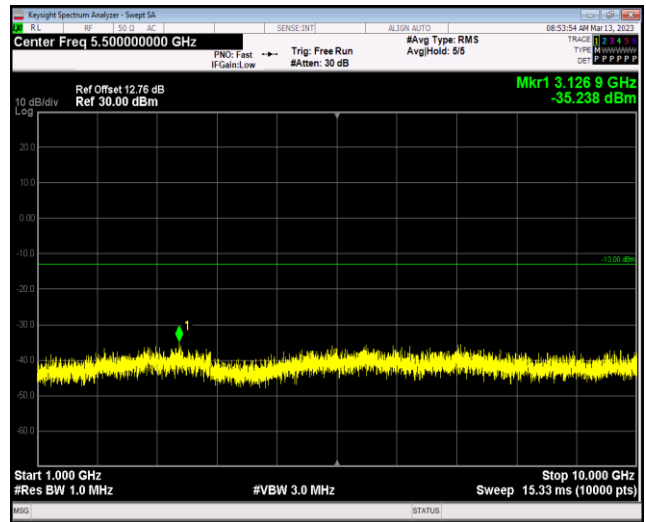
Band5-1.4MHz-64QAM-20643-1RB#0-Range2:1000~10000MHz
