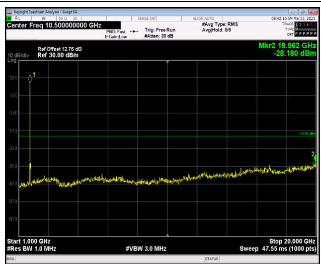
Band4-20MHz-64QAM-20050-1RB#0-Range2:1000~20000MHz
