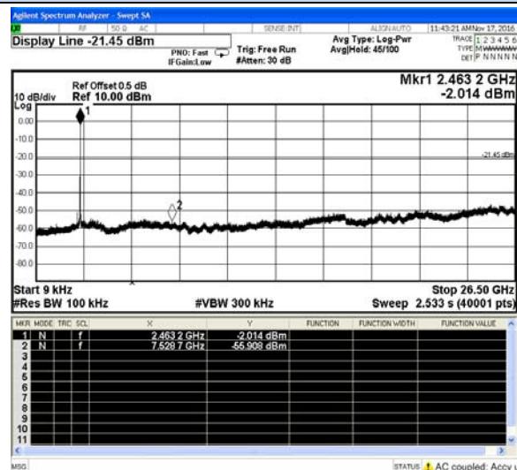
IEEE 802.11g-High channel
