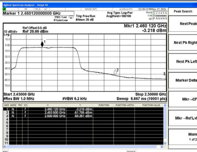
802.11n(HT20)-High channel(Average)
