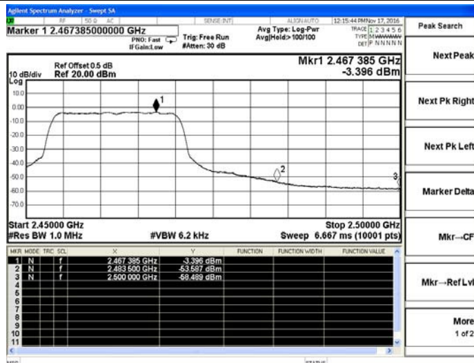
802.11g-High channel(Average)
