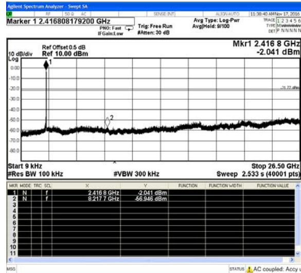
IEEE 802.11g-Low channel
