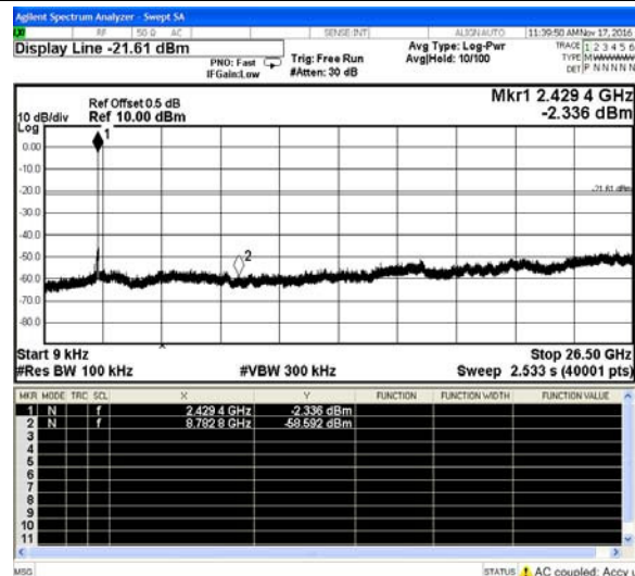
IEEE 802.11g-Middle channel
