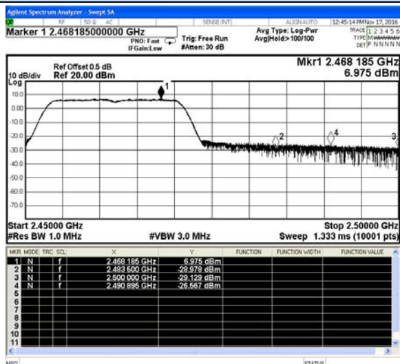
802.11n(HT20)-High channel(Peak)
