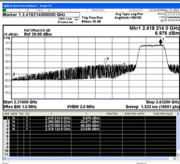
802.11n(HT20)-Low channel(Peak)
