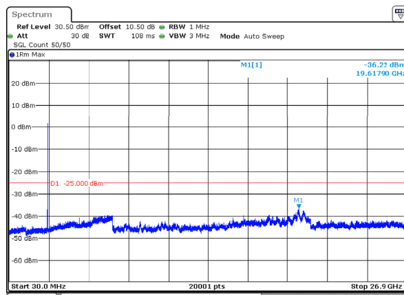
n41_40MHz_30kHz_2592.99MHz_DFT-s-OFDM QPSK_RB1@105 -36.22dBm
