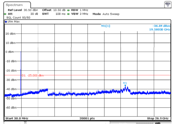
n41_15MHz_30kHz_2592.99MHz_DFT-s-OFDM QPSK_RB1@37 -36.89dBm
