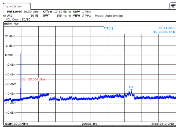
n41_50MHz_30kHz_2592.99MHz_DFT-s-OFDM QPSK_RB1@132 -36.91dBm
