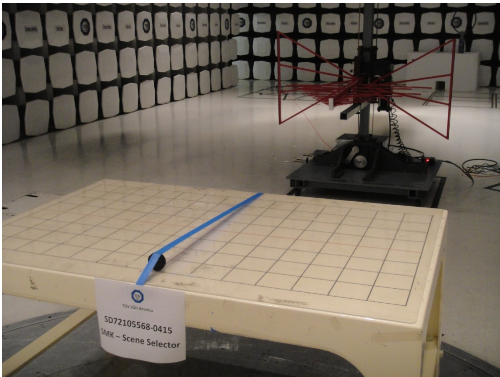
Radiated Emission Measurement Below 1GHz (Front and Rear)
