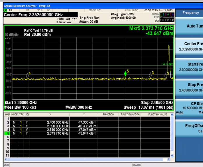
BLE_1M_Ant1_Low_2402
