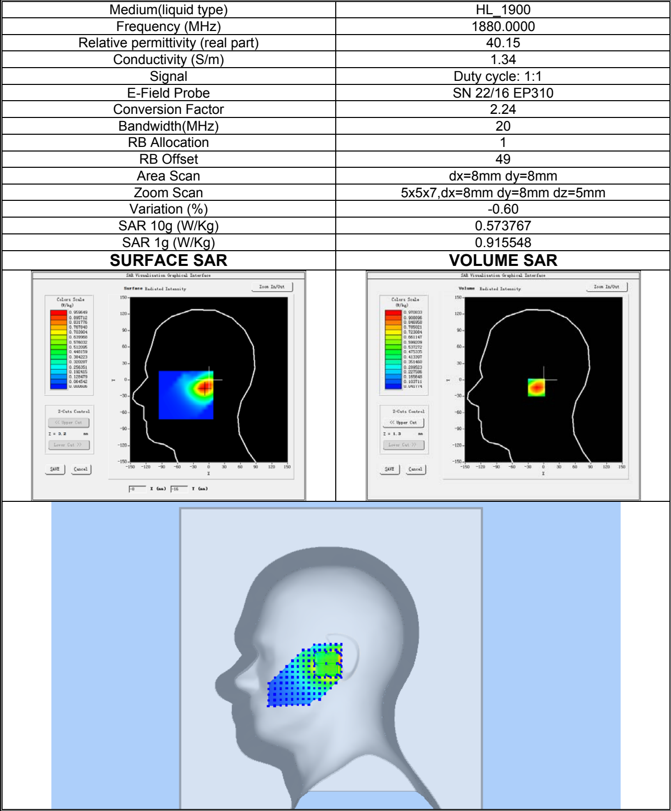
Plot 11:LTE BAND 2, Middle channel (Right Head Cheek) Product Description:Smart Phone Test Date: 2023-04-13
