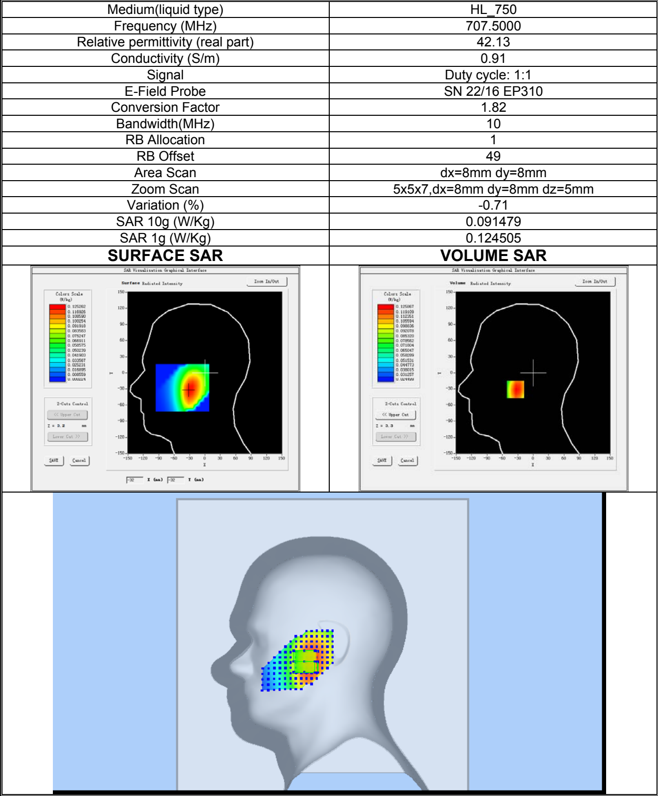
Plot 19:LTE BAND 12, Middle channel (Right Head Cheek) Product Description: Smart Phone Test Date: 2023-04-20
