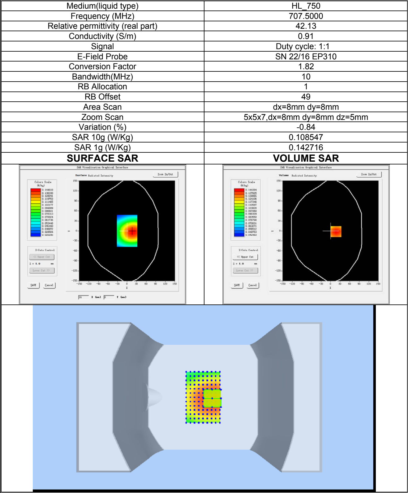
Plot 20: LTE BAND 12, Middle channel (Body-worn/ Hotspot, Back Side) Product Description: Smart Phone Test Date: 2023-04-20
