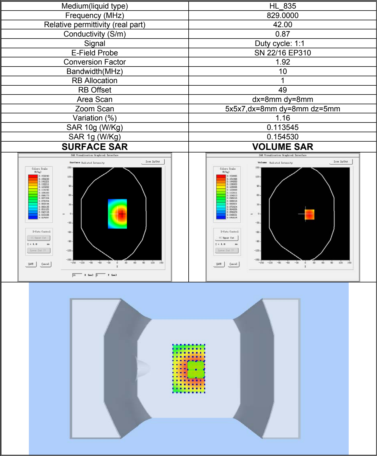
Plot 16: LTE BAND 5, Low channel (Body-worn/ Hotspot, Back Side) Product Description: Smart Phone Test Date: 2023-04-19
