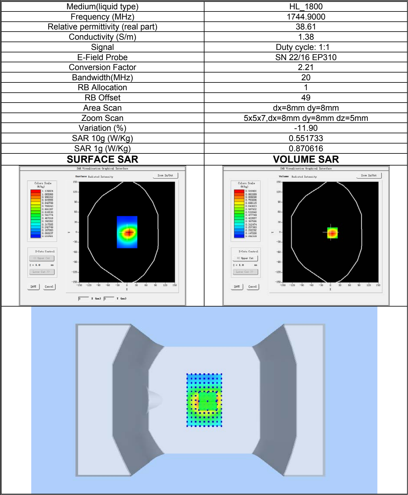
Plot 24: LTE BAND 66, Middle channel (Body-worn/ Hotspot, Back Side) Product Description: Smart Phone Test Date: 2023-04-18
