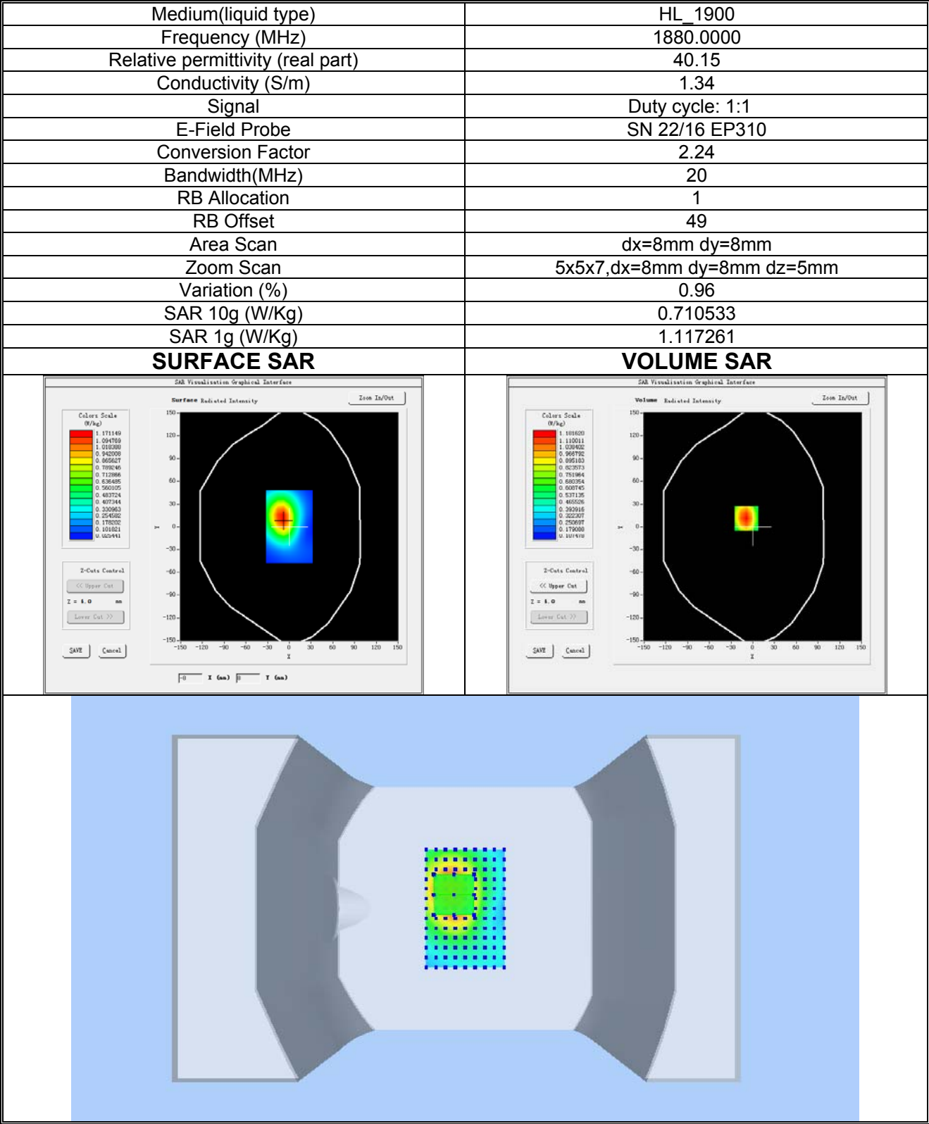
Plot 12:LTE BAND 2, Middle channel (Body-worn /Hotspot, Back Side) Product Description:Smart Phone Test Date: 2023-04-11
