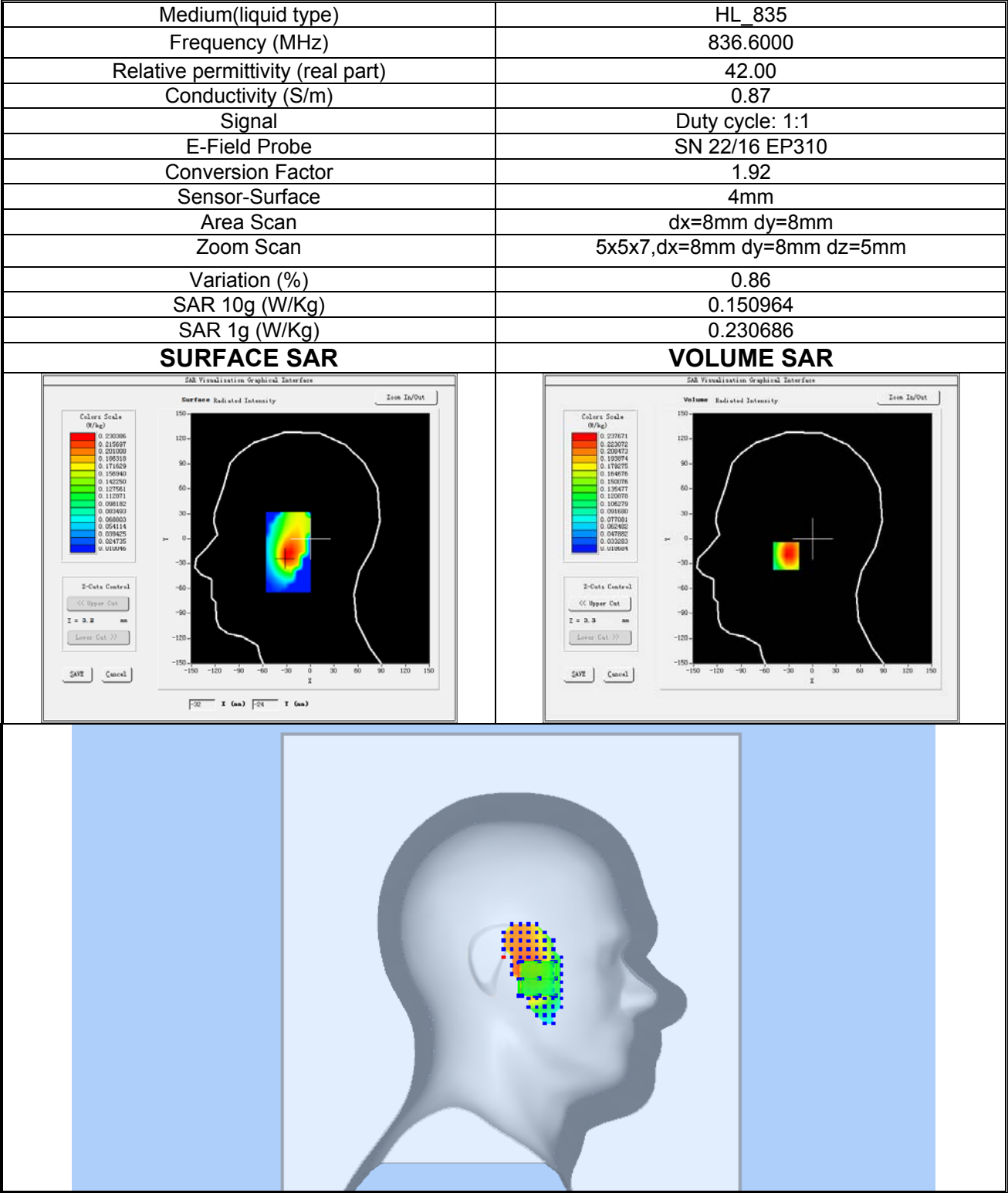
Plot 9: WCDMA BAND V, Middle channel (Left Head Cheek) Product Description: Smart Phone Test Date: 2023-04-18
