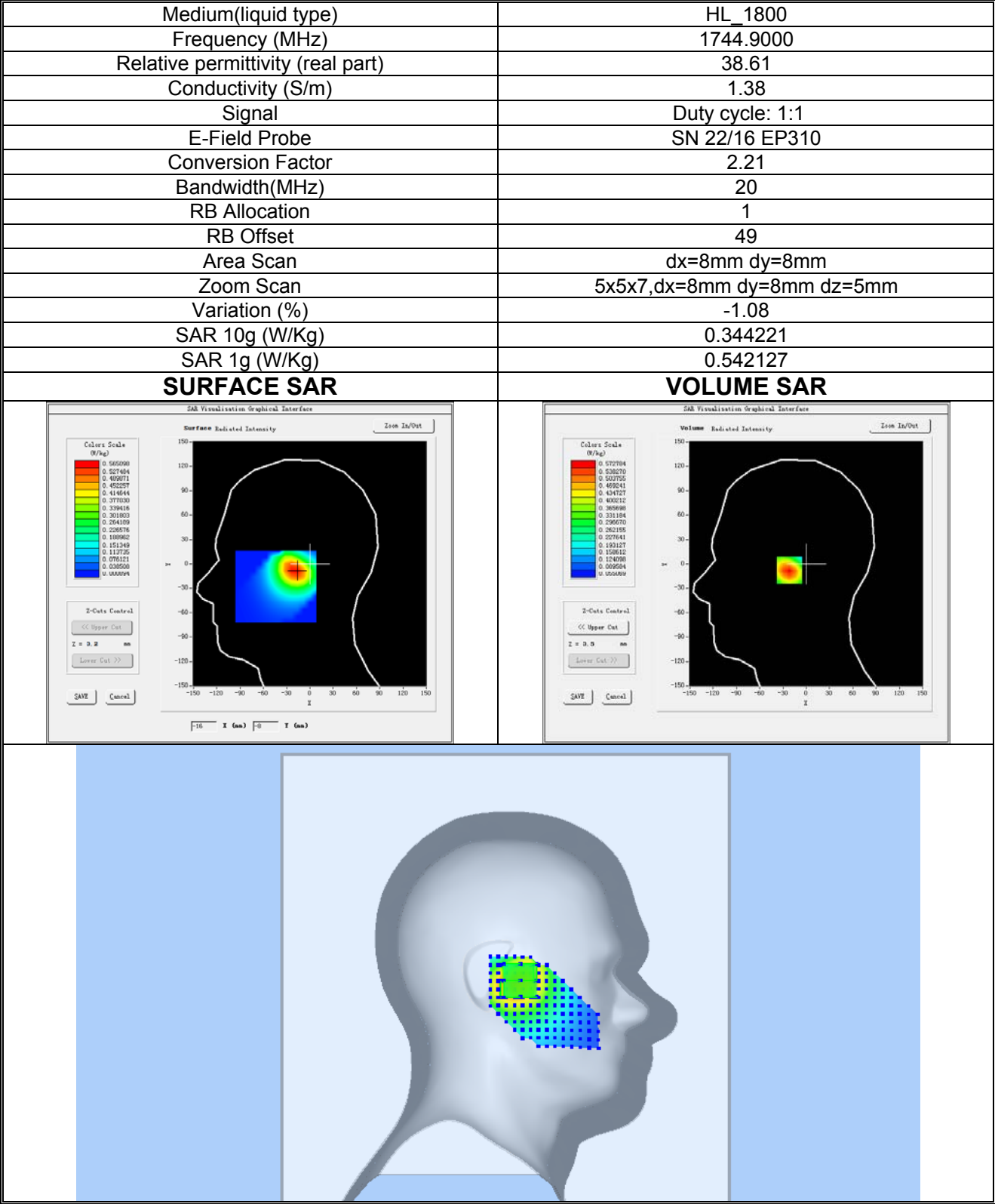
Plot 23:LTE BAND 66, Middle channel (Left Head Cheek) Product Description: Smart Phone Test Date: 2023-04-17
