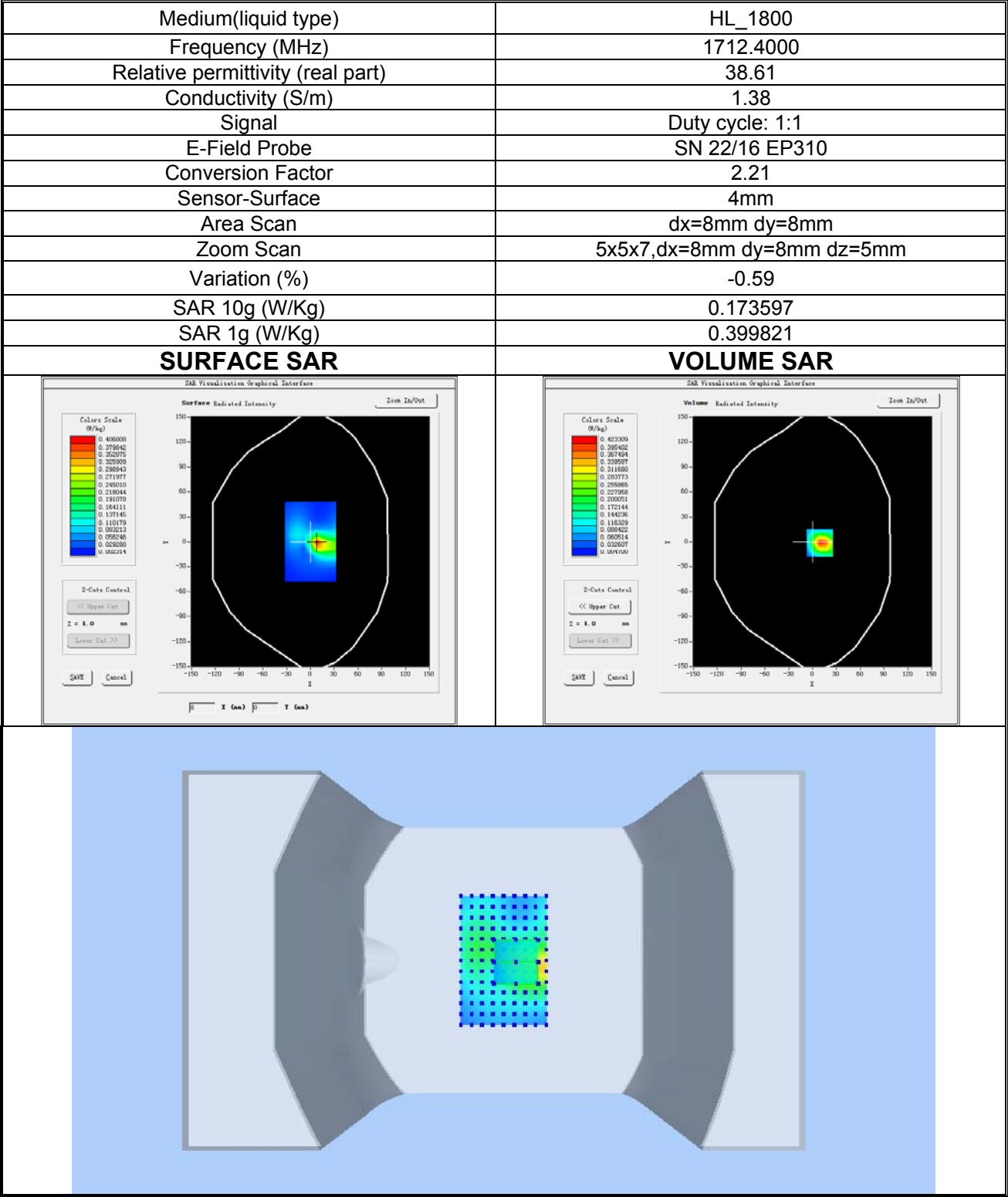
Plot 8: WCDMA BAND IV, Low channel (Body-worn/Hotspot, Back Side) Product Description: Smart Phone Test Date: 2023-04-18
