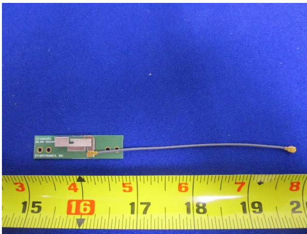
Ethertronics Prestta Antenna Top View
