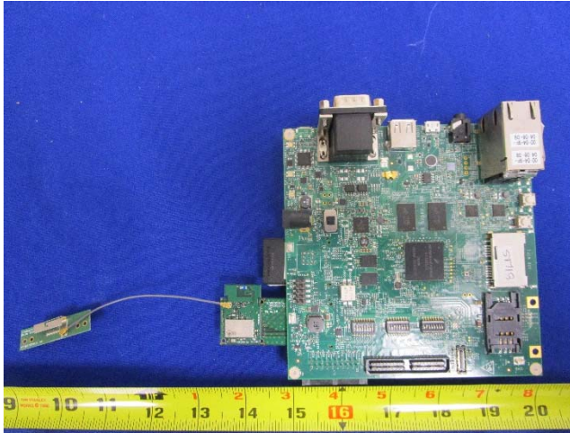
System Board With EUT Top View
