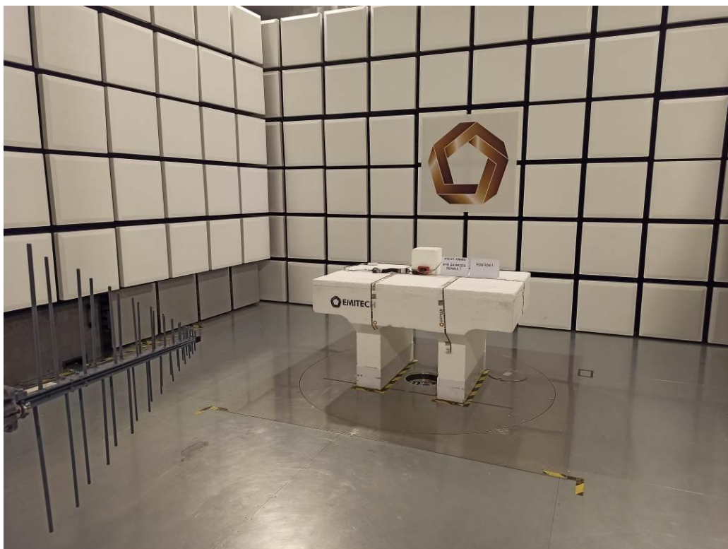
TEST SETUP PHOTO(S) - 200MHZ TO 960MHZ
