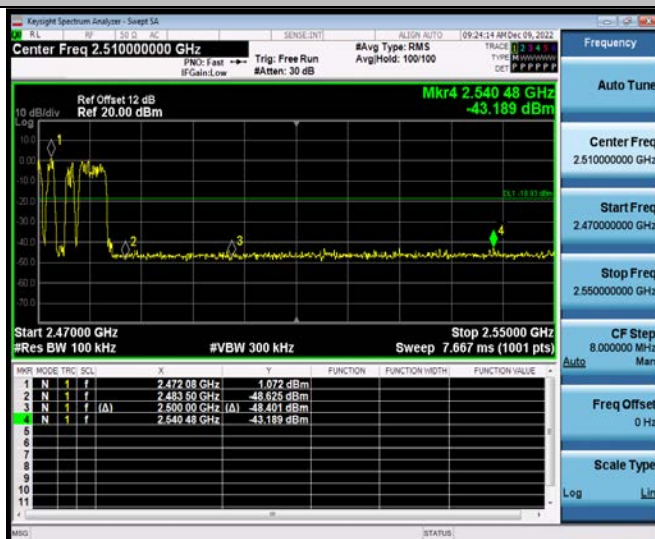
3DH5_Ant1_High_Hop_2480
