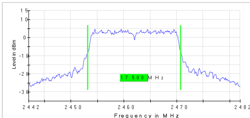
99 % Bandwidth
