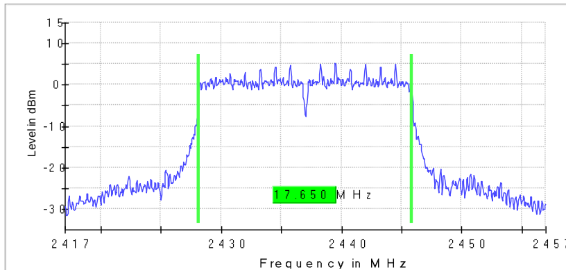
6 dB Bandwidth
