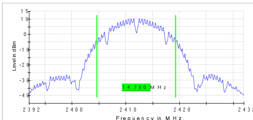
99 % Bandwidth
