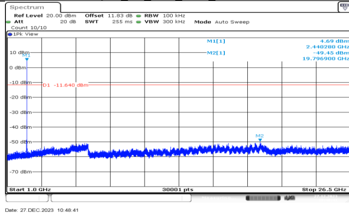
QHS_2M_Ant1_2440_1000~26500
