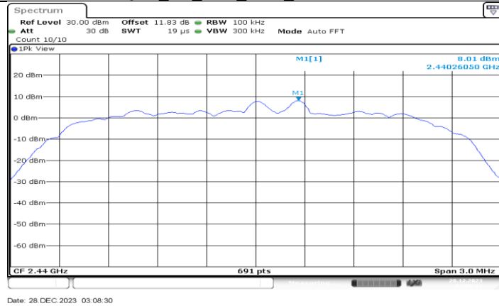
QHS_6M_Ant1_2440_0~Reference
