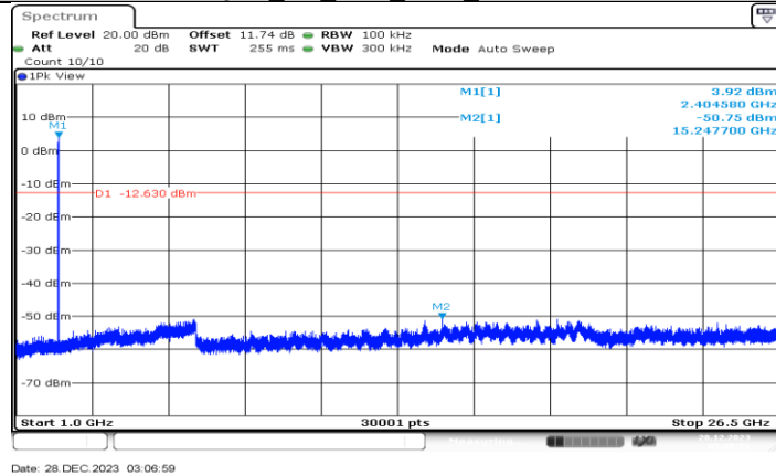
QHS_6M_Ant1_2404_1000~26500
