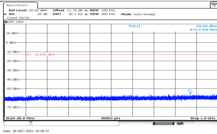
QHS_6M_Ant1_2404_30~1000
