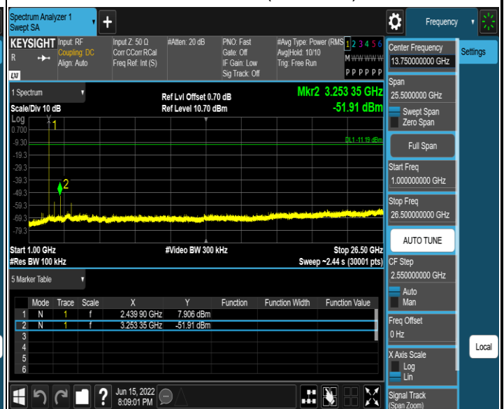
Mode 1 CH19(2440MHz)
