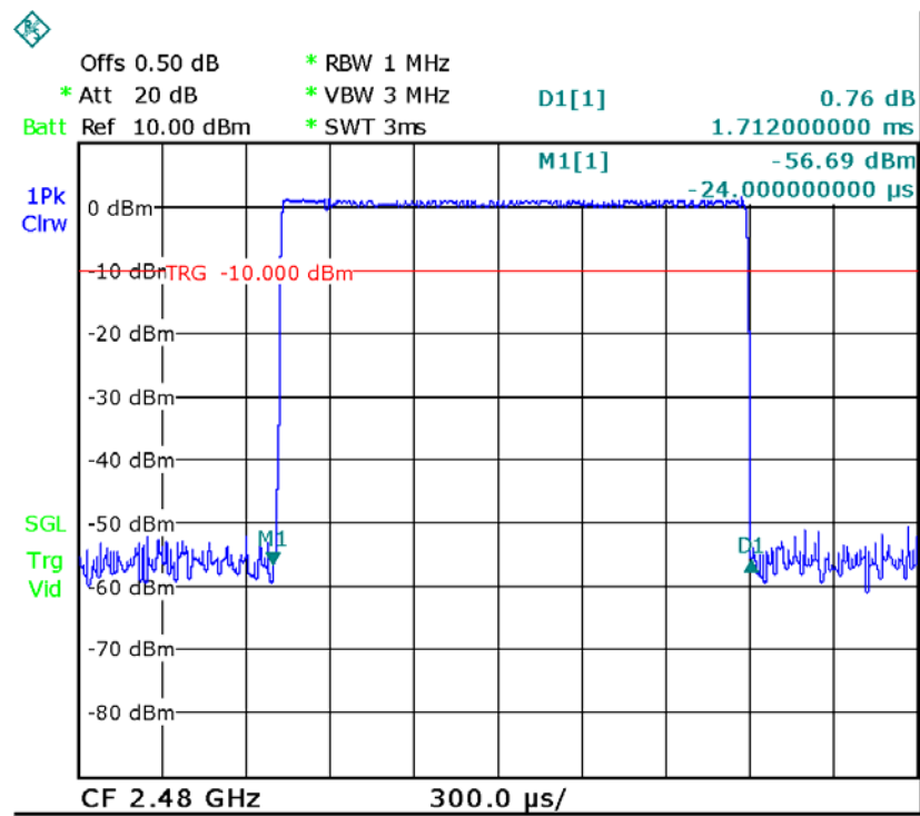
Packet:DH3,High channel
