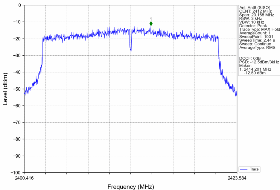
802.11ax(HEW20)_LCH_2412MHz_SU_/_Ant8 (SISO)_NTNV
