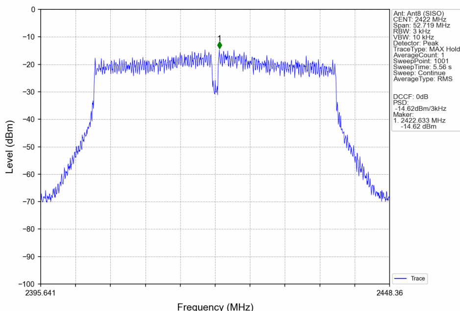
802.11ac(VHT40)_LCH_2422MHz_Ant8 (SISO)_NTNV
