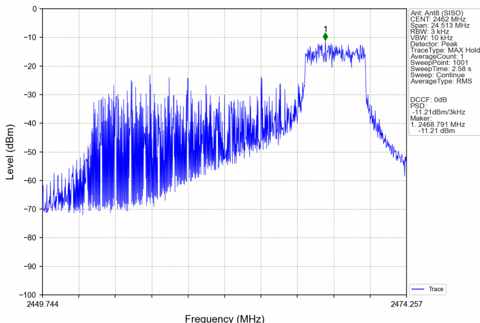
802.11ax(HEW20)_HCH_2462MHz_RU52_Right_Ant8 (SISO)_NTNV
