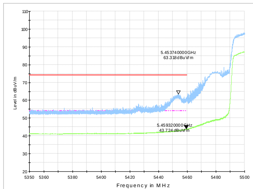
Fig.40 Band Edges (802.11n-HT40 Ch102, 5510MHz)
