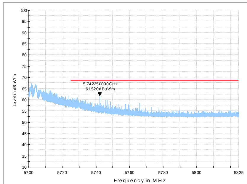
Fig.53 Band Edges (802.11ac-HT80 Ch122, 5610MHz)
