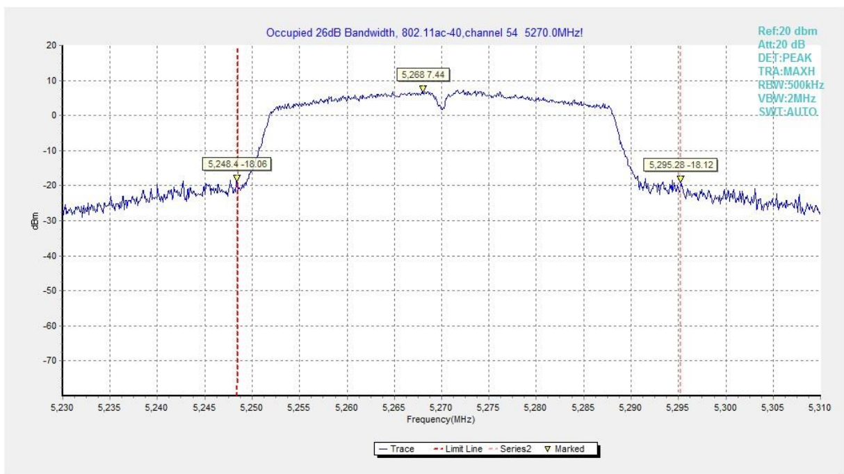
Fig.21 Occupied 26dB Bandwidth (802.11ac-HT40, 5270MHz)
