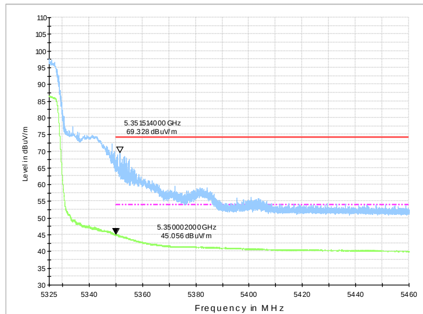
Fig.39 Band Edges (802.11n-HT40 Ch62, 5310MHz)
