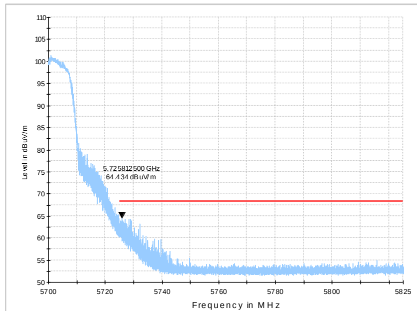
Fig.33 Band Edges (802.11a Ch140, 5700MHz)
