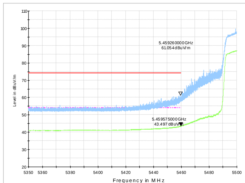
Fig.48 Band Edges (802.11ac-HT40 Ch102, 5510MHz)
