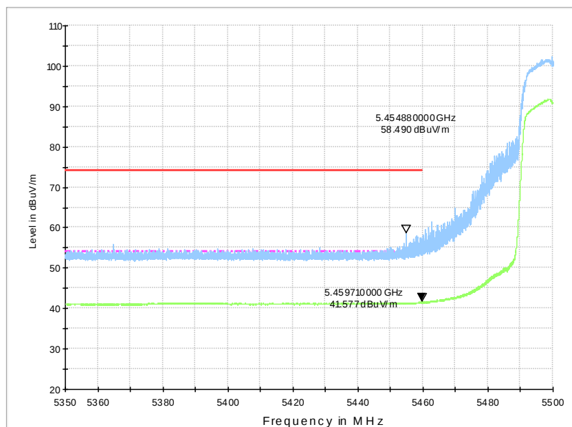
Fig.44 Band Edges (802.11ac-HT20 Ch100, 5500MHz)
