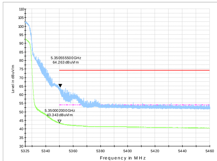
Fig.35 Band Edges (802.11n-HT20 Ch64, 5320MHz)
