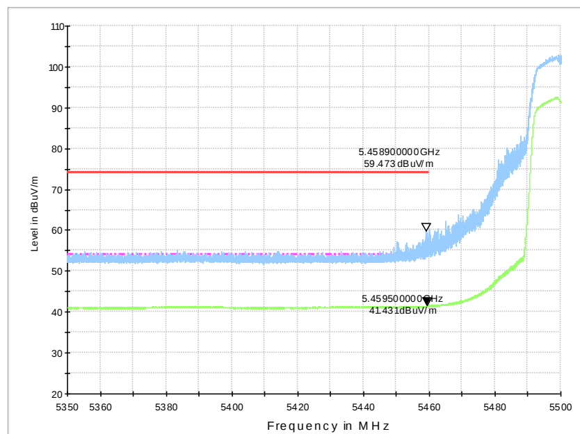
Fig.32 Band Edges (802.11a Ch100, 5500MHz)
