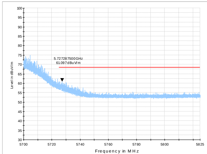
Fig.49 Band Edges (802.11ac-HT40 Ch134, 5670MHz)
