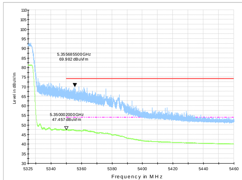
Fig.51 Band Edges (802.11ac-HT80 Ch58, 5290MHz)
