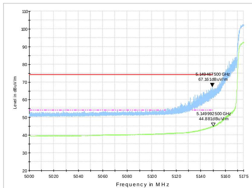
Fig.42 Band Edges (802.11ac-HT20 Ch36, 5180MHz)
