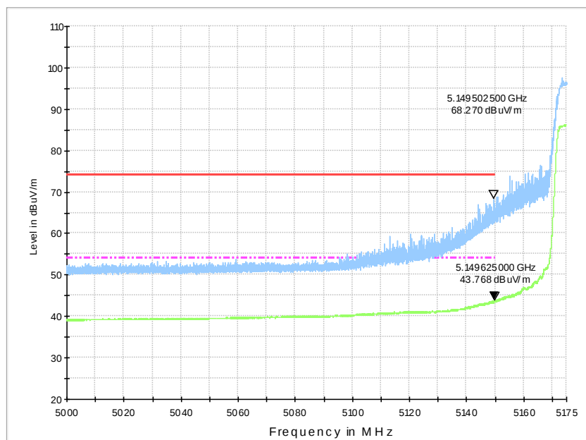
Fig.46 Band Edges (802.11ac-HT40 Ch38, 5190MHz)
