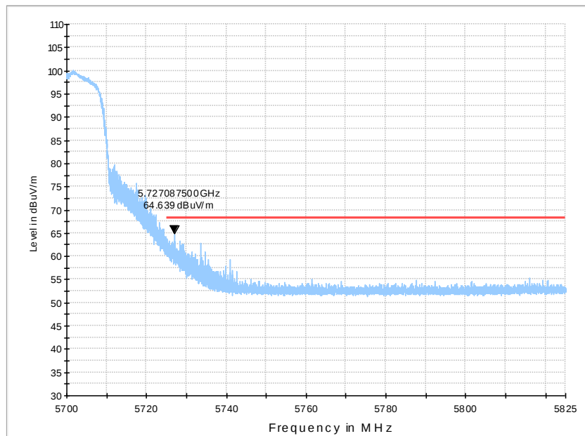
Fig.45 Band Edges (802.11ac-HT20 Ch140, 5700MHz)
