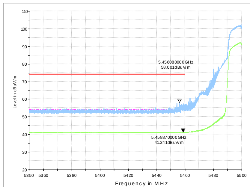
Fig.36 Band Edges (802.11n-HT20 Ch100, 5500MHz)
