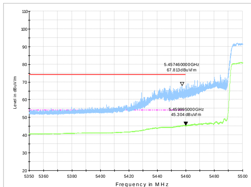
Fig.52 Band Edges (802.11ac-HT80 Ch106, 5530MHz)
