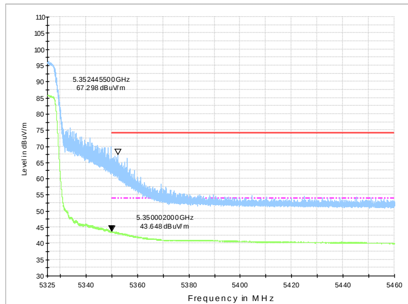
Fig.47 Band Edges (802.11ac-HT40 Ch62, 5310MHz)
