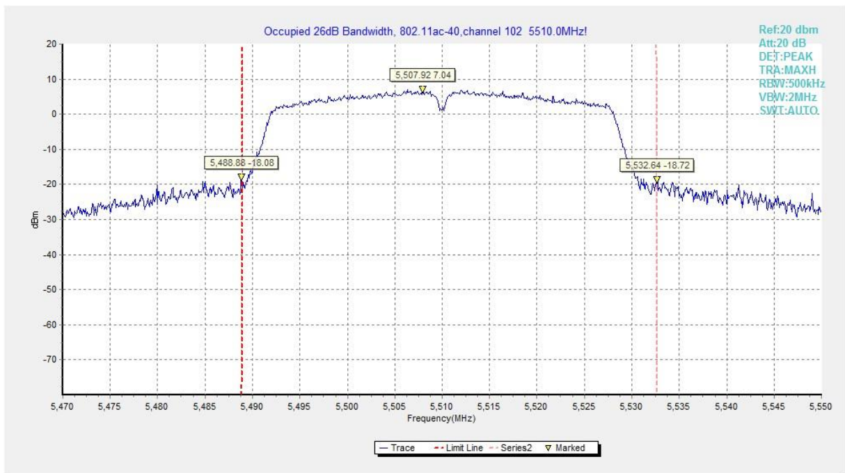
Fig.23 Occupied 26dB Bandwidth (802.11ac-HT40, 5510MHz)
