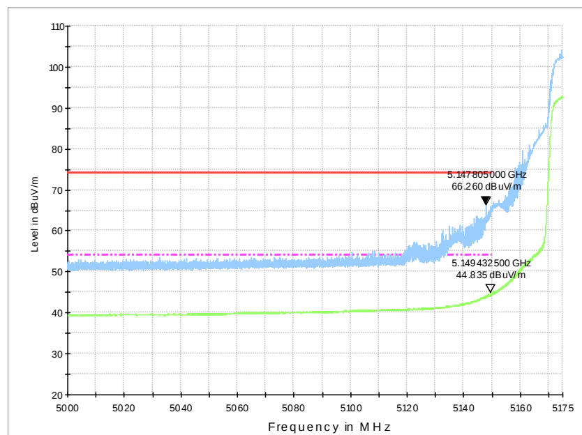
Fig.34 Band Edges (802.11n-HT20 Ch36, 5180MHz)
