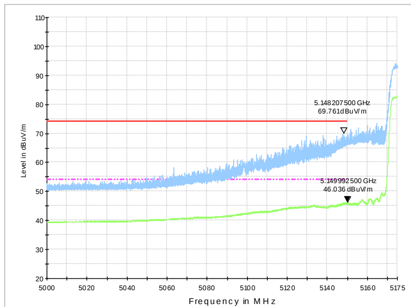
Fig.50 Band Edges (802.11ac-HT80 Ch42 , 5210MHz)
