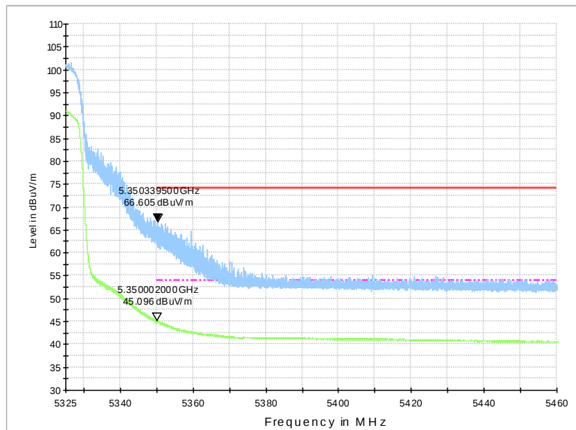
Fig.43 Band Edges (802.11ac-HT20 Ch64, 5320MHz)
