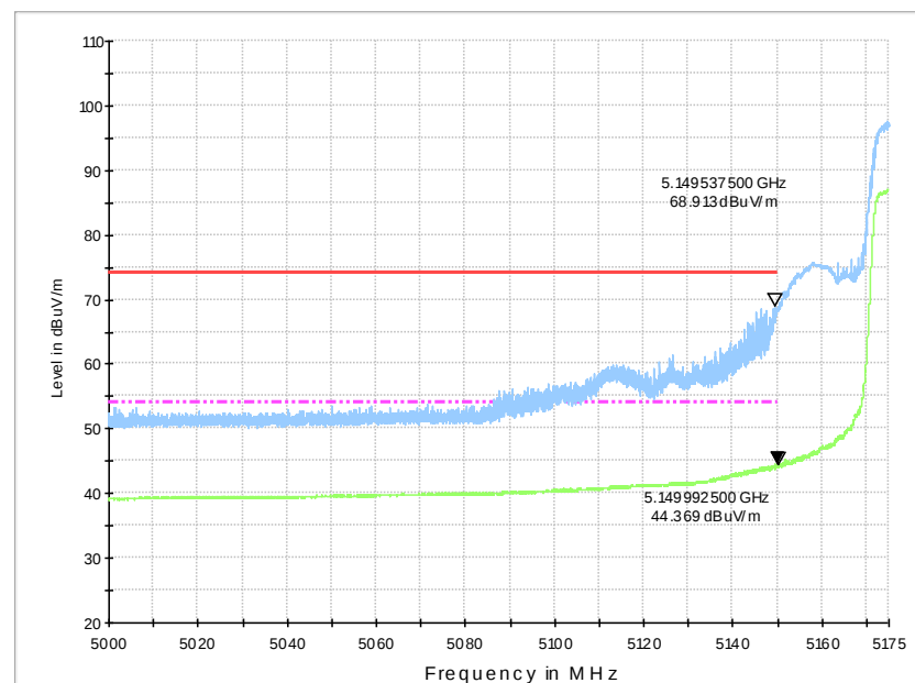
Fig.38 Band Edges (802.11n-HT40 Ch38, 5190MHz)
