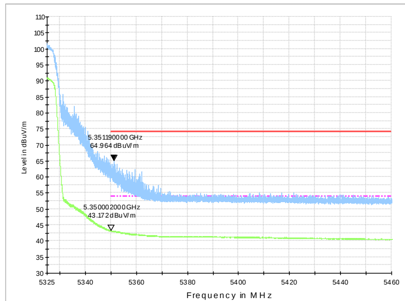
Fig.31 Band Edges (802.11a Ch64, 5320MHz)
