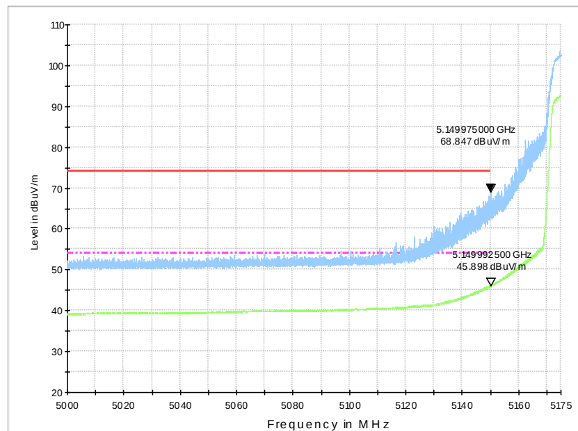
Fig.30 Band Edges (802.11a Ch36, 5180MHz)
