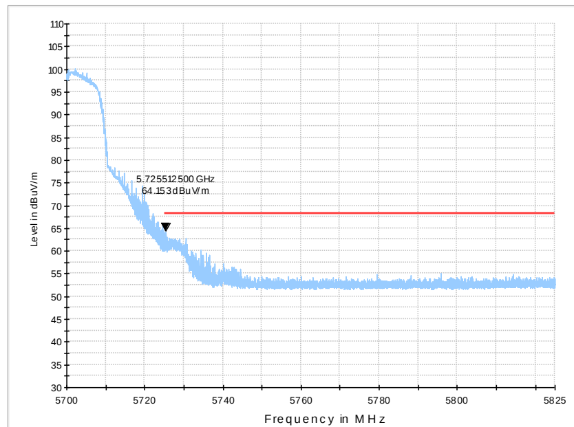
Fig.37 Band Edges (802.11n-HT20 Ch140, 5700MHz)
