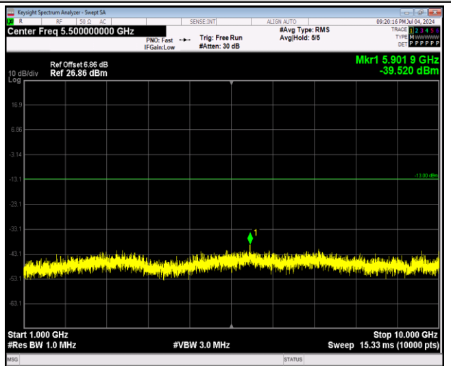
Band26-1.4MHz-16QAM-26697-1RB#0-Range2:1000~10000MHz
