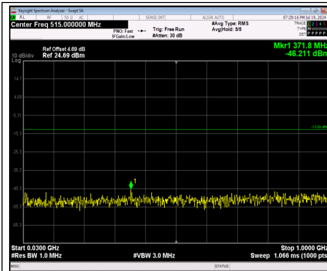
Band25-1.4MHz-64QAM-26683-1RB#0-Range1:30 ~1000MHz
