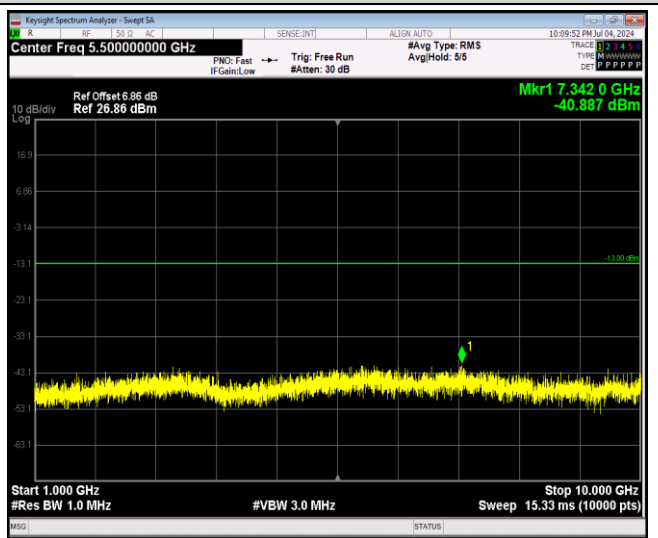
Band26-1.4MHz-16QAM-26697-1RB#0-Range2:1000~10000MHz
