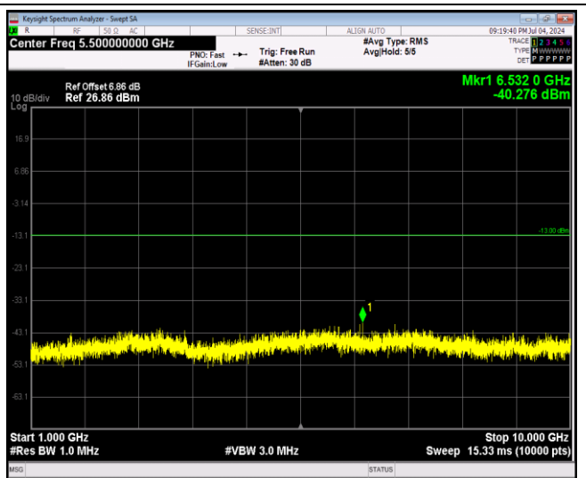
Band26-1.4MHz-QPSK-27033-1RB#0-Range2:1000~10000MHz
