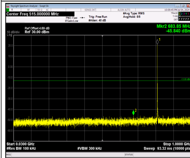
Band26-1.4MHz-16QAM-26697-1RB#0-Range1:30~1000MHz
