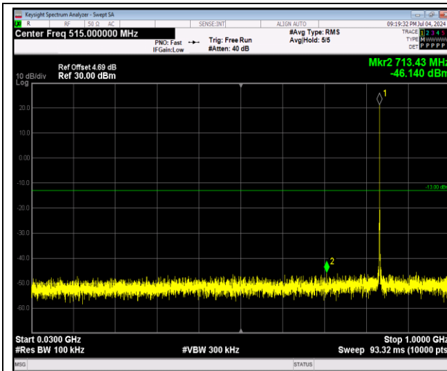
Band26-1.4MHz-QPSK-27033-1RB#0-Range1:30~1000MHz
