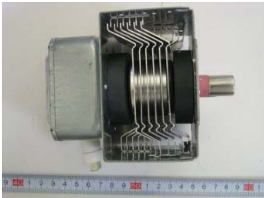
EUT- Magnetism Signal Generator Left View
