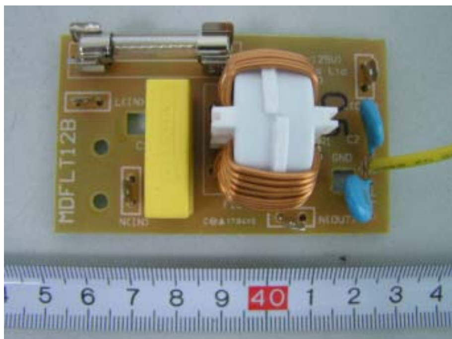
EUT – EMI Filter PCB Top View
