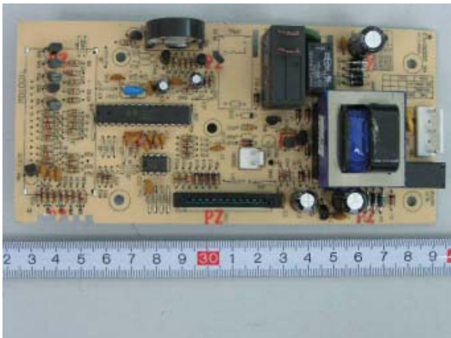
EUT – Control PCB Top View
