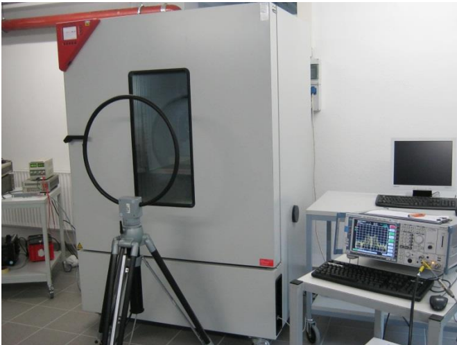
Test setup
