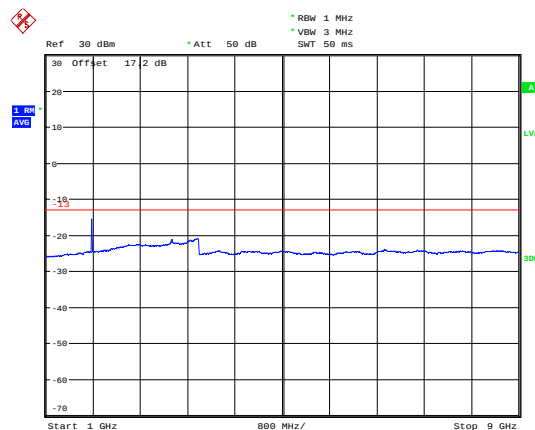
LTE Band 14 5MHz CH-Middle 1GHz~9GHz
