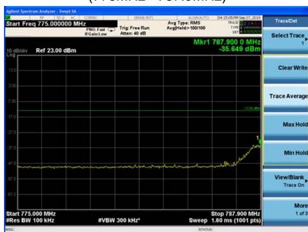
LTE Band 14 16QAM 5MHz CH-LOW 100%RB (775MHz ~787.9MHz)
