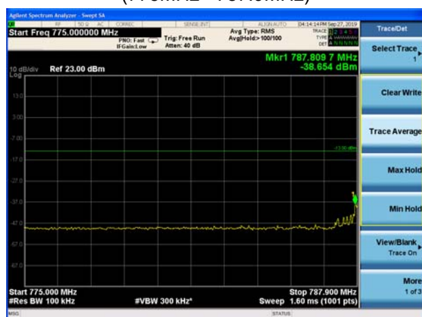
LTE Band 14 QPSK 5MHz CH-LOW 1 RB (775MHz ~787.9MHz)
