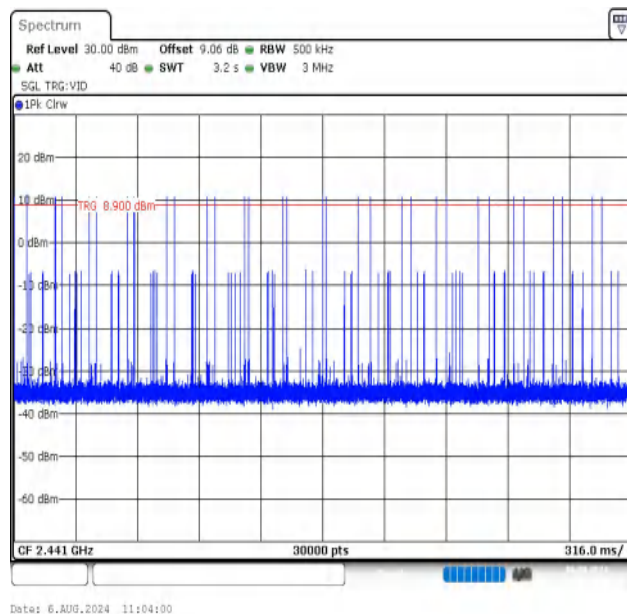
3DH1-Ant1-Hop-PASS
