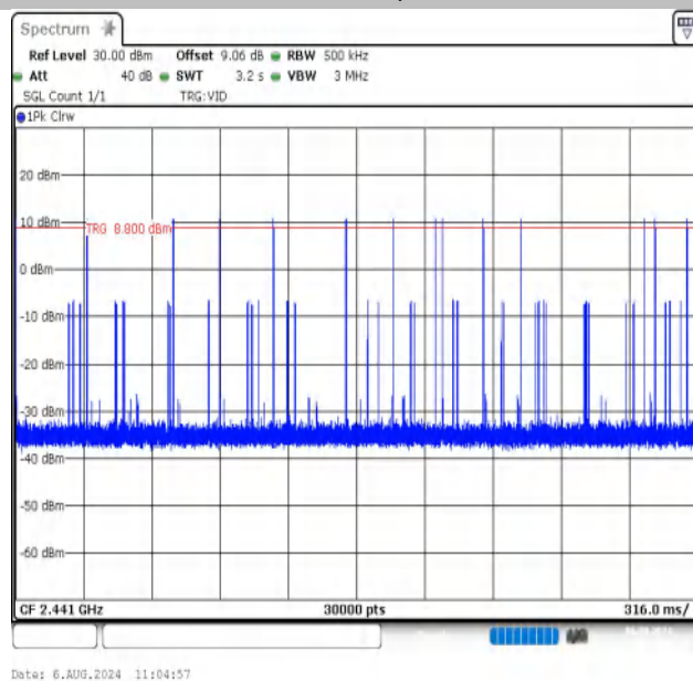
3DH3-Ant1-Hop-PASS
