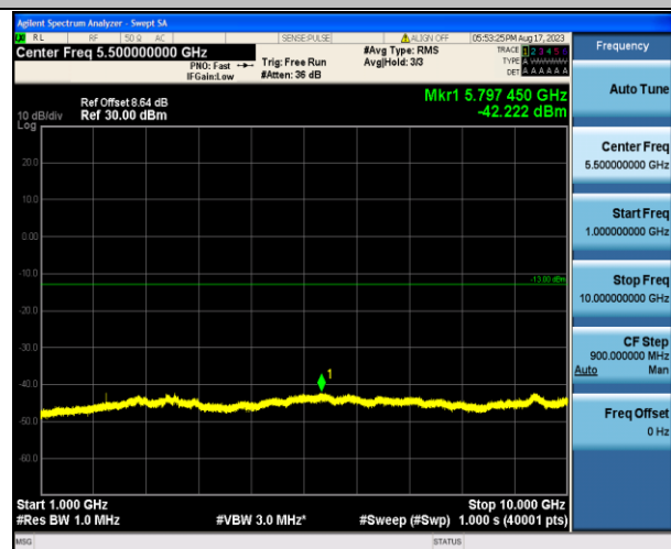
Band12_1.4MHz_QPSK_23095_1RB#0_1000~10000_1000~100
