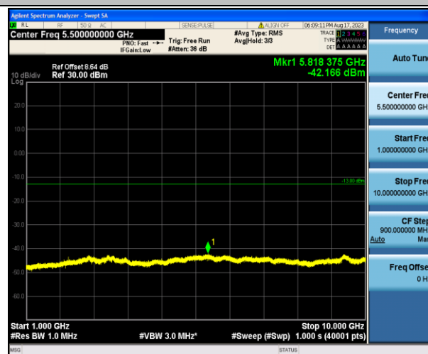
Band12_3MHz_QPSK_23095_1RB#0_1000~10000_1000~10000
