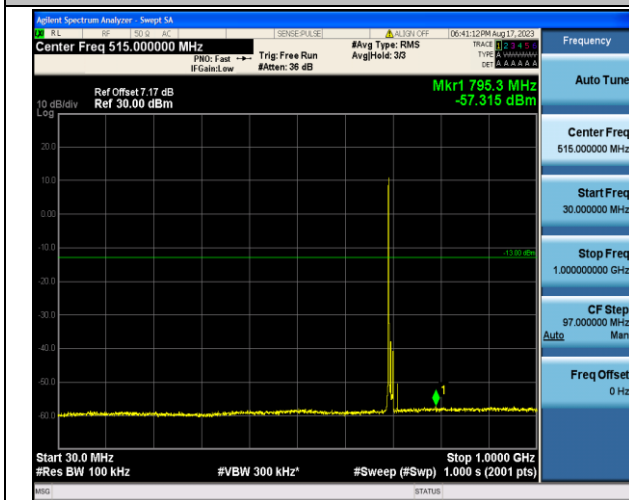
Band12_10MHz_16QAM_23060_1RB#0_30~1000_30~10
