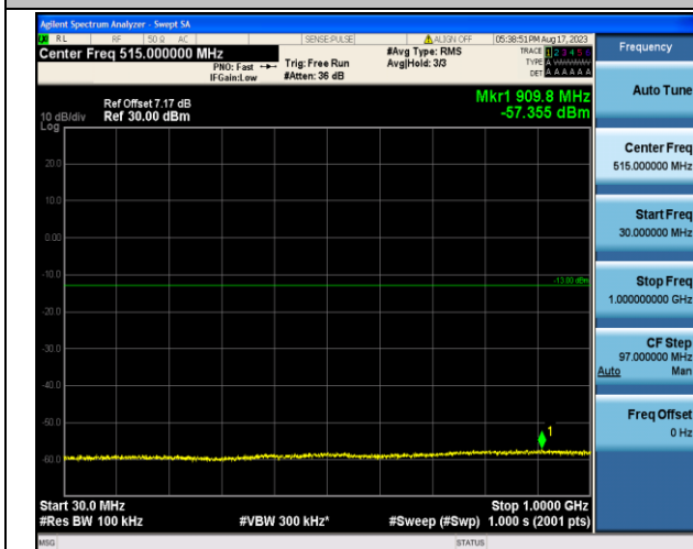
Band4_20MHz_QPSK_20175_1RB#0_30~1000_30~1000
