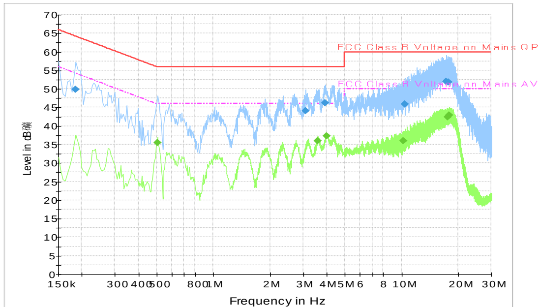
Fig.A.11.1 AC Powerline Conducted Emission- Bluetooth TN-050100U6 (Dong Guan City GangQi Electronic CO.,Ltd.)
