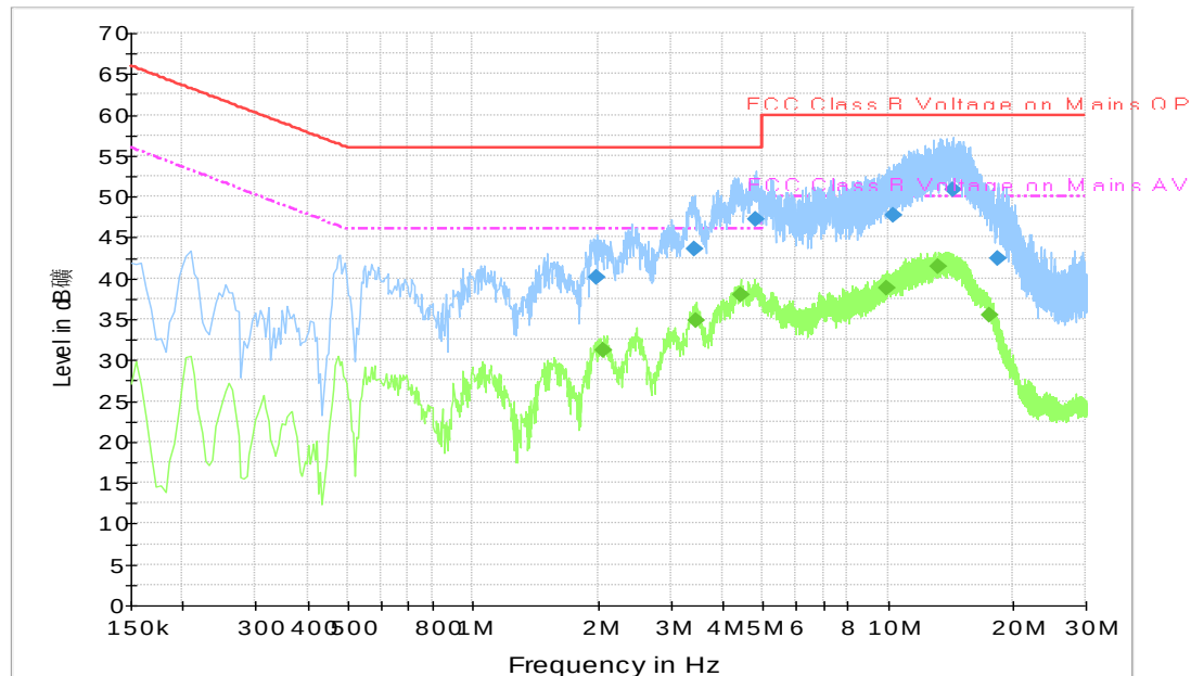
Fig.A.11.3 AC Powerline Conducted Emission- Bluetooth TN-050100U6 (Guangdong Beicom Electronics Co.,Ltd.)
