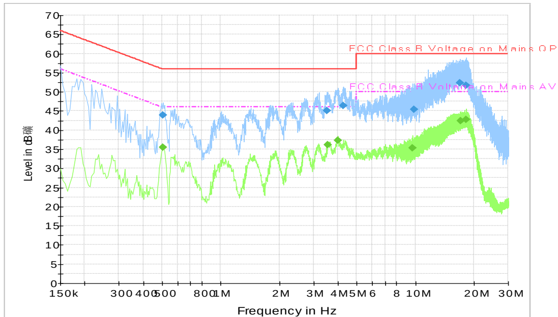
Fig.A.11.2 AC Powerline Conducted Emission-Idle TN-050100U6 (Dong Guan City GangQi Electronic CO.,Ltd.)
