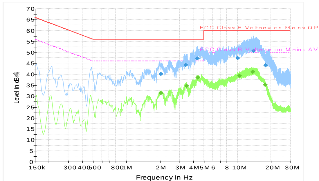
Fig.A.11.4 AC Powerline Conducted Emission-Idle TN-050100U6 (Guangdong Beicom Electronics Co.,Ltd.)
