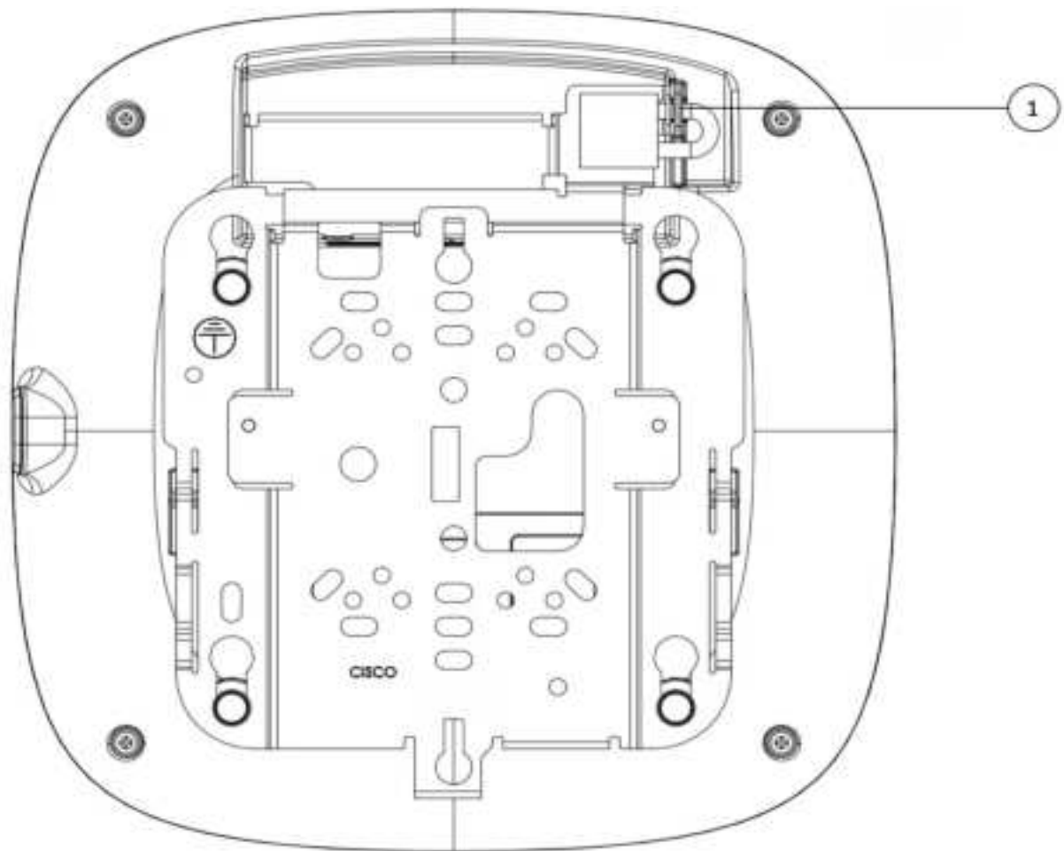
Figure 6 Locking the AP to the Bracket
