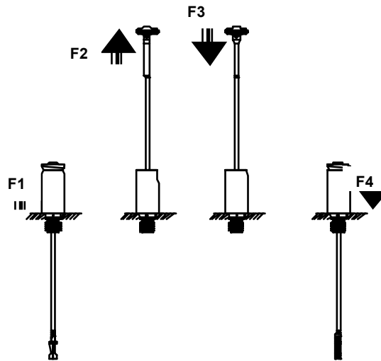
Figure 1. Force Designation for Retraction Forces
