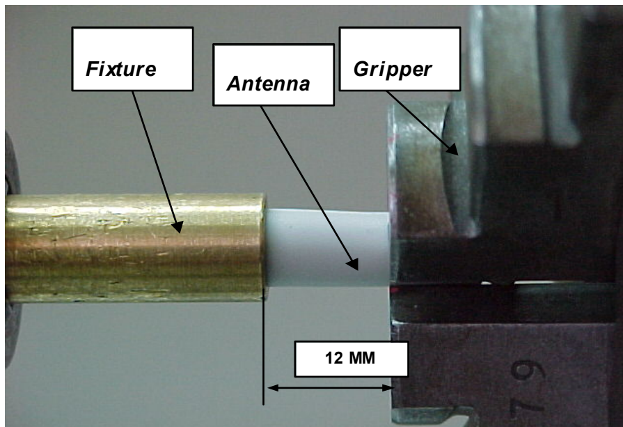
Figure 3. Method for Torque Measurement
