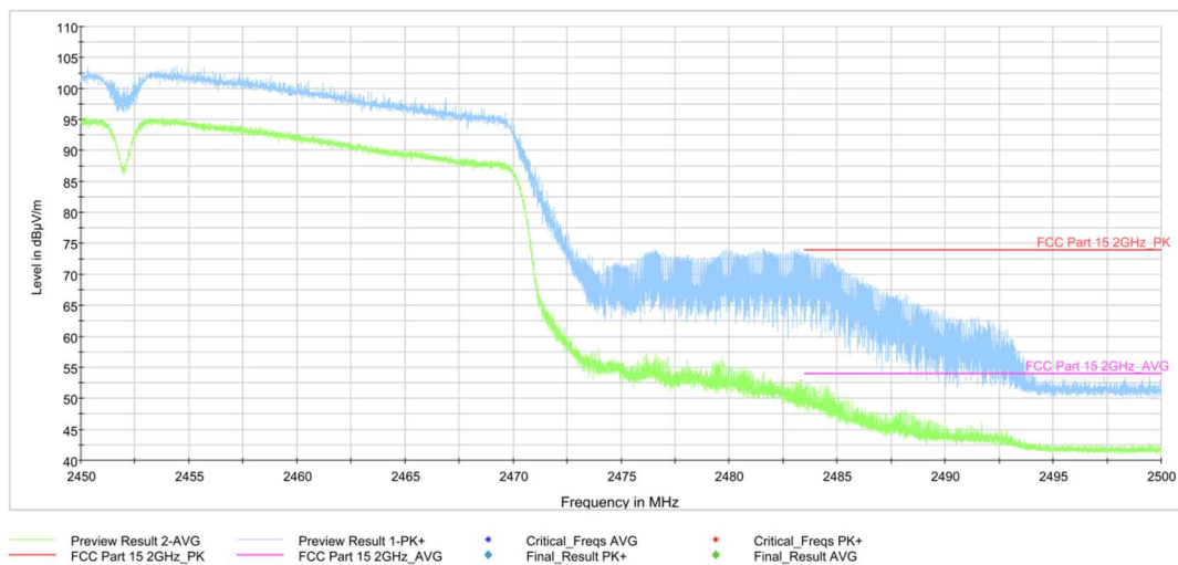
Fig.A.6.2.8 Transmitter Spurious Emission - Radiated (Power): 802.11n-HT40, ch9, 2.45 GHz - 2.50GHz
