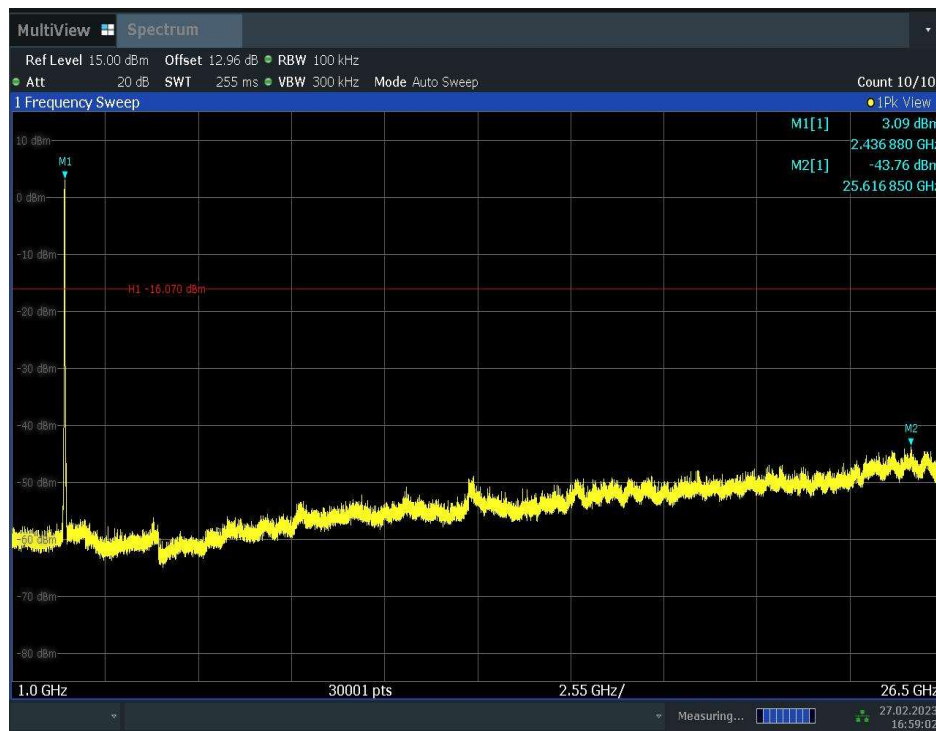
Fig.A.6.1.24 Transmitter Spurious Emission - Conducted (802.11n-HT20, Ch6, 1 GHz-26.5 GHz)
