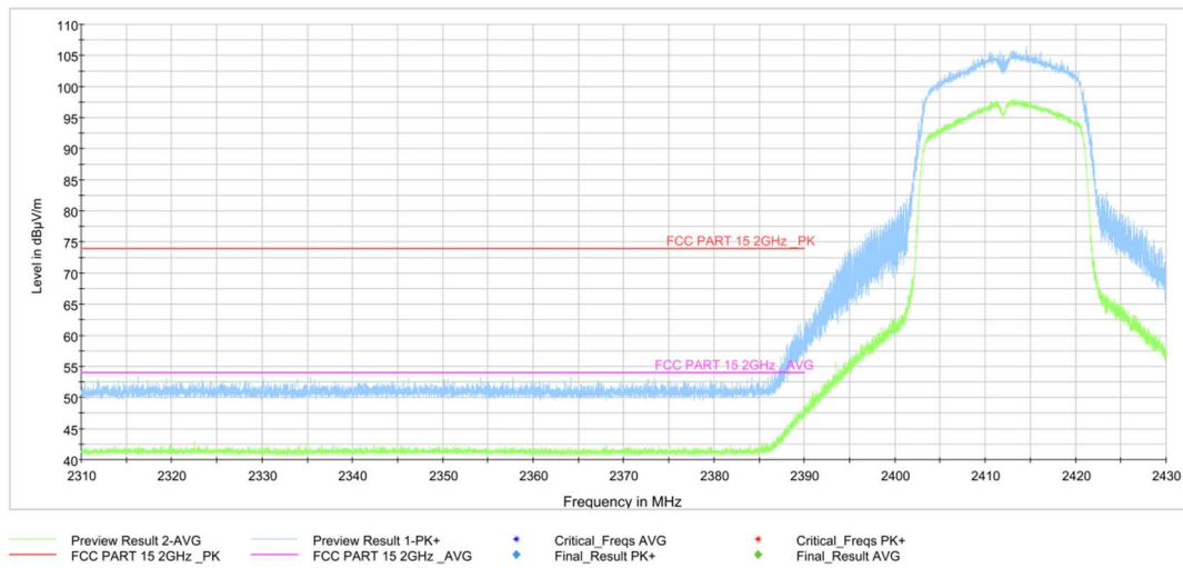
Fig.A.6.2.5 Transmitter Spurious Emission - Radiated (Power): 802.11n-HT20, ch1, 2.31 GHz - 2.43GHz
