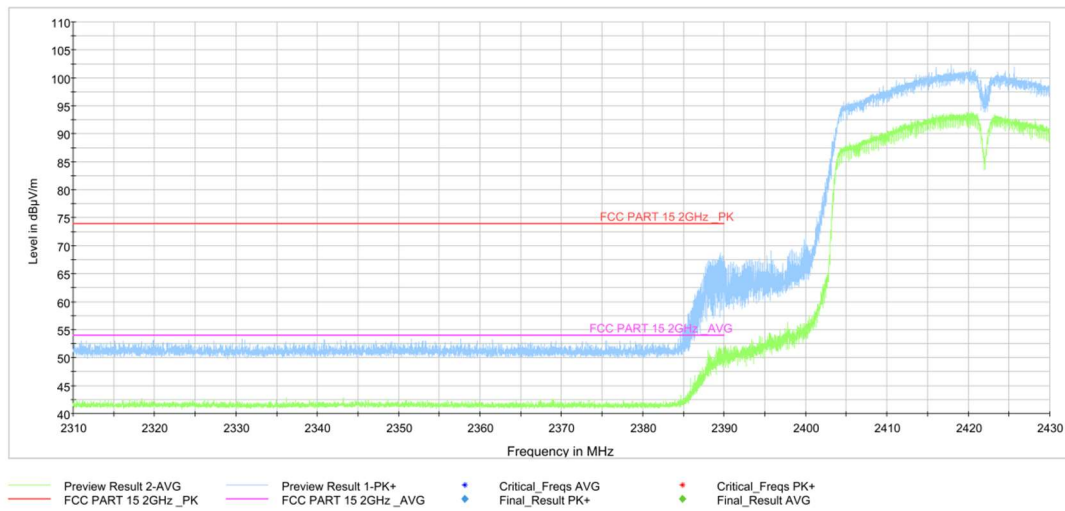
Fig.A.6.2.7 Transmitter Spurious Emission - Radiated (Power): 802.11n-HT40, ch3, 2.31 GHz - 2.43GHz
