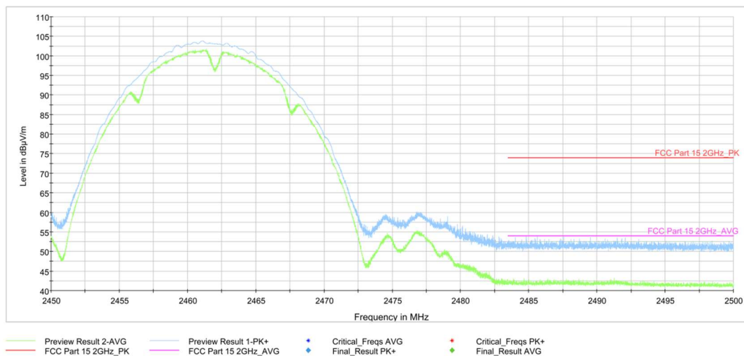
Fig.A.6.2.4 Transmitter Spurious Emission - Radiated (Power): 802.11g, ch11, 2.45 GHz - 2.50GHz
