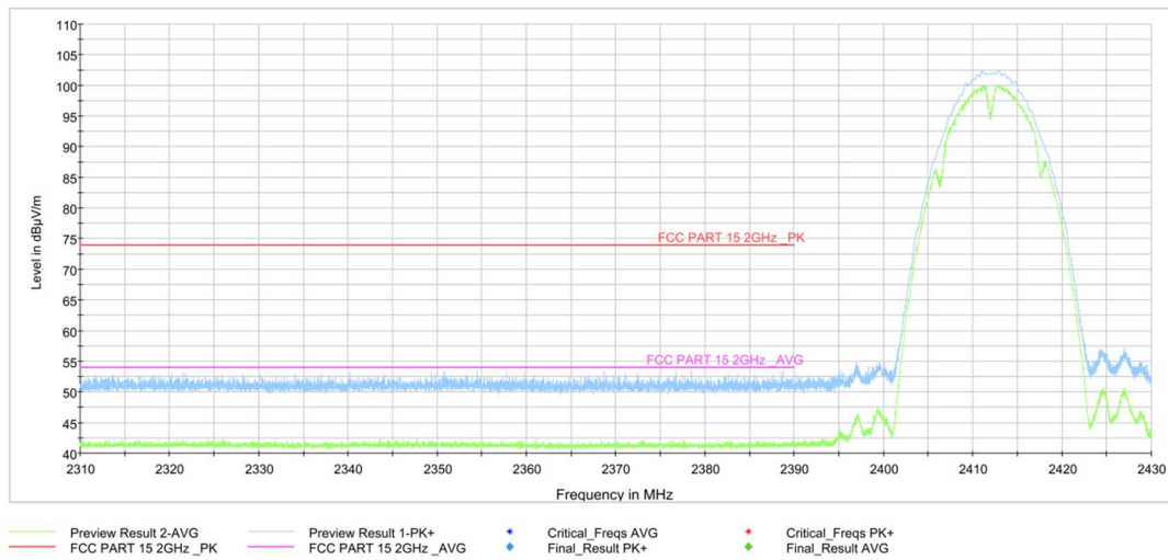
Fig.A.6.2.3 Transmitter Spurious Emission - Radiated (Power): 802.11g, ch1, 2.31 GHz - 2.43GHz
