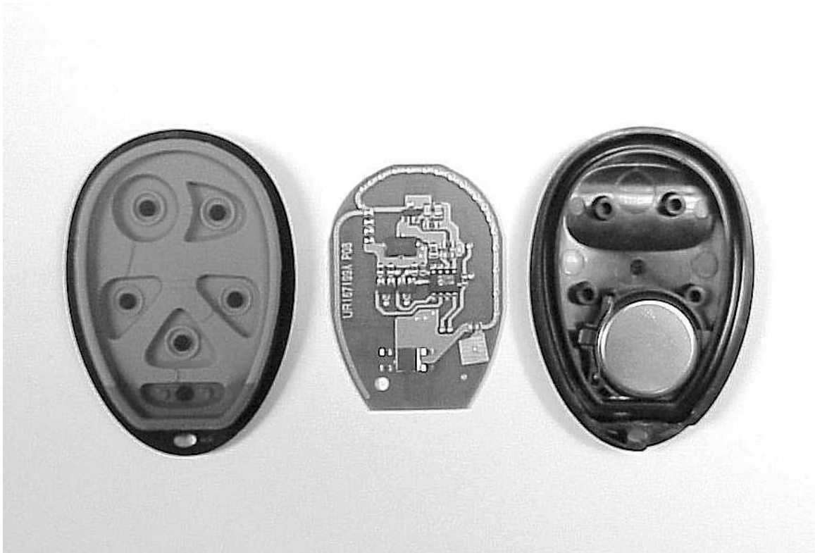
RFA-X FOB Internal View
