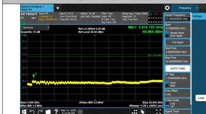
Band2-3MHz-QPSK-19185-1RB#0-3000~20000-PASS
